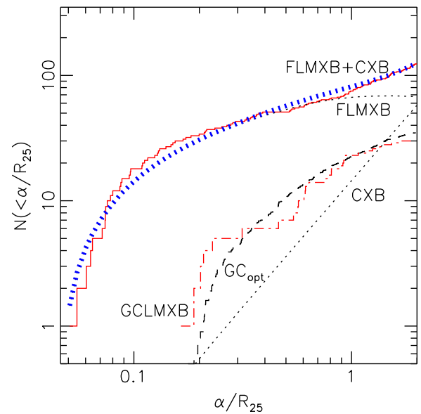
Figure 2. Radial distribution of observed sources excluding GC LMXBs (red solid line), compared to the model (thick blue dotted line) composed of field LMXBs (FLMXB) and CXB sources (thin black dotted line). Also plotted are the radial distributions of GC LMXBs (red dotted-dashed line) and the optical GCs (dashed line, divided by a factor of 10). The cumulation starts at \alpha/R_{25} = 0.046 (i.e., excluding the central a = 10'' elliptical region) and ends at 2D_{25} . To reduce the incompleteness effects, only sources with L_X \geq 4.0 \times 10^{36} erg s ^{-1} are used.
