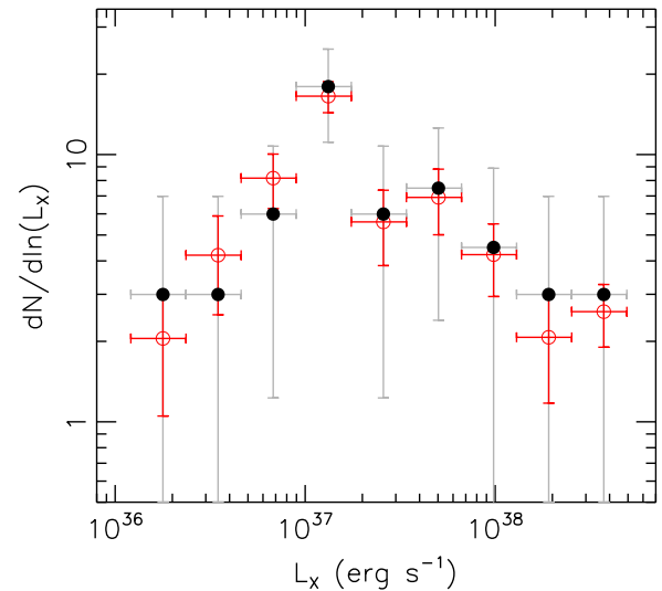
Figure 8. XLF of observed GC LMXBs (filled black circles) and the XLF using the mean of 1,000 simulations (open red circles, with the standard deviation as the error bar). The simulations take into account the possibility that some GCs might host multiple LMXBs (see the text). The XLFs were not corrected for the incompleteness effects.
