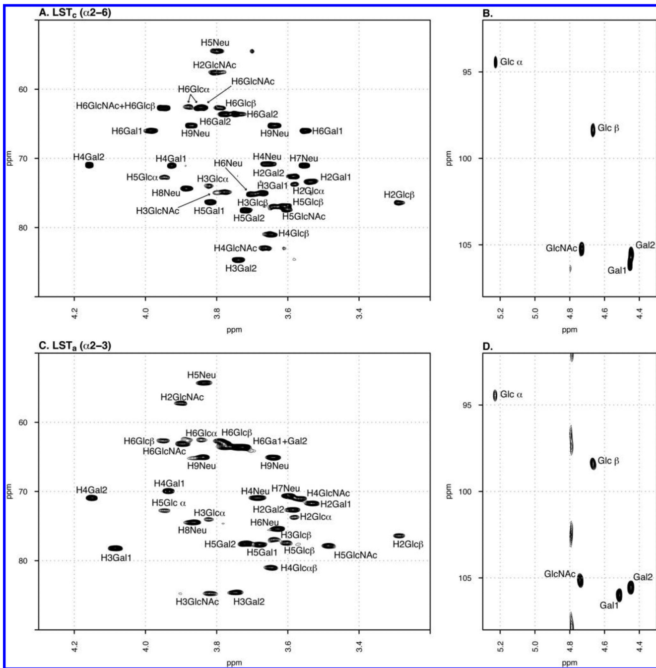
Figure 1. 1 H- 13 C HSQC NMR spectra of LSTc (A and B) and LSTa (C and D).
