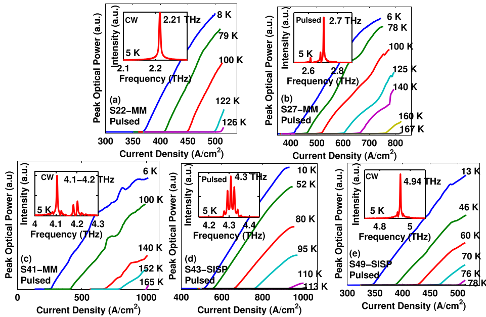
FIG. 3. Pulsed light-current measurements and lasing spectra (both pulsed and CW at \sim 5 K, insets) of the samples listed in Table I. (a) Sample S22-MM, (b) sample S27-MM, (c) sample S41-MM, (d) sample S43-SISP, and (e) sample S49-SISP.
