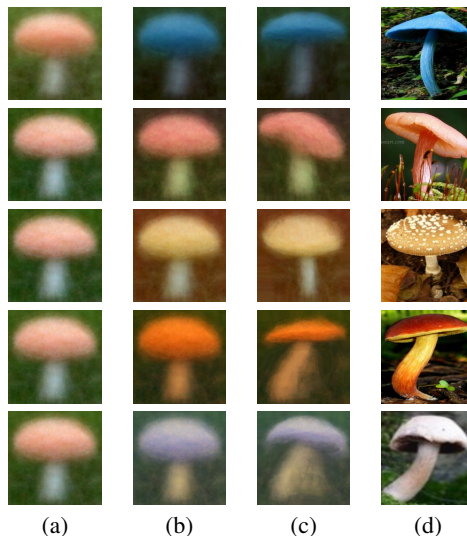
Figure 3. Evolution of mushrooms from \mathbf{g} to \mathbf{f} . (a): \mathbf{g}_k(\mathbf{x}) , (b): \mathbf{A}_k \mathbf{g}_k(\mathbf{x}) + \mathbf{b}_k , (c): \mathbf{A}_k \mathbf{g}_k(\mathbf{u}_k(\mathbf{x})) + \mathbf{b}_k , (d): \mathbf{f}_k(\mathbf{x})
