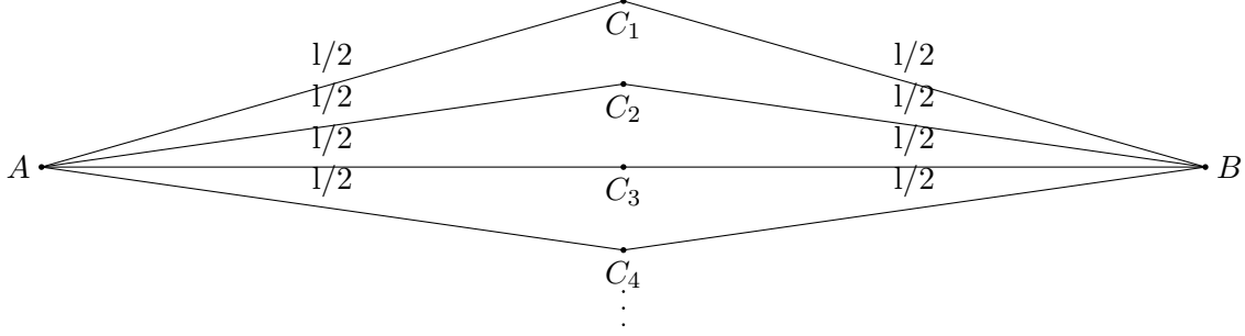
Figure 2: Splitting Operation
