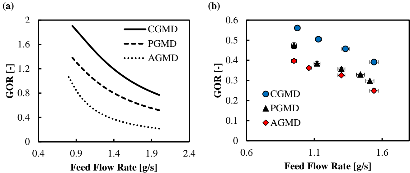
Figure 5. (a) Numerical model predictions on GOR as a function of feed flow rate. (b) Experimental GOR as a function of flow rate, d_{gap} = 1.24 mm
