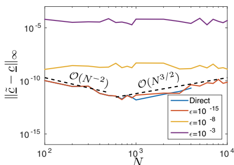
FIG. 8. The maximum absolute error \|\tilde{c} - c\|_\infty , where c and \tilde{c} satisfy (6.4). Here, the DHT was computed with direct summation and our algorithm with \epsilon = 10^{-3}, 10^{-8}, 10^{-15} . As N \rightarrow \infty the DHT is its own inverse, up to a diagonal scaling. For N < 700 the error \|\tilde{c} - c\|_\infty decays like \mathcal{O}(N^{-2}) because (6.3) only holds asymptotically as N \rightarrow \infty . For N > 700 the error \|\tilde{c} - c\|_\infty grows like \mathcal{O}(N^{3/2}) from numerical error accumulation.
