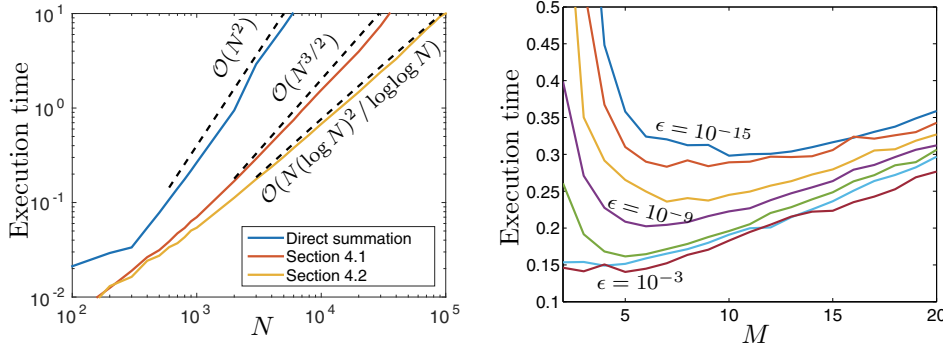
FIG. 5. Left: Execution time for computing (4.2) with \mathcal{O}(N^2) direct summation, the \mathcal{O}(N^{3/2}) algorithm (see section 4.1), and the \mathcal{O}(N(\log N)^2/\log \log N) algorithm (see section 4.2). Right: Computational timings for N = 5,000 with 2 \leq M \leq 20 and \epsilon = 10^{-15}, 10^{-11}, \dots, 10^{-3} . Numerical experiments like these motivate the choice M = \max(\lceil 0.3 \log(1/\epsilon) \rceil, 3) in (4.5).
