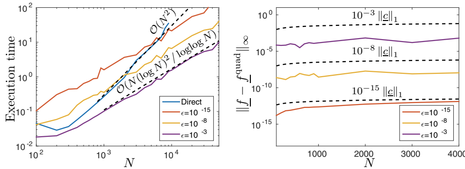
FIG. 7. Left: Execution time for computing the DHT in (6.1) using direct summation and our \mathcal{O}(N(\log N)^2/\log\log N) algorithm with \epsilon = 10^{-15}, 10^{-8}, 10^{-3} . Right: The maximum absolute error in the computed vector \underline{f} . Here, we compare the computed error (solid lines) with the expected error bound \mathcal{O}(\epsilon\|\underline{c}\|_1) .
