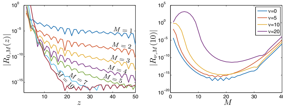
FIG. 1. Left: The absolute value of R_{0,M}(z) in (3.1) on z \in (0, 50] for M = 1, 2, 3, 4, 5, 7, 10 . For any M \geq 1 and sufficiently large z , the asymptotic expansion is an accurate approximation. Right: The absolute value of R_{\nu,M}(10) for 1 \leq M \leq 40 and \nu = 0, 5, 10, 20 . For a fixed z , increasing M may reduce the accuracy of the asymptotic expansion and will eventually lead to numerical overflow issues.
