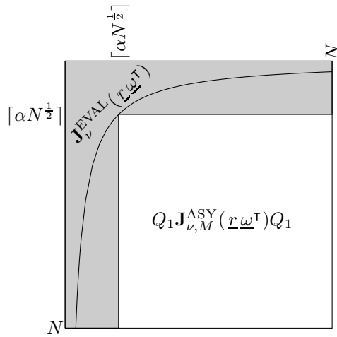
FIG. 3. A partition of the entries of \mathbf{J}_\nu(\underline{r}\underline{\omega}^\top) that motivates the matrix decomposition (4.8). The asymptotic expansion (3.1) is used for the (k, n) entry if it satisfies \min(k, n) \geq \lceil \alpha N^{1/2} \rceil . The gray region shows the nonzero entries of \mathbf{J}_\nu^{\text{EVAL}}(\underline{r}\underline{\omega}^\top) that are not dealt with by the asymptotic expansion. The black curve indicates the entries satisfying |R_{\nu, M}(r_k \omega_n)| = \epsilon . A numerically stable \mathcal{O}(N^{3/2}) algorithm for evaluating Schlömilch expansions follows.
