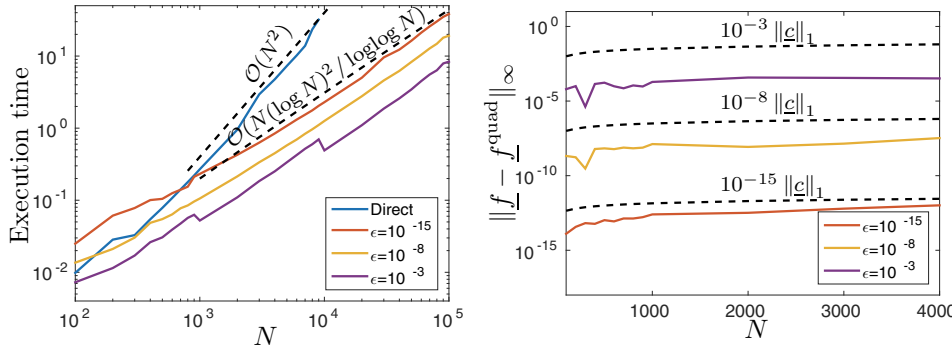
FIG. 6. Left: Execution time for evaluating (5.1) at 1/N, \dots, N/N with \mathcal{O}(N^2) direct summation and the \mathcal{O}(N(\log N)^2/\log \log N) algorithm described in this section. For a relaxed working accuracy our algorithm becomes even more computationally advantageous over direct summation. Right: Maximum absolute error in the computed vector \underline{f} . Here, we compare the observed error (solid lines) with the expected bound of \mathcal{O}(\epsilon\|\underline{c}\|_1) (dotted lines).
