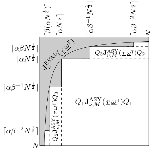
FIG. 4. A partition of the entries of \mathbf{J}_\nu(\underline{r}\underline{\omega}^\top) that motivates the matrix decomposition (4.9). The gray region shows the nonzero entries of \mathbf{J}_\nu^{\text{EVAL}}(\underline{r}\underline{\omega}^\top) that are not dealt with by the asymptotic expansion. The black curve indicates the entries satisfying |R_{\nu,M}(r_k\omega_n)| = \epsilon . The asymptotically near-optimal choice of the parameter \beta is \mathcal{O}(1/\log N) and the number of partitions should grow like \mathcal{O}(\log N/\log\log N) with N . A numerically stable \mathcal{O}(N(\log N)^2/\log\log N) algorithm for evaluating Schlömilch expansions follows.
