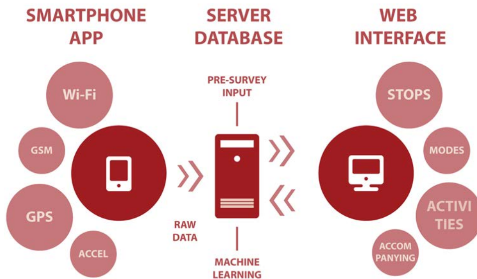
Figure 2: Survey architecture
