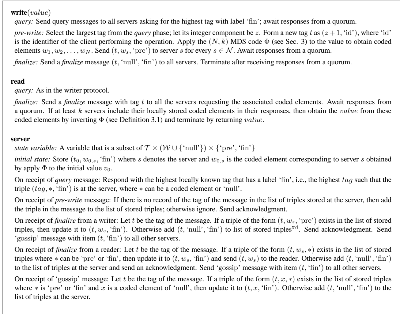
Figure 1: Write, read, and server protocols of the CAS algorithm.
