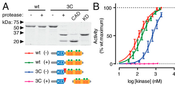
Fig. 1. TgCDPK1 is not activated by removal of its regulatory domain. (A) Introduction of a 3C protease cleavage site between the CAD and KD of TgCDPK1 , in the kinase referred to as 3C, enables separation of the two domains upon protease treatment. The wild-type (WT) enzyme was unaffected by the protease treatment. The CAD and KD could be further isolated from the digested 3C. (B) Kinase activity of WT and 3C, before (-) and after (+) protease treatment. Mean \pm SEM, n = 3 independent experiments.
