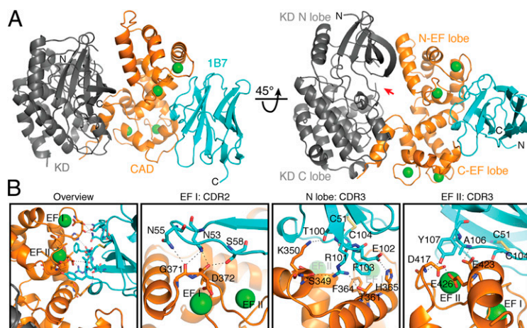
Fig. 4. 1B7 stabilizes a novel conformation of TgCDPK1 . (A) Cartoon depicting the structure of the complex with the catalytic KD (gray), the CaM-like CAD (orange), bound calcium ions (green spheres), and 1B7 (blue). The position of the active site pocket is indicated (red arrow). (B) Specific interactions within the CAD:1B7 binding interface. Hydrogen bonds and salt bridges are depicted as black dotted lines. Interacting residues are shown as sticks for the CAD and 1B7. Cys51, in the beta strand immediately preceding CDR2, and Cys104, in CDR3, form a stabilizing, intrachain disulfide in 1B7. CDR1 on 1B7 makes no contacts with TgCDPK1 .
