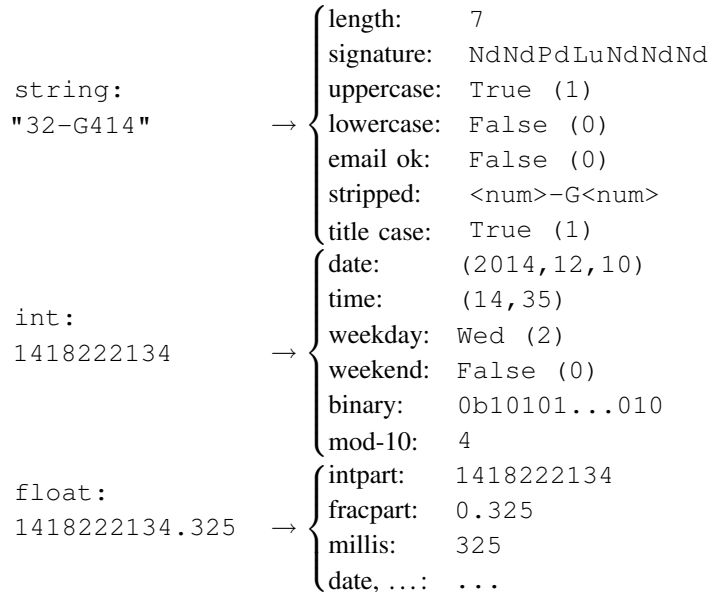
Fig. 2: Selected tuple expansion rules.
