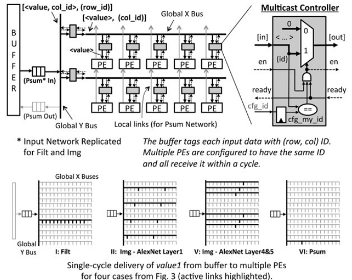
Figure 14.5.4: Network-on-Chip (NoC) for multicasting.
