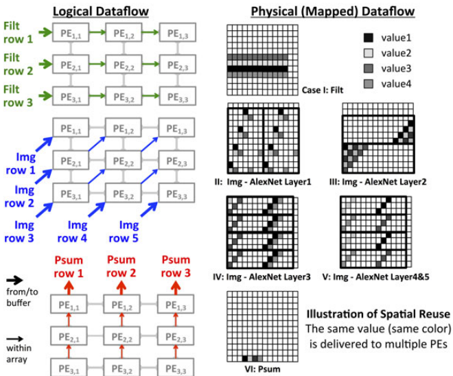
Figure 14.5.3: Logical and physical dataflows.
