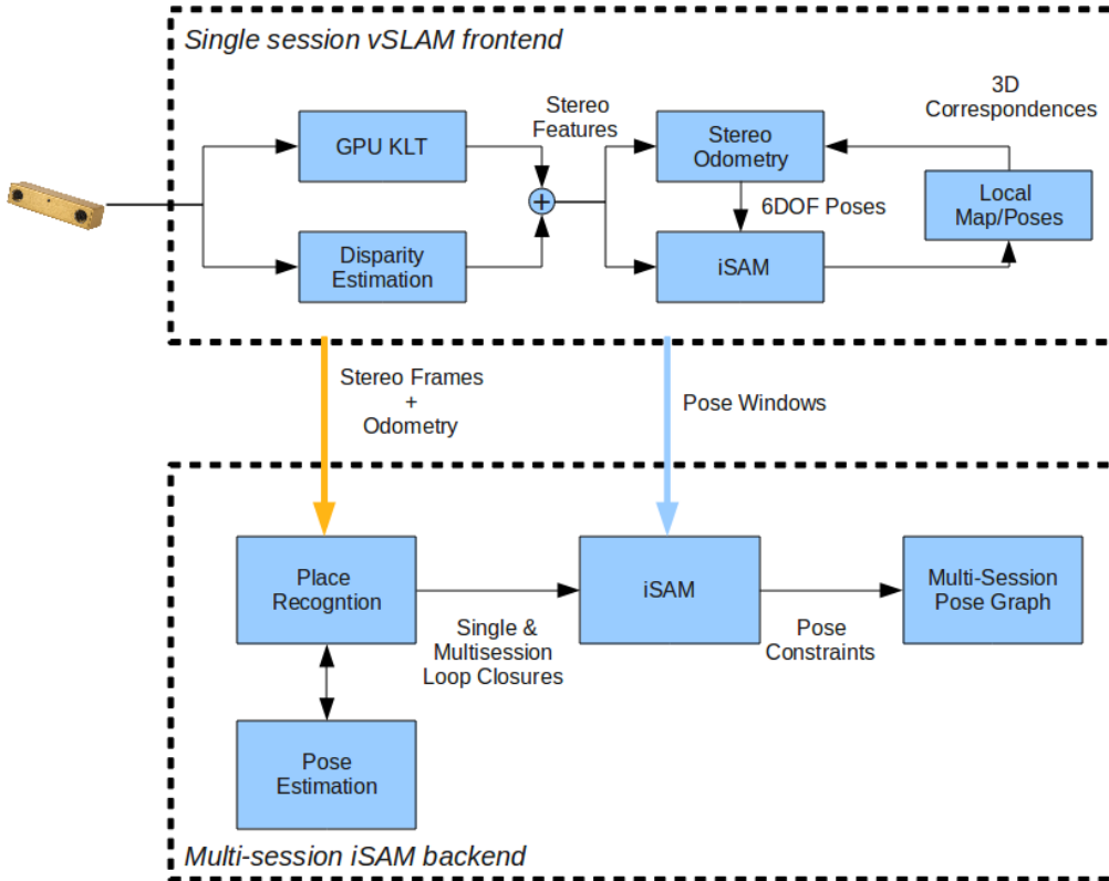
Figure 1: Internal architecture of windowed and multi-session visual SLAM (vSLAM) processes.
