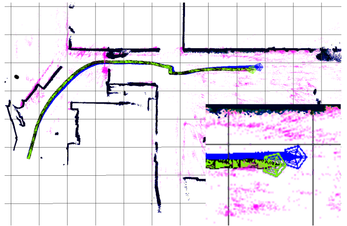
Figure 6: Comparison of drift in single session visual SLAM against 2D LiDAR scan matcher over a 20m trajectory. Grid scale is 2m. (For interpretation of the references to colour in the text, the reader is referred to the web version of this article.)
