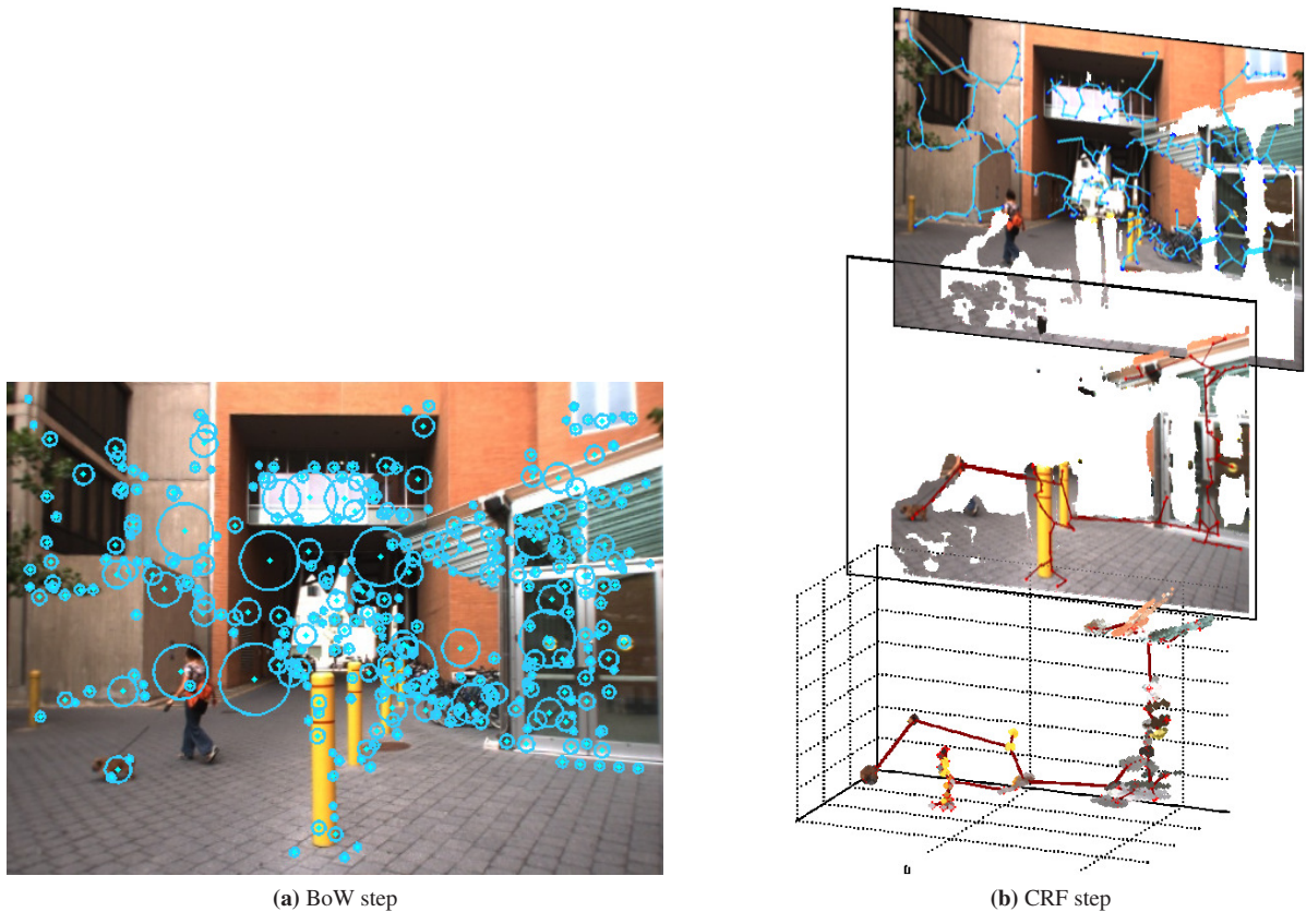
Figure 2: Illustration of steps involved in the combined BoW-CRF place recognition scheme. (a) For each input stereo pair we compute a set of SURF-features for one image of the stereo pair to provide the input of the BoW stage. (b) For the CRF stage we compute the two minimum spanning trees (MST), one for features with 3D information (near features), and the second for the remaining ones, with image information (far features). In (b), we show the two resulting graphs: in blue the graph for far features ( \mathcal{G}_{Im} ), in dark red the graph for near features ( \mathcal{G}_{3D} ). We apply CRF-Matching over both graphs. The minimum spanning tree of \mathcal{G}_{3D} is computed according to the metric coordinates, projected over the middle image only for visualisation. In the bottom, we show \mathcal{G}_{3D} in metric coordinates with the 3D point cloud (textured) of each vertex in the tree. The MST provides a representation of the dependencies between features in a scene, and allows for robust consistency checks of feature associations between scenes. (For interpretation of the references to colour in this figure legend, the reader is referred to the web version of this article.)
