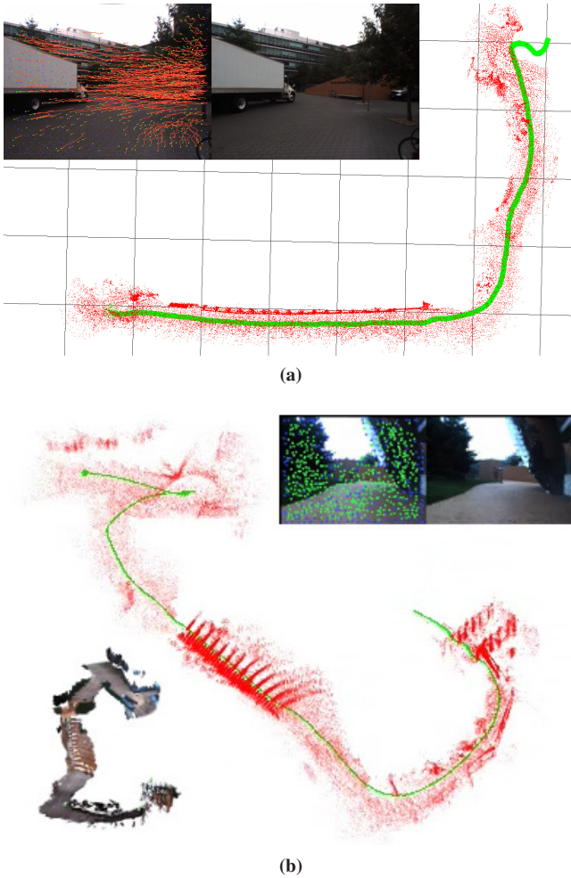
Figure 5: Single session visual SLAM processing including full 6-DOF motion.
