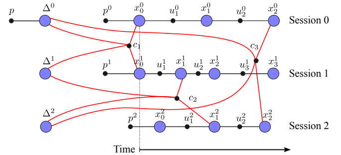
(d) The relative pose graph formulation generalizes to more than two sessions, and does not require the pose graphs to be synchronized or even to start at the same time or location. This example shows three encounters between three sessions.
