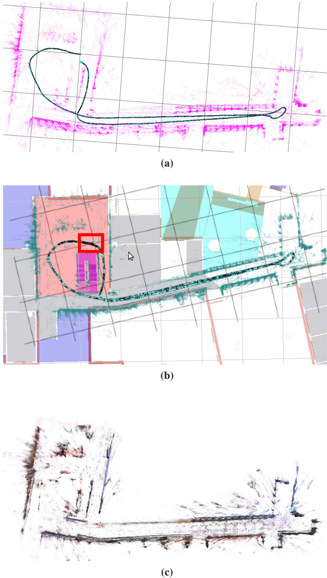
Figure 7: Single-session dataset containing a large loop. Here the grid scale is at 5m. (a) Map and pose graph prior to loop closure showing drift in position and structure. (b) Map and pose graph showing correction in the position and structure due to a series of loop closures in the area shown by the red square. Background image shows ground truth CAD floorplans of the environment. (c) Textured version of figure (b). (In order to fully interpret this figure the reader is referred to the online colour version.)
