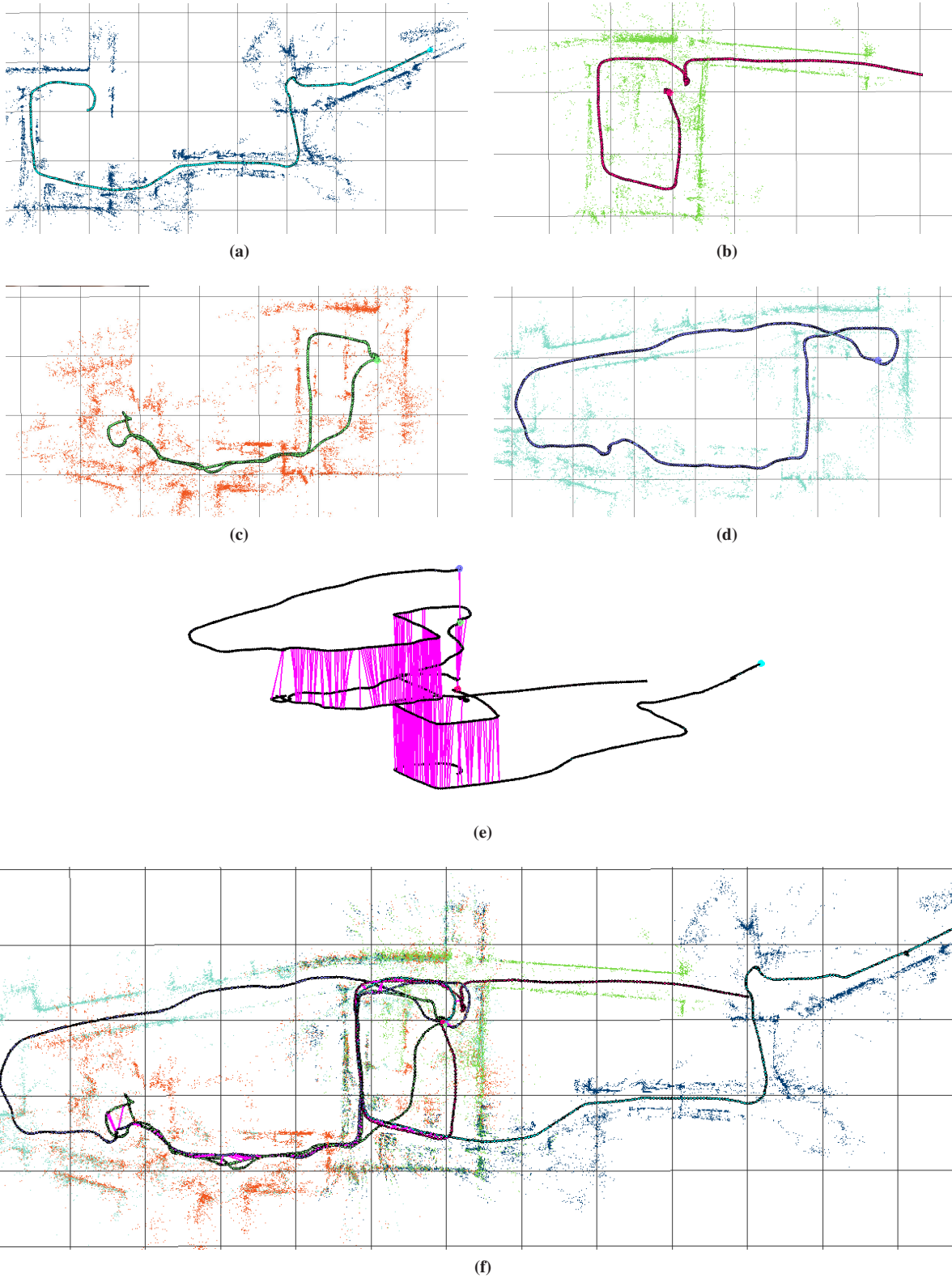
Figure 11: Stata Center second floor dataset with four separate sessions captured over a 75m \times 25m area. The underlying grid is set at a 5m scale in all figures. (a) – (d) show maps and pose graphs for each individual session. (e) shows the detected loops within and between pose graphs where the z-axis increase with time. (f) shows the combined multi-session map and pose graph. See Section 4.2 for further details. (In order to fully interpret this figure the reader is referred to the online colour version.)
