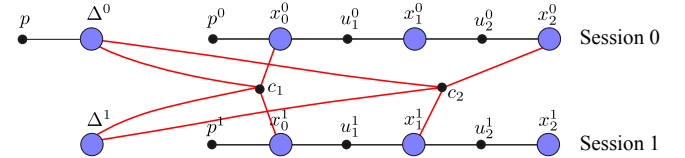
(c) The same encounters as in (b), but using the relative formulation from Kim et al. [3]. Here anchors \Delta^s are introduced for each trajectory that specify the offset of the trajectory with respect to a common global frame. Each encounter measurement now additionally connects to the anchors of both trajectories.
