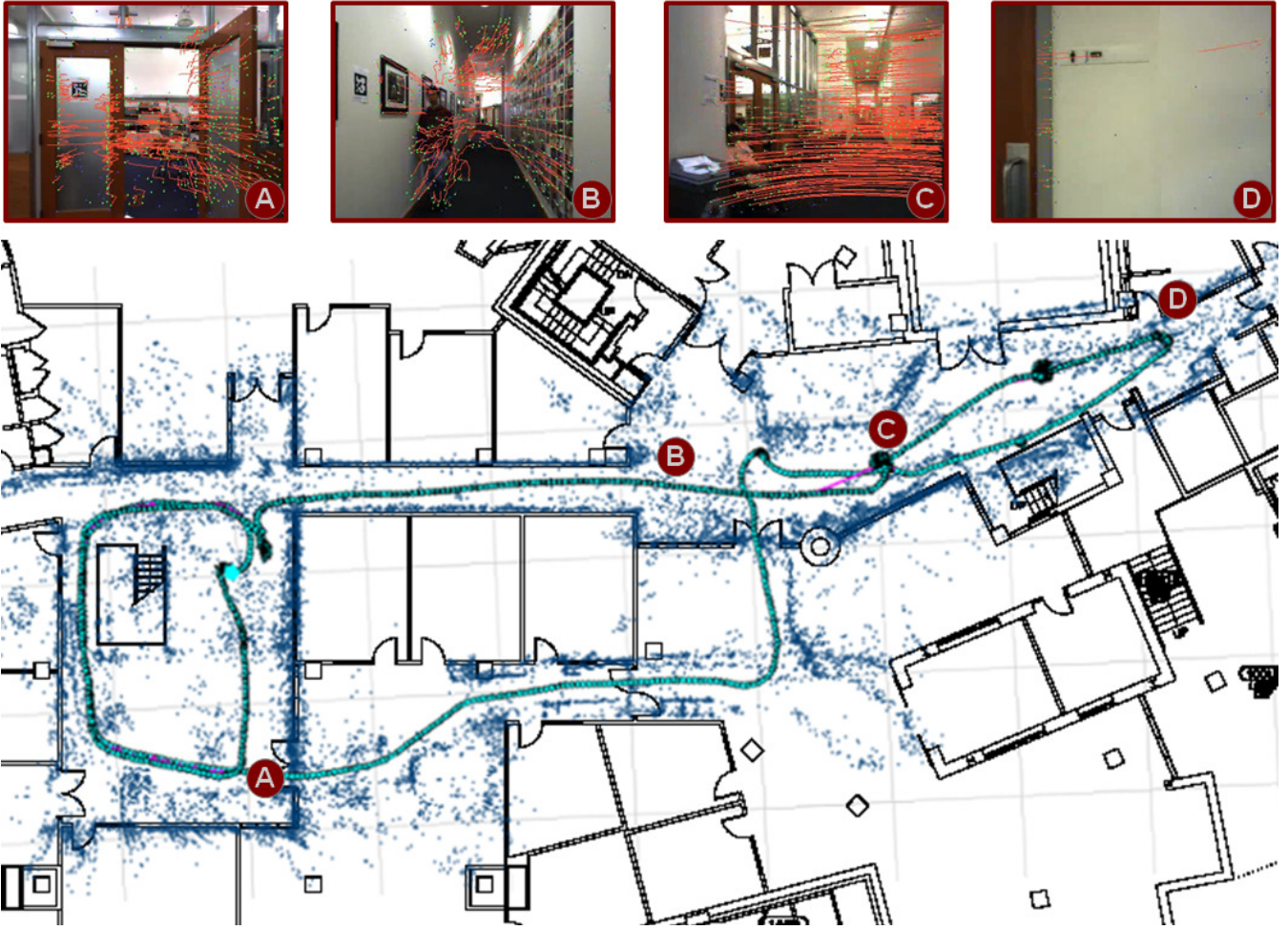
Figure 8: Top-down orthographic projection of the results for the Experiment 1 single session dataset described in Table 1. Here the map is overlaid on an architectural floorplan for comparison with ground-truth. The reference grid is shown at a scale of 5m. Images A–D displayed above the map show sample frames from the sequence with their approximate location highlighted on the map. Further details can be found in Section 4.1. (In order to fully interpret this figure the reader is referred to the online colour version.)
