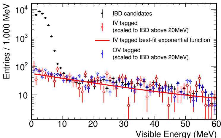
Figure 8. The IBD selection extended to 60 MeV in visible energy (black) together with the Fast Neutron spectrum (red and blue) obtained with an Inner Veto and Outer Veto tag (as explained in the text) normalized to the IBD above 20 MeV. The solid red curve shows the best fit to the Inner Veto tagged events, used to estimate the FN background in the signal region.
