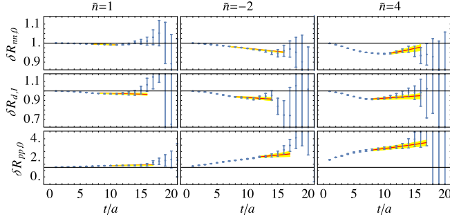
FIG. 1. Correlator ratios defined in Eq. (2) for the mn , the j_z = +1 deuteron and pp systems for field strengths \tilde{n} = 1, -2, 4 , for the m_\pi \sim 450 MeV ensemble. The bands correspond to the exponential fit and its statistical uncertainties associated with the shown fit interval. Systematic uncertainties from the choice of fit range are separately assessed.
