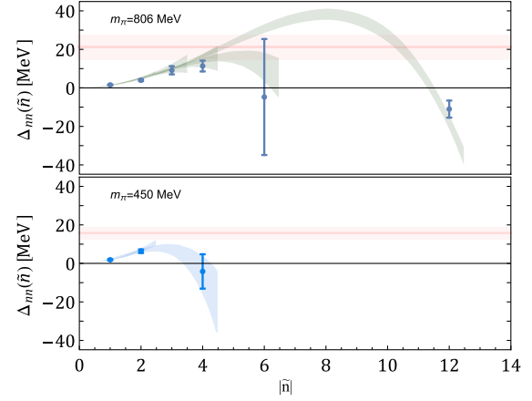
FIG. 2. Response of the binding of the dineutron system to applied magnetic fields. The upper panel shows the result at m_\pi = 806 MeV, while the lower panel is for m_\pi = 450 MeV. The shaded regions correspond to the envelopes of successful fits to the energy shifts using linear and quadratic polynomials in \tilde{n}^2 to data points in the corresponding range indicated by the shaded region. The horizontal bands indicate the binding threshold.
