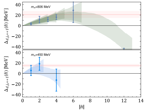
FIG. 3. Response of the binding of the j_z = +1 state of the deuteron to applied magnetic fields. The shaded regions correspond to the envelopes of successful fits to the energy shifts using polynomials in \tilde{n} of up to 4th (2nd) order for the m_\pi = 806 (450) MeV ensemble. The horizontal bands indicate the binding threshold.
