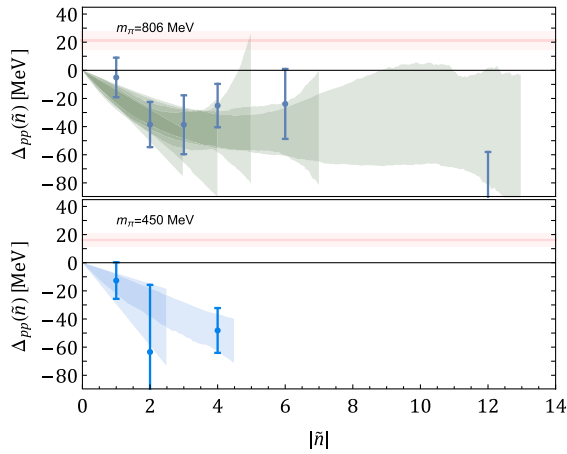
FIG. 4. Response of the binding of the diproton to applied magnetic fields. The shaded regions correspond to the envelopes of successful fits to the energy shifts using polynomials in \tilde{n} of up to 4th (2nd) order for the m_\pi = 806 (450) MeV ensemble. The horizontal bands indicate the binding threshold.
