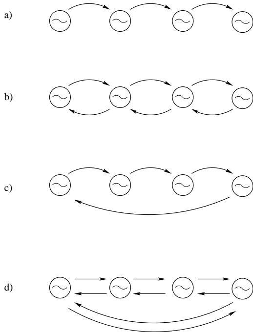
Fig. 6. Chain array topologies: a) and b) open array with unidirectional and bidirectional coupling, respectively, c) d) unidirectional and bidirectional array closed in feedback.
