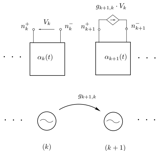
Fig. 5. Coupling in a chain array: (top) the voltage across the k th oscillator controls the current injected into the k+1 oscillator (bottom) schematic representation of this local coupling.
