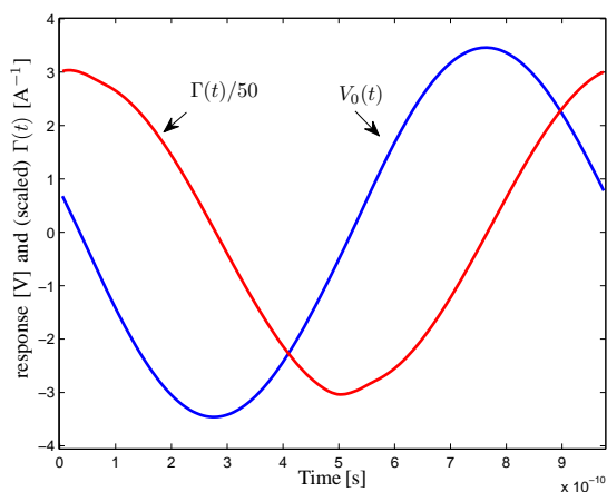
Fig. 2. Free-running response and function \Gamma(t) of an LC oscillator.
