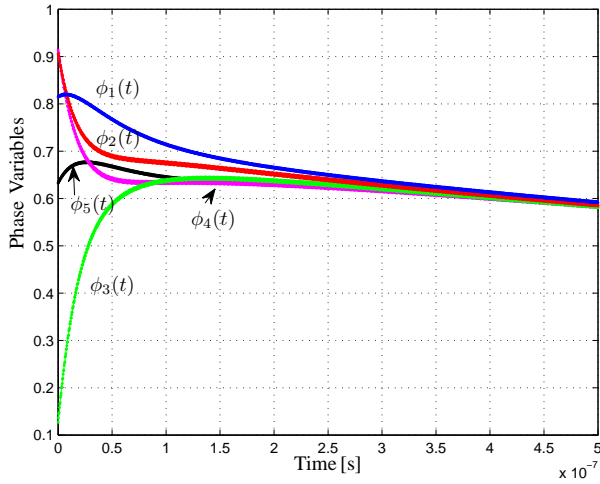
Fig. 8. Setting 1): phase variables converge to the same waveform.
