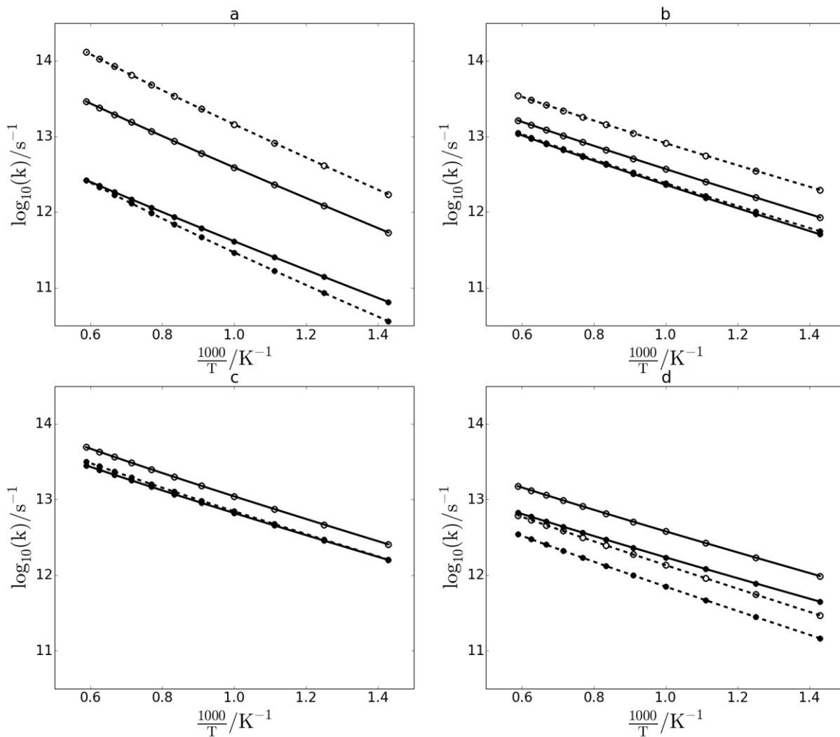
Figure 1: Rate coefficients as a function of temperature. Cyclopentyl and norbornyl decomposition reaction rate coefficients from Sirjean et al. 63, 64 . Tricyclodecyl decomposition reaction rate coefficients calculated in this work. Tricyclodecyl decomposition reactions are represented by full symbols.
