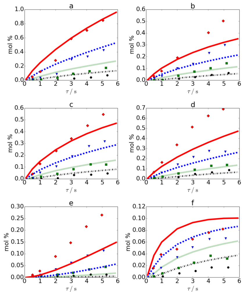
Figure 4: Mole fractions as a function of residence time of a) dihydrogen, b) propene, c) 1,3-cyclopentadiene, d) ethene, e) methane, f) cyclopentene at four temperatures: \blacklozenge 933K, \blacktriangledown 913K, \blacksquare 893K, \bullet 873K. Lines are model predictions, symbols are Nancy data 10 . Conditions: 4 mol% exo-TCD in He at the reactor inlet, T = 848 -933K, P = 1 \cdot 10^5 Pa, conversion = 0.01-25%.
