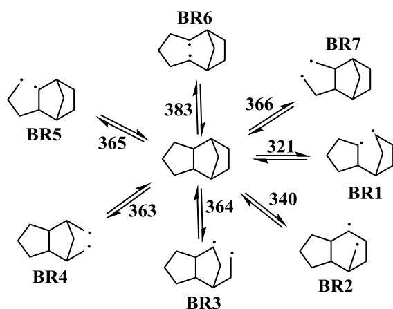
Scheme 2: Exo-TCD initiation routes through unimolecular C–C scission reactions resulting in seven biradicals, BR x , x=1..7. Nomenclature for the biradicals is adopted from Herbinet et al. 10 . Values represent standard reaction enthalpies (kJ mol -1 ) at 298K, based on thermochemistry used in this model.
