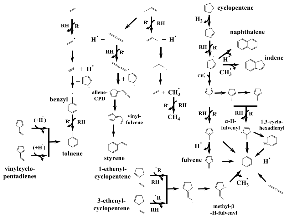
Scheme 6: Pathways of secondary conversion of primary products relevant at T=1100K, P=1.7 10 5 Pa.
