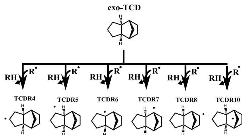
Scheme 2: Six possible C_{10}H_{15} tricyclodecyl radicals created by H-abstraction reactions from exo-TCD. Nomenclature for the tricyclodecyl monoradicals is adopted from Hudzik et al. [1].
