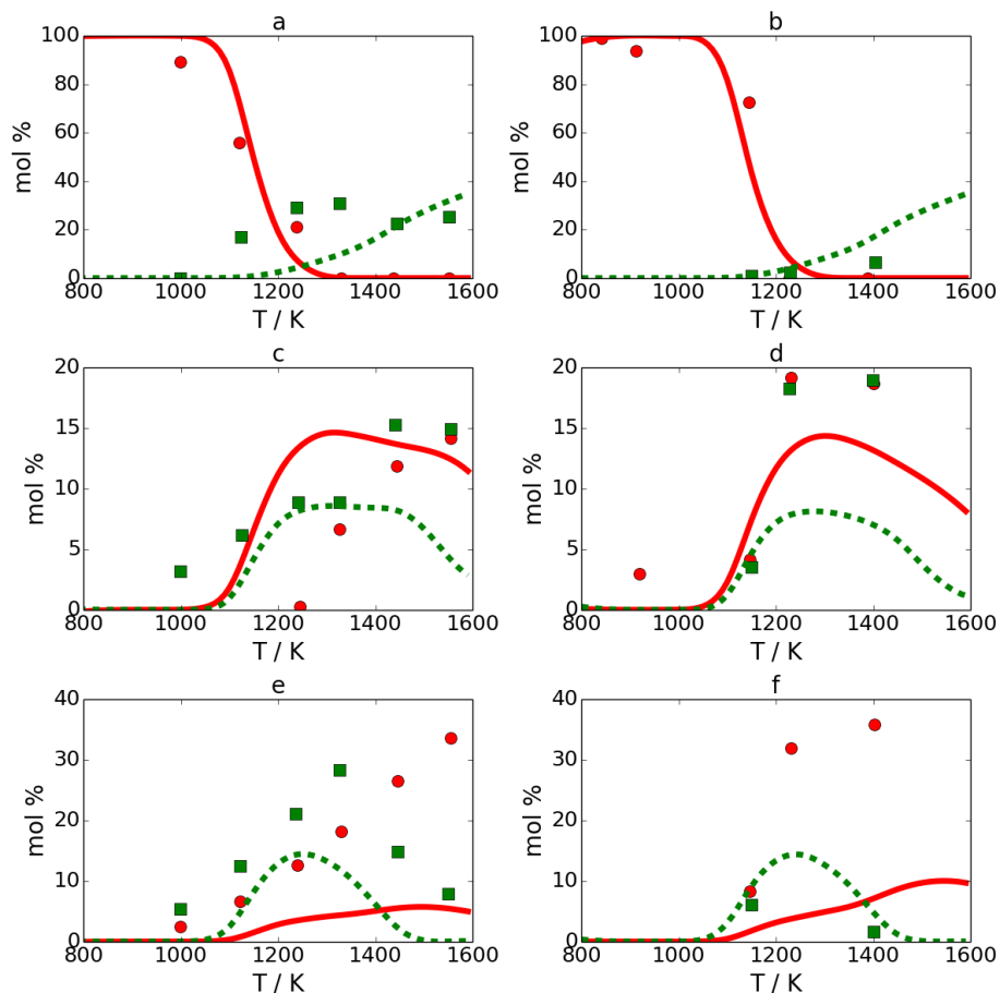
Figure 6: Mole fractions as a function of reactor temperature for model predictions versus Nakra data 13 (left column) and Van Devener data 14 (right column). a) and b) experiments: ● exo-TCD, ■ ethyne, model predictions: —: exo-TCD, - -: ethyne, c) and d) experiments: ● ethene, ■ propyne, model predictions: —: ethene, - -: propyne, e) and f) experiments: ● benzene, ■ 1,3-cyclopentadiene, model predictions: —: benzene, - -: 1,3-cyclopentadiene. Conditions for the Nakra 13 and Van Devener 14 data respectively: 2.6 / 3.9 mol% JP-10 in Argon, P = 300-400 / 1500-1900 Pa, conversion = 0-100%.
