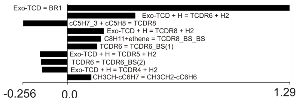
Figure 9: Normalized sensitivity coefficients for benzene at T = 1100K , P = 1.7 \cdot 10^5 Pa, corresponding to an exo-TCD conversion = 36%. “BS” indicates that the species represents is formed through a \beta -scission reaction of the reactant.
