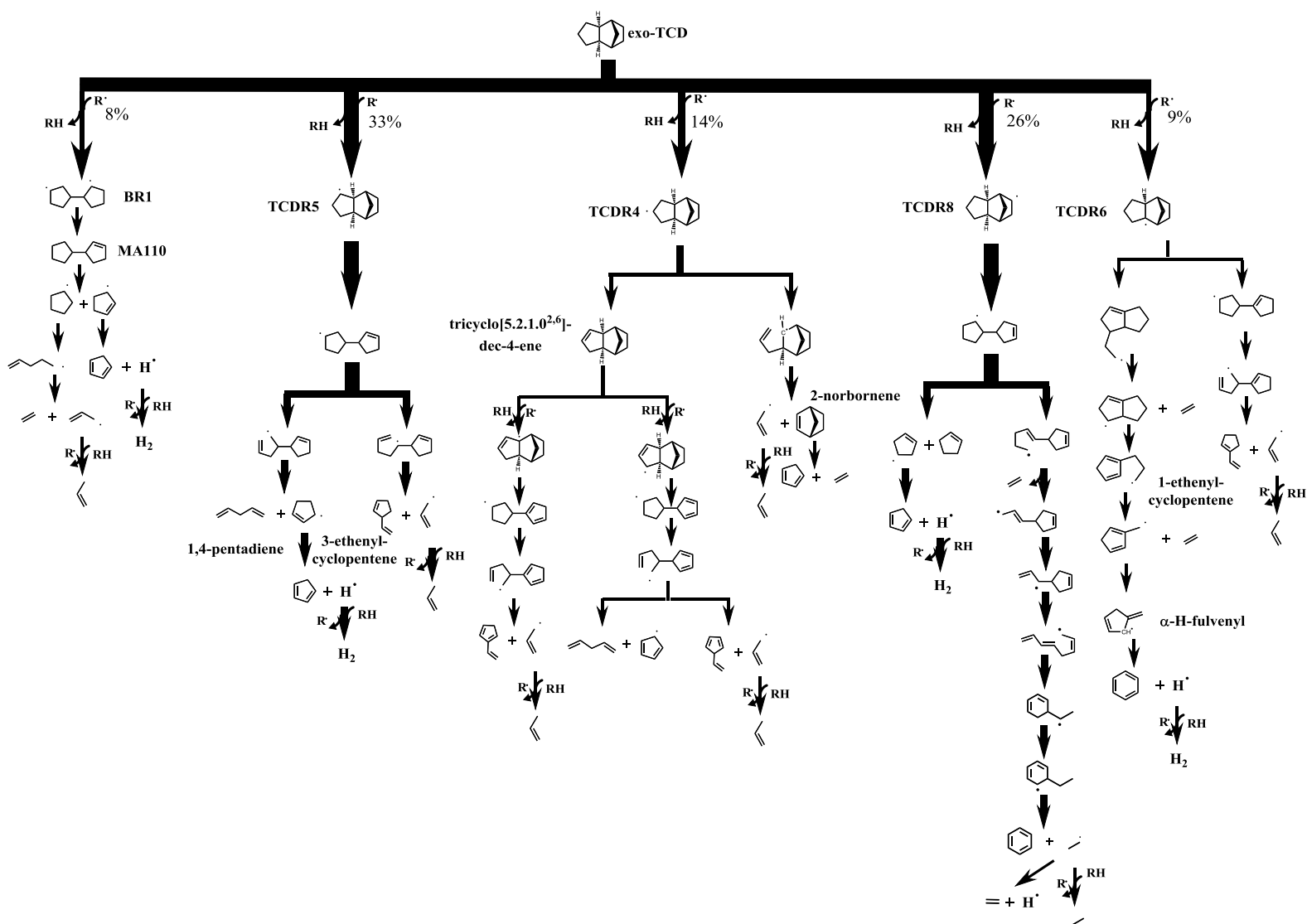
Scheme 5: Reaction pathway analysis for the decomposition of exo-TCD. The reported percentages represent the predicted reaction rate relative to the total exo-TCD decomposition rate. T=1100K, P=1.7 10 5 Pa, Conversion exo-TCD = 19%, 10 mol% exo-TCD in N 2 corresponding to conditions of the Ghent data set. Only major exo-TCD decomposition pathways are shown.
