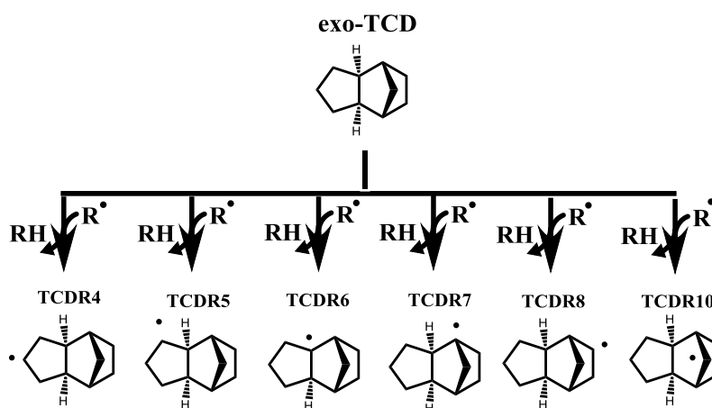
Scheme 4: Six possible C 10 H 15 tricyclodecyl radicals created by H-abstraction reactions from exo -TCD. Nomenclature for the tricyclodecyl monoradicals is adopted from Hudzik et al. 47 .
