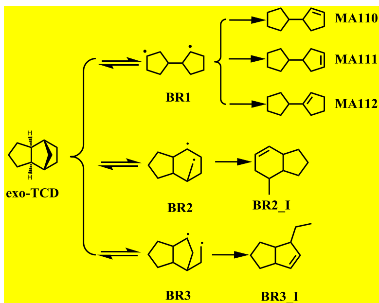
Scheme 3: The unimolecular C-C scission of exo-TCD yielding biradicals and subsequent intramolecular H-abstraction reactions yielding molecular intermediates taken into account in this work.
