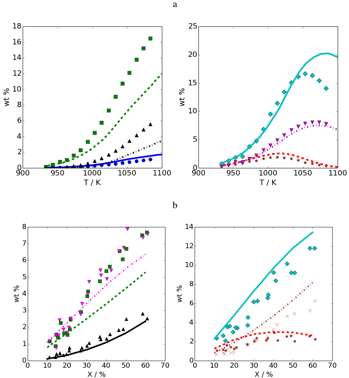
Figure 3: a) Mass fractions as a function of temperature for the Ghent data 18 . Left: ● dihydrogen, ▲ methane, ■ ethene, —: dihydrogen, - -: methane, - -: ethene. Right: ◆ 1,3-cyclopentadiene, ▼ propene, * cyclopentene, —: 1,3-cyclopentadiene, - -: propene, - -: cyclopentene. Conditions: 10 mol % JP-10 in N 2 at reactor inlet. P = 1.7 10 5 Pa. b) Mass fractions as a function of exo-TCD conversion for the Rao data 12 . Left: ▲ methane, ▼ propene, ■ ethene, — methane, - - propene, - - ethene. Right: * cyclopentene, × benzene, ◆ 1,3-cyclopentadiene, - - cyclopentene, - - benzene, — 1,3-cyclopentadiene. Conditions: 100 mol % JP-10 at
