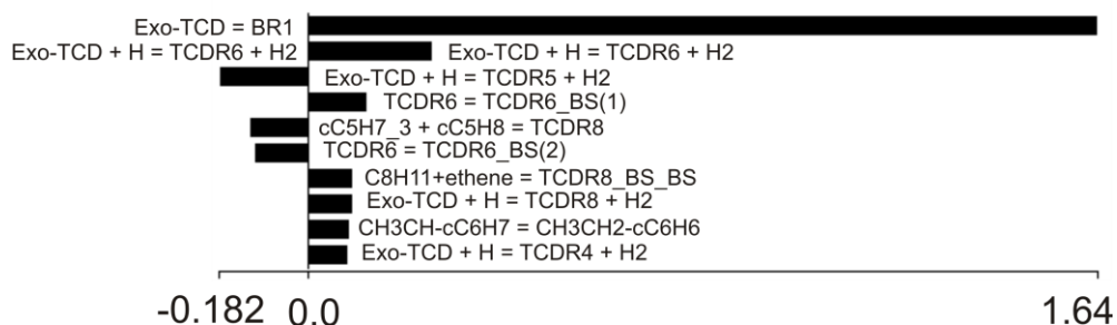
Figure 8: Normalized sensitivity coefficients for ethene at T = 1100\text{K} , P = 1.5 \cdot 10^5 \text{ Pa} , corresponding to an exo-TCD conversion = 16%. “BS” indicates that the species represents is formed through a \beta -scission reaction of the reactant.
