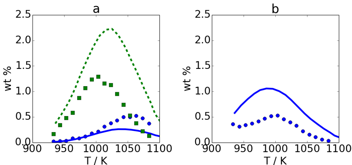
Figure 7: Mass fractions as a function of temperature for the Ghent data 18 for a) ● 1-methyl-1,3-cyclopentadiene, ■ 3-ethenylcyclopentene, —: 1-methyl-1,3-cyclopentadiene, - -: 3-ethenylcyclopentene, b) ● tricyclo(5.2.1.0 [2,6] )dec-4-ene, —: tricyclo(5.2.1.0 [2,6] )dec-4-ene. Conditions: 10 mol % JP-10 in N 2 at reactor inlet. P = 1.7 10 5 Pa. Symbols are experimental data, lines are model predictions.
