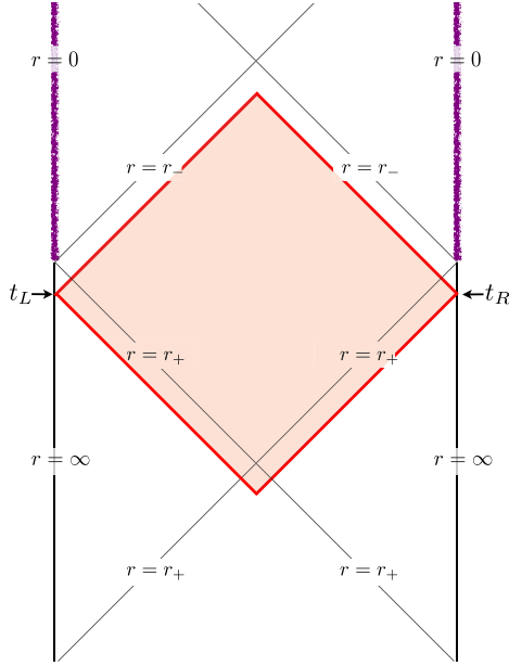
FIG. 2. For a charged AdS black hole, the Wheeler-DeWitt patch does not extend all the way to the singularity, and instead ends when the ingoing light sheets self-intersect just outside the inner horizon at r_- .
