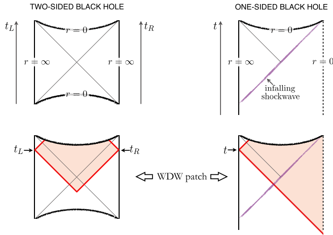
FIG. 1. The two-sided eternal AdS black hole (left) and a one-sided AdS black hole that forms from a collapsing shockwave (right). The two-sided AdS black hole is dual to an entangled (thermofield double) state of two CFTs that live on the left and right boundaries; the one-sided black hole is dual to a single CFT. Our complexity-action conjecture relates the complexity of the CFT state to the action of the Wheeler-DeWitt patch (shown shaded).
