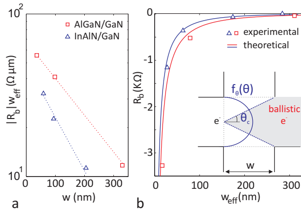
FIG. 4. Experimental determination of the characteristic ballistic length for both heterostructures. a. Logarithmic scale plot of w_{\text{eff}}|R_b| versus w for both InAlN/GaN and AlGaN/GaN heterostructures at 4 K. The characteristic ballistic length L_b was extracted from the slope of these curves. b. Bend resistance R_b versus effective cross width w_{\text{eff}} = w - w_{\text{dep}} (squares for AlGaN/GaN and triangles for InAlN/GaN), along with the theoretical curves (solid lines). (Inset) Schematic of the ballistic transmission of electrons to the opposite lead in these crosses.
