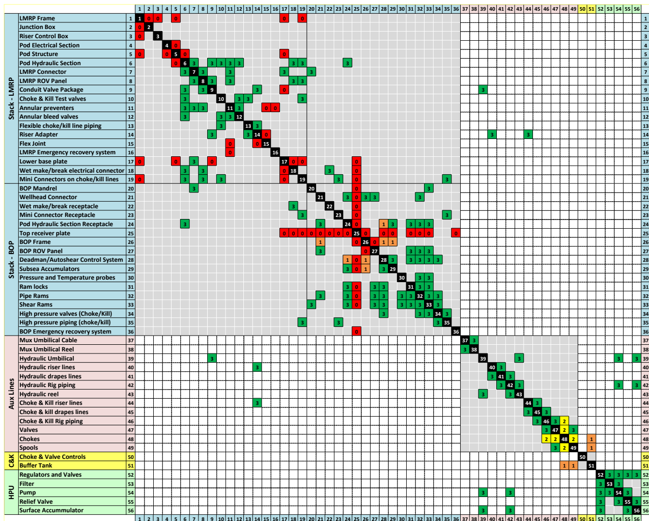
Figure 7: Maximum Structural Integration Level DSM
