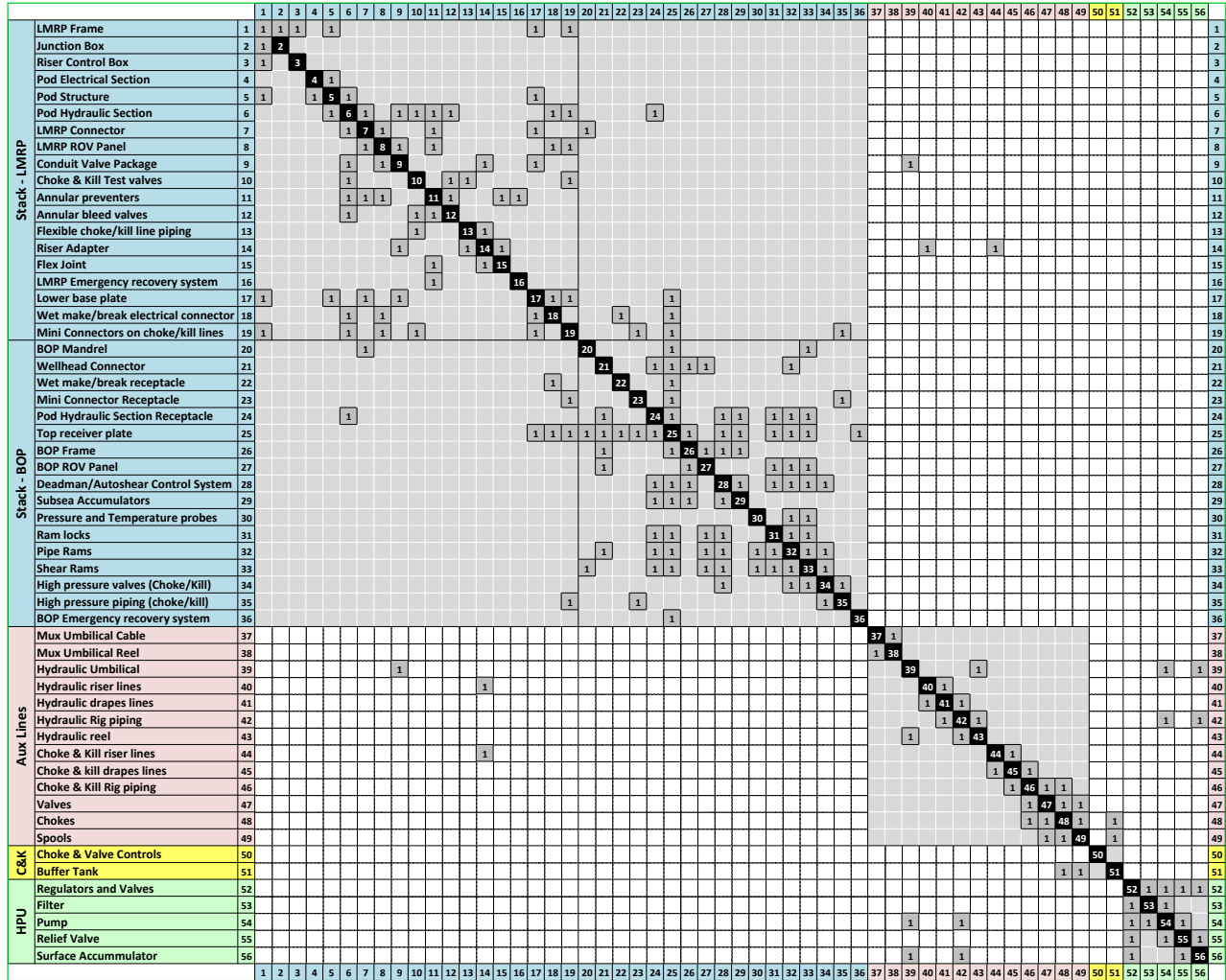
Figure 3: System Architecture DSM Representation of Structural Interactions between Components
