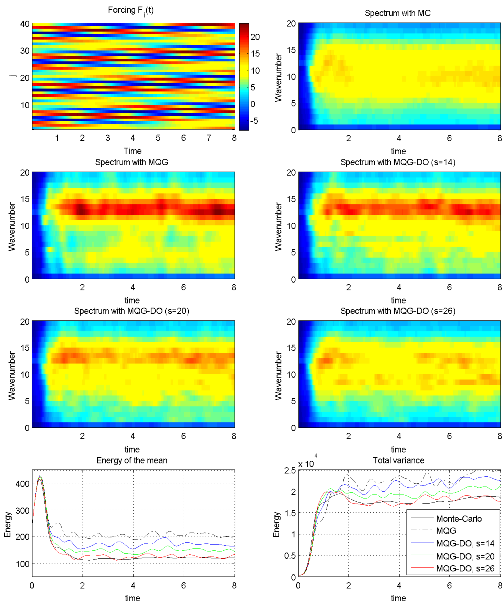
Figure 8: Lorenz 96 system with extreme time and space dependent forcing. The performance of MQG and MQG-DO methods (for various s ) is shown and compared with Monte-Carlo in terms of the spectrum, the energy of the mean, and the total stochastic energy.
