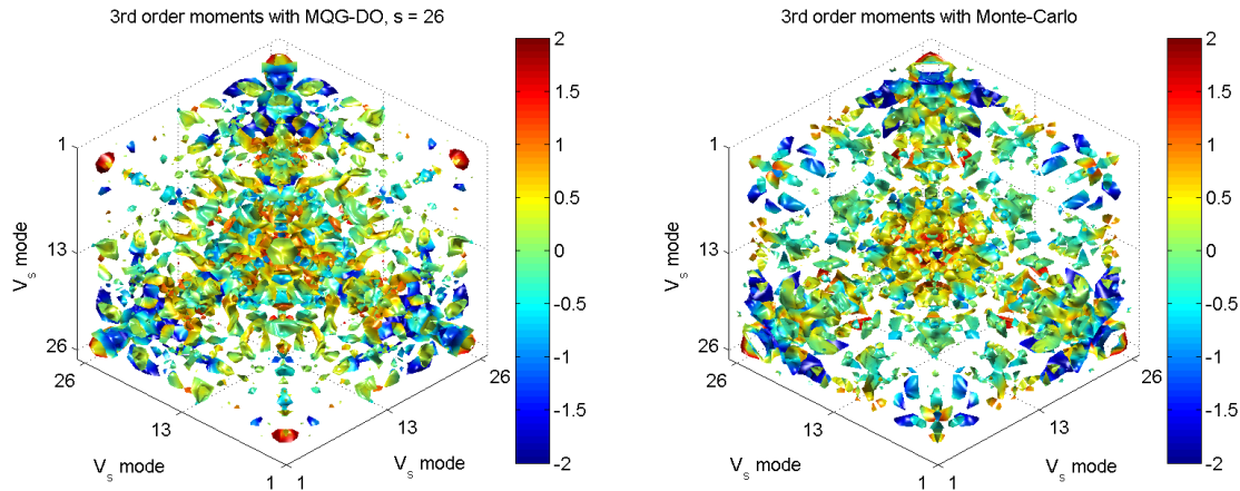
Figure 10: Comparison of third-order central-moments for Lorenz 96 subjected to extreme excitation. The moments inside the subspace are shown (for t = 8 ) computed with MQG-DO ( s = 26 ) and Monte-Carlo. The visualization follows the same technique used in Figure 2.
