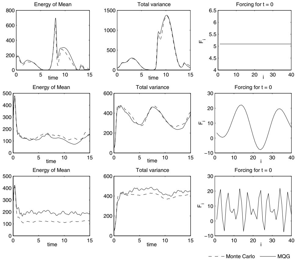
Figure 4: Comparison of MQG UQ scheme (solid line) with Monte-Carlo (dashed line) in L-96 for different spatial dependence of the forcing F_i(t) (eq. (19)). First row: a = 0 - no spatial dependence; second row: a = 0.2 - weak spatial dependence; third row: a = 1 - strong spatial dependence. The tuning of the fluxes has been made using steady state statistics that correspond to constant forcing F = 8 .
