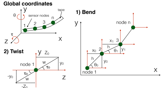
Figure 7. The graphical representation of bending and twisting calculations. The bending only happens in the X-Y plane and twisting in the Y-Z plane.
