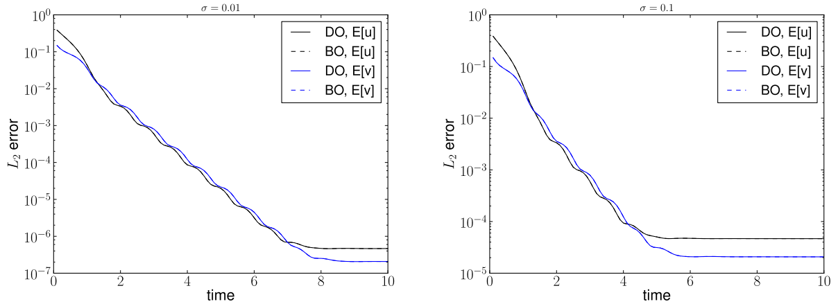
Figure 14: L_2 error for the mean of the solution in time: \sigma = 0.01 (left) and \sigma = 0.1 (right). It converges to the steady solution after time t = 8 ( \sigma = 0.01 ) and t = 6 ( \sigma = 0.1 ).
