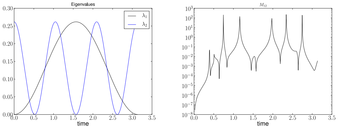
Figure 6: Left: eigenvalues, right: M_{12} . The eigenvalues cross out at the six locations at which M_{12} peaks as shown in the right figure.
