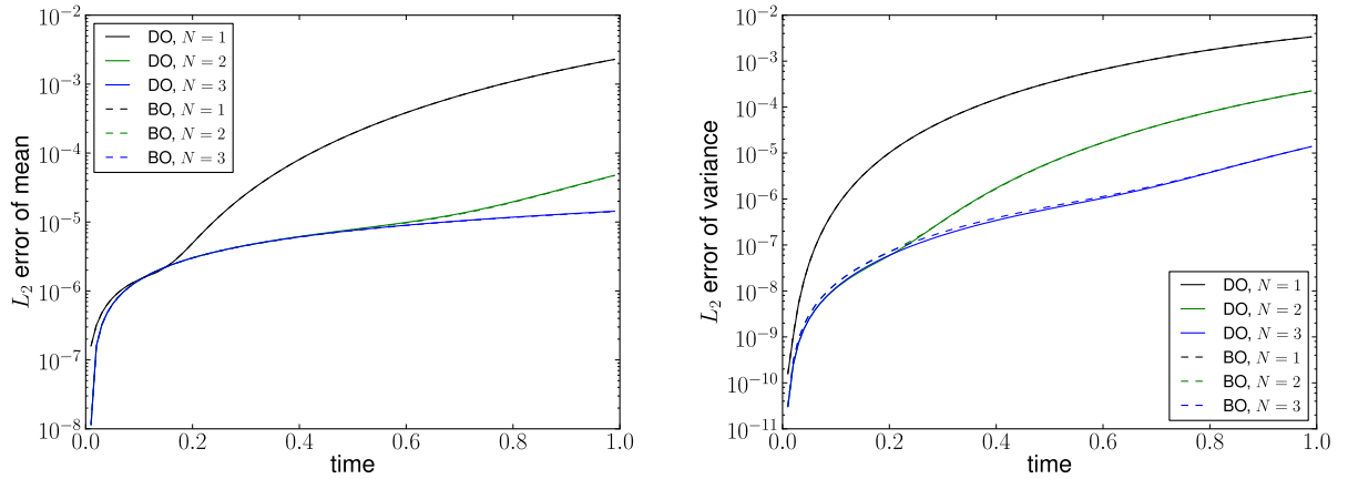
Figure 8: Advection-diffusion: one-dimensional parametric space with \xi_1 = \xi_2 = 0.1\xi . The error of the mean (left) and variance (right) versus time with respect to different number of modes.
