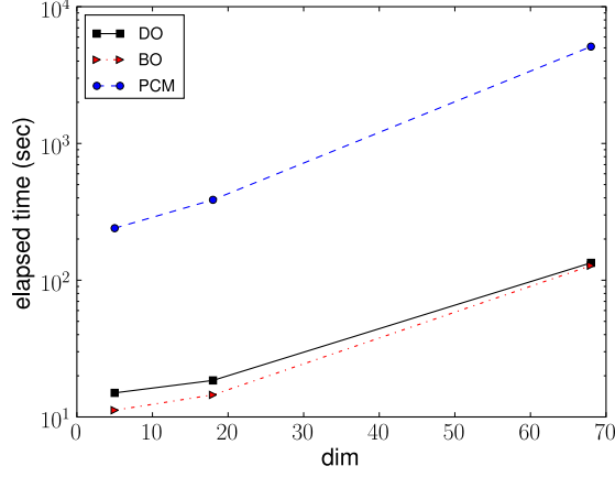
Figure 2: Computational time on Intel Xeon X5550 2.67GHz to solve the advection problem up to time t = 5 using DO, BO and PCM. DO is much faster than PCM, especially in high dimensions, and BO is slightly faster than DO for low dimensions.
