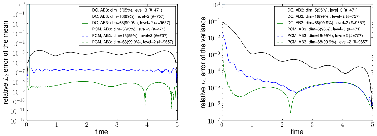
Figure 1: Relative L_2 error for the mean (left) and variance (right). The reference solution for the mean and variance is from the exact formula. As we increase the dimension of the random space i.e. we approximate V(t; \omega) better with more terms, the relative L_2 error decreases. Note that BO results do not appear in these plots but they have exactly the same accuracy as DO. (AB3 refers to the third-order Adams-Bashforth integration, and "level" refers to the level of the sparse grid.)
