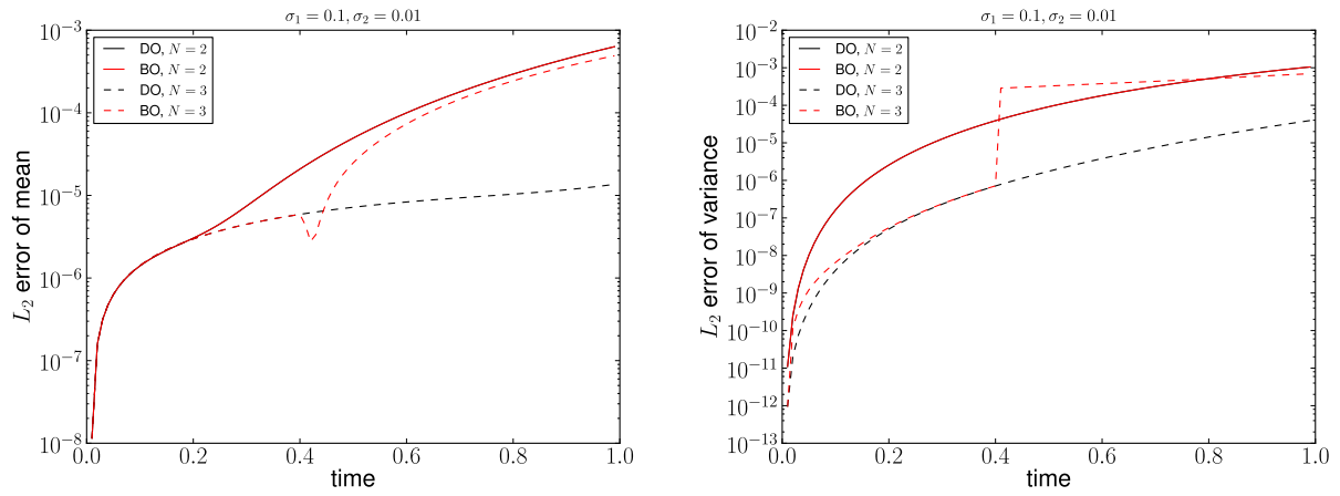
Figure 9: Case I. The DO and BO are tested with different number of modes. As we increase the number of modes, the convergence improves. For N = 3 , the error in the BO increases suddenly around t = 0.4 because of the eigenvalue crossing.
