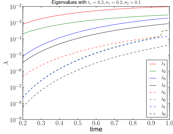
Figure 13: Case II with t_s = 0.2 . The eigenvalue crossing occurs around t = 0.95 .
