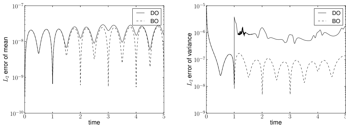
Figure 3: Relative L_2 error for the mean (left) and variance (right) of the solution for the Burgers equation with random forcing using DO and BO with N = 6 . Both methods have the same accuracy for the mean while BO is an order of magnitude more accurate compared to DO for the variance. BO is numerically more stable than DO for high modes while they have the same accuracy for low modes. Note that the switching time is 1 and the error before the switching time is the same as collocation method is used in the hybrid method.
