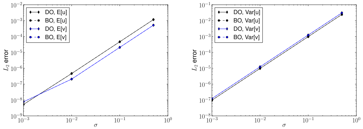
Figure 15: L_2 error for the mean (left) and variance (right) of the steady state solution for the Kovaszny flow versus the magnitude using DO and BO.
