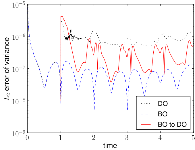
Figure 5: Relative L_2 error for the variance at t = 5 with N = 6 . The top one is the variance from the DO evolution equations; the bottom from the BO evolution equations; the middle one from the DO components via the dynamical transformation from the BO.
