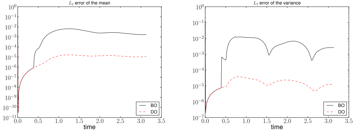
Figure 7: Left: mean, right: variance. Both the error of the mean and variance in BO jumps when the eigenvalues cross while the error in DO does not.
