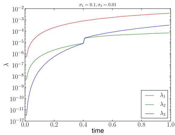
Figure 10: Case I. The eigenvalue crossing occurs around t = 0.4 .
