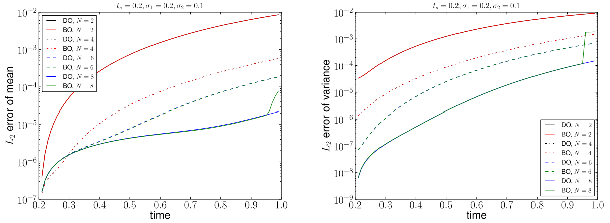
Figure 12: Case II with t_s = 0.2 . L_2 error of the mean and variance.
