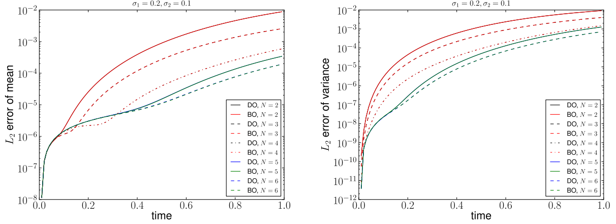
Figure 11: Case II with t_s = 0.01 . L_2 error of the mean and variance.
