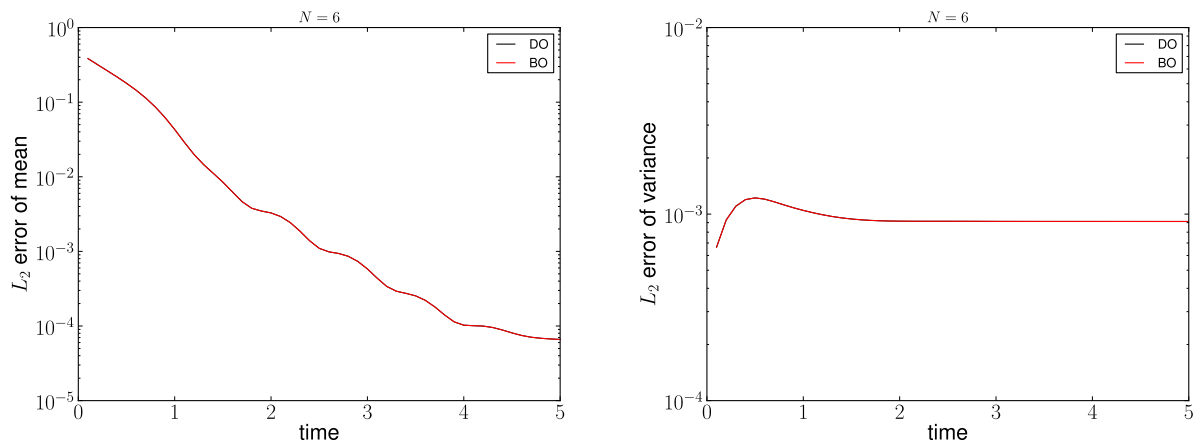
Figure 16: L_2 error for the mean and variance in time with six dimensional parametric space.
