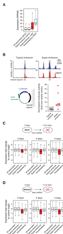
Figure 3. Super-enhancers confer high transcriptional activity and sensitivity to perturbation
