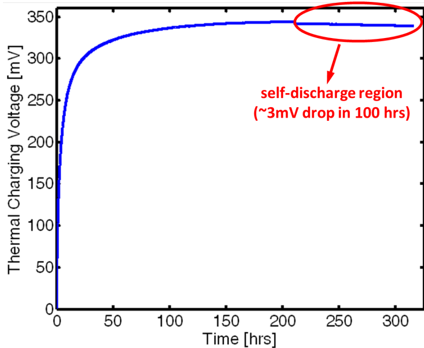
Figure S1. An extremely long-time thermal charging experiment to investigate the self-discharge behavior of the thermally charged EDLC. The thermal charging voltage reaches saturation after about 210 hours. Then the voltage of the EDLC starts to decrease which indicates the EDLC is self-discharging. However, the voltage drops only 3mV in about 100 hours, which means the self-discharge of the thermally charged voltage is negligible.
