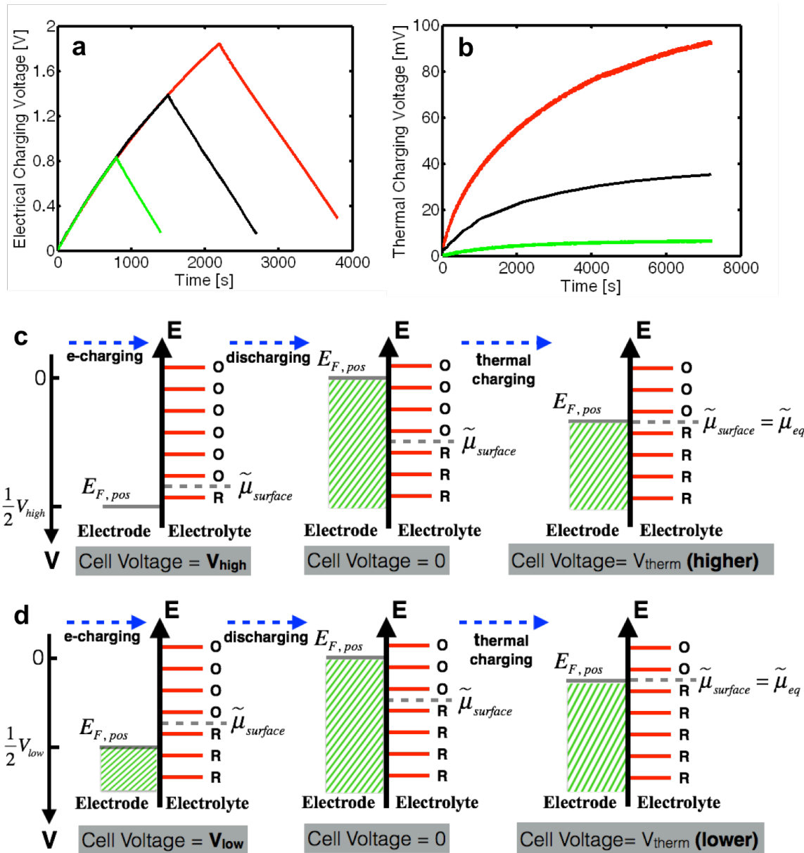
Figure S5. Effect of electrical charging voltage cut-off on “thermally charged” voltage (a) Voltage profiles of the activation step with different charging voltage cut-off. The red, black and green curves are electrically charged to 1.85V, 1.39V, and 0.83V, respectively. (b) The corresponding three “thermal charging” curves. Higher electrical charging voltage cut-off in the activation step results in higher “thermally charged” voltage. (c) and (d) Corresponding mechanism for high charging voltage cut-off (c) and low charging voltage cut-off (d) (only the positive electrode is illustrated). When the electrically charged voltage cut-off is high, the functional group at higher reaction potential can be oxidized. As a result, after electrical discharging, there are more functional groups in the oxidized state with high electrical charging voltage cut-off compared to that with low electrical charging voltage cut-off. Consequently the final “thermally charged” voltage can reach a higher value.
