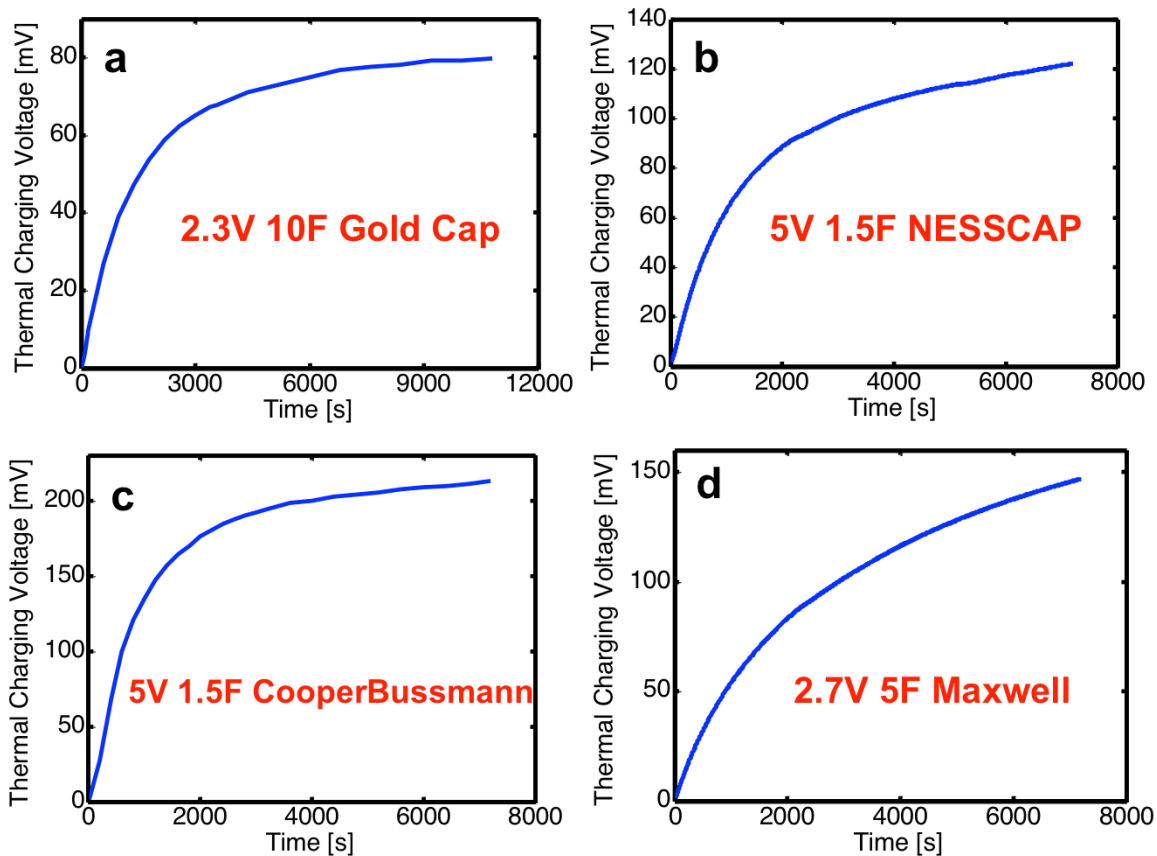
Figure S3. “Thermal charging” experiments for different types of commercial EDLCs, indicating that the “thermal charging” is a universal phenomenon in EDLCs. All these “thermal charging” experiments were conducted after electrical activation, and the activation currents for these four types of EDLC are: a) Gold Cap: 5mA, b) NESSCAP: 10mA, c) CooperBussmann: 10mA, d) Maxwell: 10mA.
