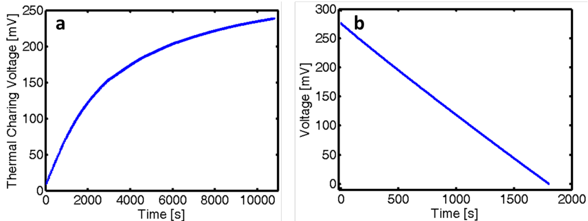
Figure S2. a) “Thermal charging” of a Maxwell (2.7V 5F) EDLC after three successive electrical charge/discharge activation cycles using cyclic voltammetry method with a scan rate of 0.1mV/s and scan range 0-2.6V. The “thermally charged voltage at 60°C for 3 hours is about 240mV; b) Constant current discharge curve for the same EDLC to measure its capacitance, which is the current divided by the slope of this discharging curve. The measured capacitance for this EDLC is 6.52F, which is similar to the nominal capacitance of this EDLC 5F. Note the initial voltage of the EDLC is about 275mV which is larger than 240mV. This is because after the “thermal charging” at 60°C, the capacitor was kept at room temperature for 5 days (Room temperature “thermal charging” causes the voltage slightly increase during the 5 days). This is also an evidence that the “thermally charged” voltage can be kept when the capacitor goes from high temperature to low temperature.
