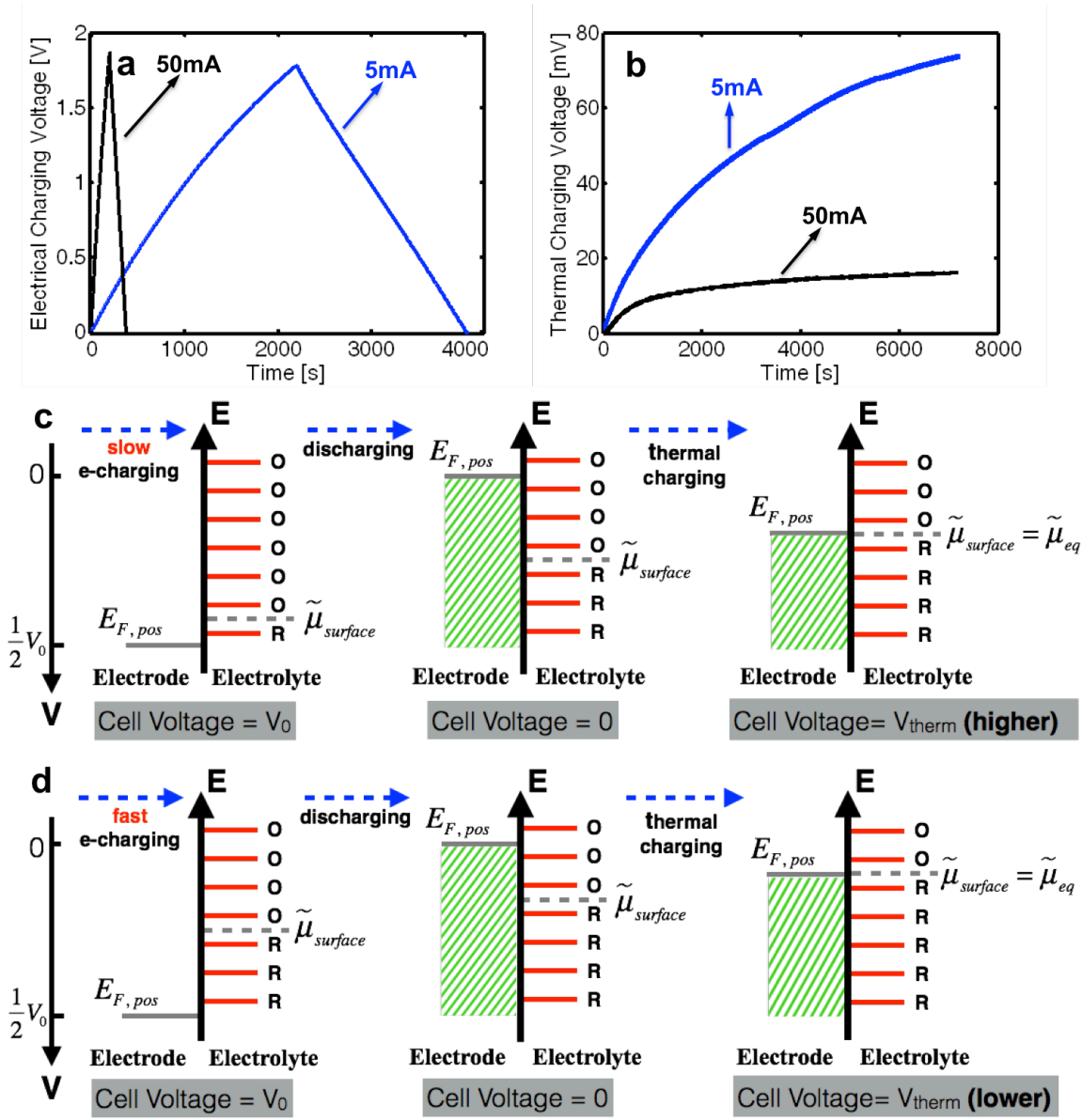
Figure S6. Effect of electrical charging current rates on “thermally charged” voltage. (a) Voltage profiles of activation step with different currents. The black and blue ones correspond to 50mA and 5mA, respectively. (b) The corresponding “thermally charged” voltage curves. Slower electrical charging current during the activation step results in higher “thermally charged” voltage. (c) and (d) Corresponding mechanism for different electrical charging current rates (only the positive electrode is illustrated). The processes with low and high currents are represented in (c) and (d), respectively. When the electrical charging process is slow (c), more functional groups have enough time to be oxidized, especially at high reaction potential. Then after electrical discharging, more functional groups in the oxidized state will be left at the electrode surface. (d) When the electrical charging process is fast, most functional groups in the reduced state do not have enough time to be oxidized, especially for those with high reaction potential. Then after the electrical discharging step, less functional groups in the oxidized state are left at the electrode
