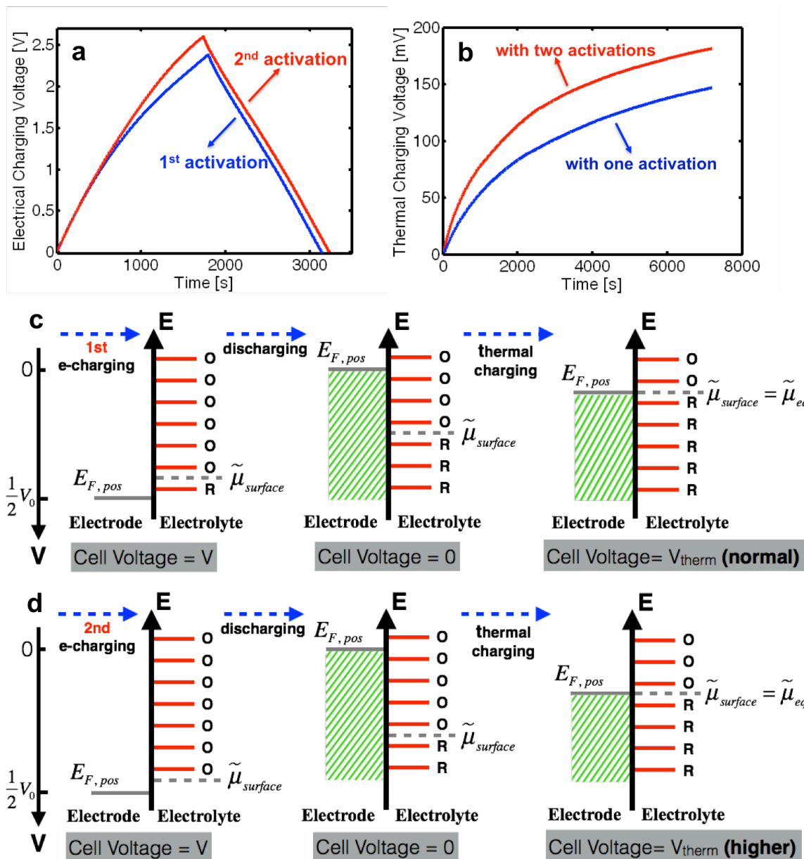
Figure S7. Effect of multiple times electrical charging on “thermally charged” voltage. (a) Blue line represents a capacitor with only one activation, and red line represents the same type capacitor with two activations (charge/discharge cycle). (b) The corresponding “thermal charging” curves of these two EDLCs treated with different times of activation. Two activations result in higher “thermally charged” voltage; (c) and (d) corresponding processes for one activation (c) and two activations (d) (only the positive electrode is illustrated). When the EDLC was activated for twice, more functional groups are left oxidized, as some functional groups have already been oxidized in the first activation process (charge/discharge). Therefore the “thermally charged” voltage would be higher in this case.
