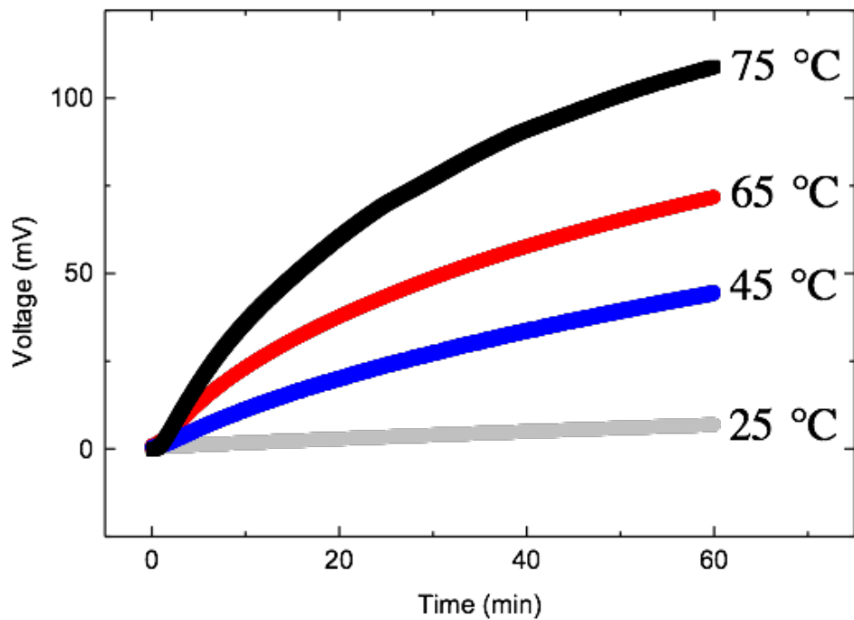
Figure S4. Thermal charging the same type EDLC for one hour at different temperatures after one electrical charge/discharge cycle (10mA charging/discharging rate). It clearly shows that the thermal charging speed increases as the temperature gradually increases from 25 °C to 75 °C.
