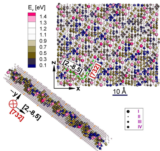
Fig. 9 Structure of the first minimum energy state of the \Sigma 11 GB viewed along the y and [732] directions. The view along the [732] direction is tilted so that it constitutes an orthographic projection of the view along the y direction. Atoms are sized according to the atom groups shown in Fig. 6b and colored according to vacancy formation energy
