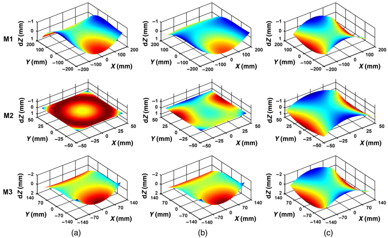
Fig. 6 Comparing mirror aspheric departure shapes: (a) conventional rotational aspheres design, (b) XY polynomial freeform design, and (c) NURBS freeform design.
