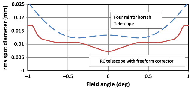
Fig. 11 rms spot diameters over the field of view.
