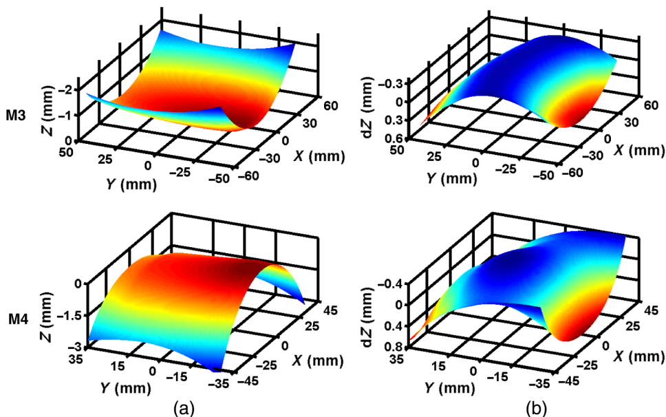
Fig. 10 Freeform corrector mirrors: (a) physical shapes and (b) aspheric departures from best-fit sphere.
