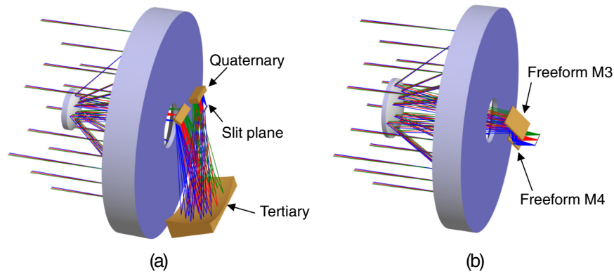
Fig. 9 Telescopes for spectrometer: (a) four-mirror Korsch design and (b) RC telescope with a two-mirror freeform corrector.
