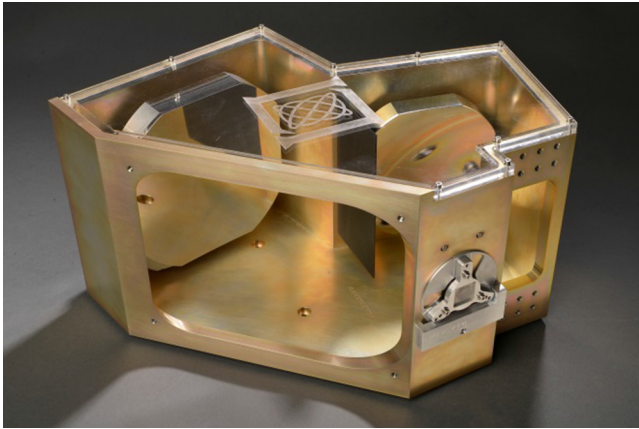
Fig. 8 Freeform demonstration telescope.
