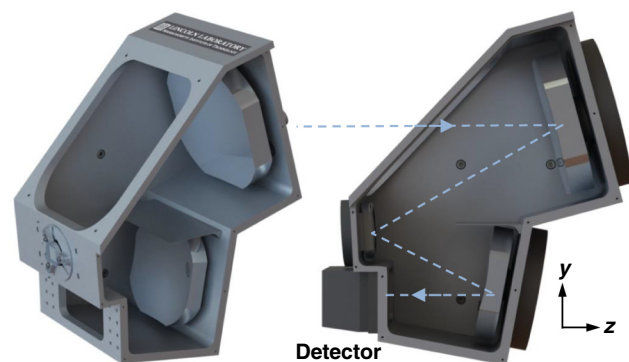
Fig. 7 Optomechanical design of the freeform demonstration telescope.
