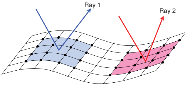
Fig. 1 Rays reflecting from third-degree NURBS surface.
