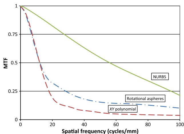
Fig. 5 MTF comparison between designs.
