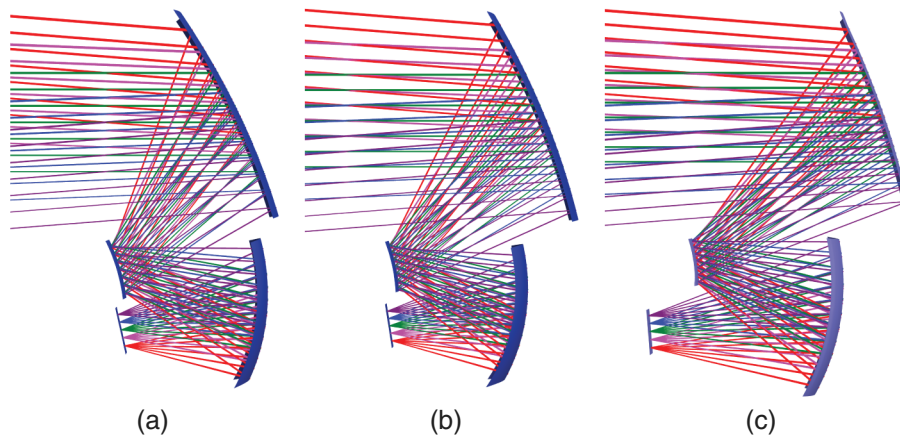
Fig. 3 Three-mirror anastigmat f/2 designs: (a) conventional rotational aspheres design, (b) XY polynomial freeform design, and (c) NURBS freeform design.
