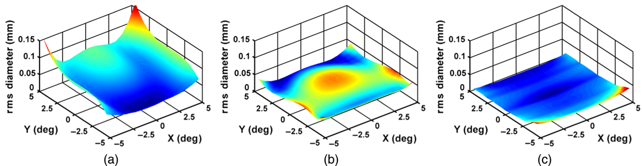
Fig. 4 Field map of rms spot sizes for f/2 three-mirror anastigmat designs: (a) conventional rotational aspheres design, (b) XY polynomial freeform design, and (c) NURBS freeform design.
