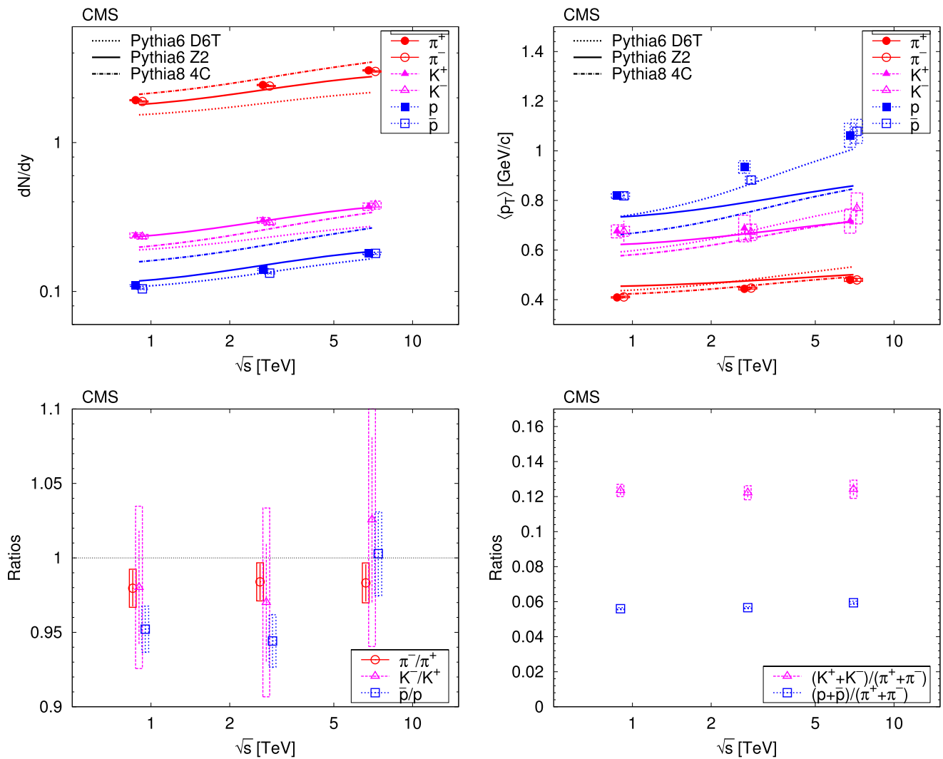
Fig. 17 Center-of-mass energy dependence of dN/dy , average transverse momentum ( p_T ), and ratios of particle yields. Error bars indicate the uncorrelated combined uncertainties, while boxes show the uncorrelated systematic uncertainties. For dN/dy ( \langle p_T \rangle ) the fully correlated
