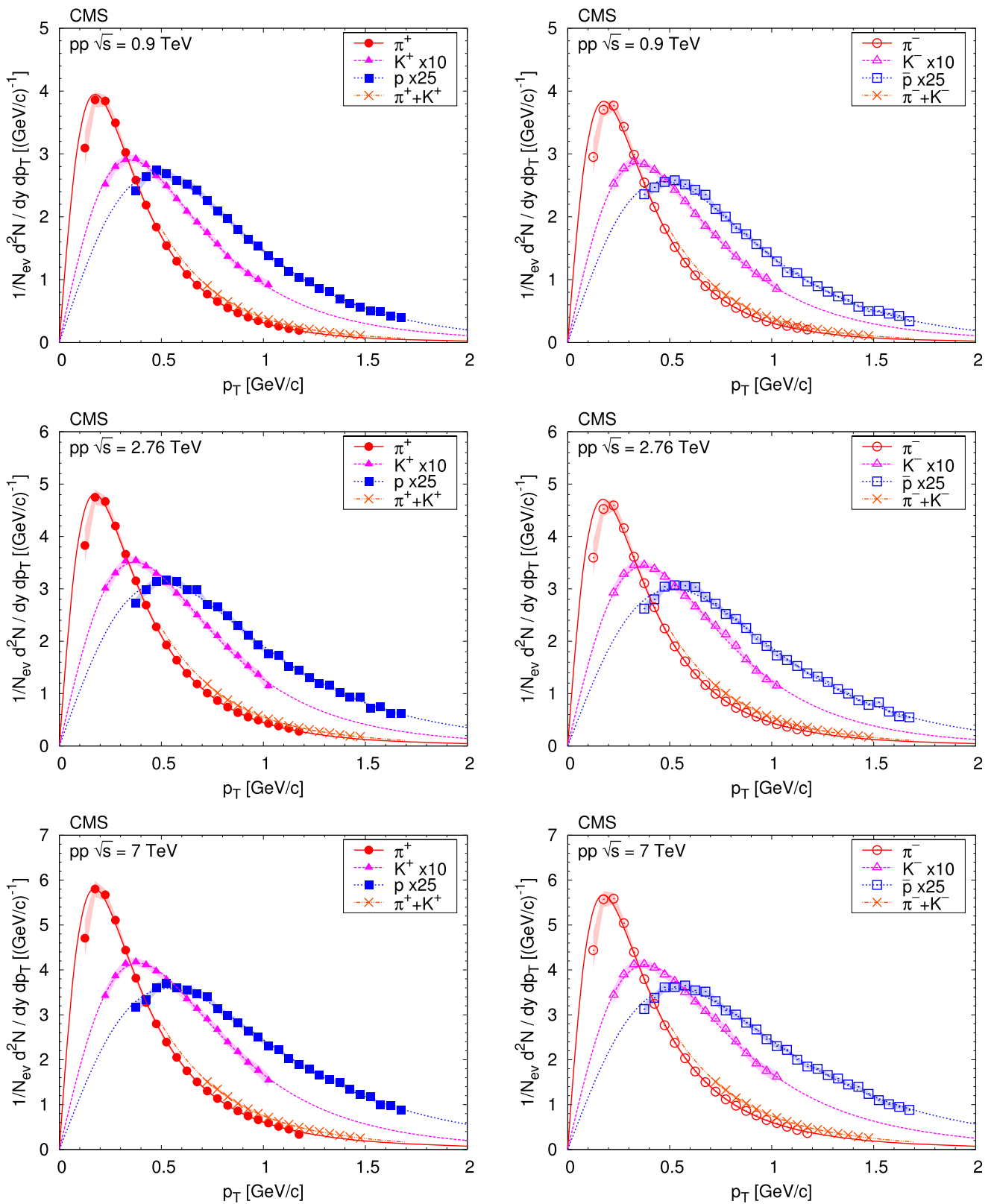
Fig. 9 Transverse momentum distributions of identified charged hadrons (pions, kaons, protons) in the range |y| < 1 , for positive ( left ) and negative ( right ) particles, at \sqrt{s} = 0.9, 2.76 , and 7 TeV (from top to bottom). Kaon and proton distributions are scaled as shown in
