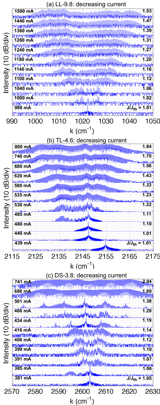
FIG. 4. Spectra of the three uncoated QCLs (a) LL-9.8, (b) TL-4.6, and (c) DS-3.8 as the current is decremented, starting from the current reached at the end of the upward current ramp shown in Fig. 3.
