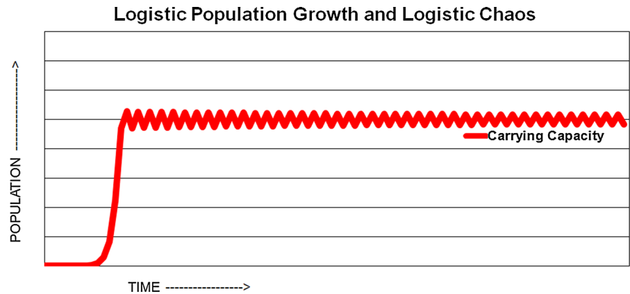
Fig. 3 Logistic growth for chaos parameter = 2
