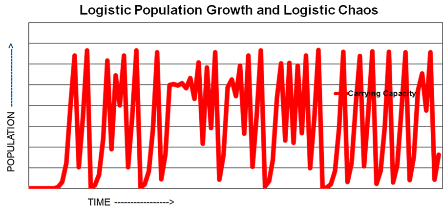
Fig. 5 Logistic growth for chaos parameter = 2.9
