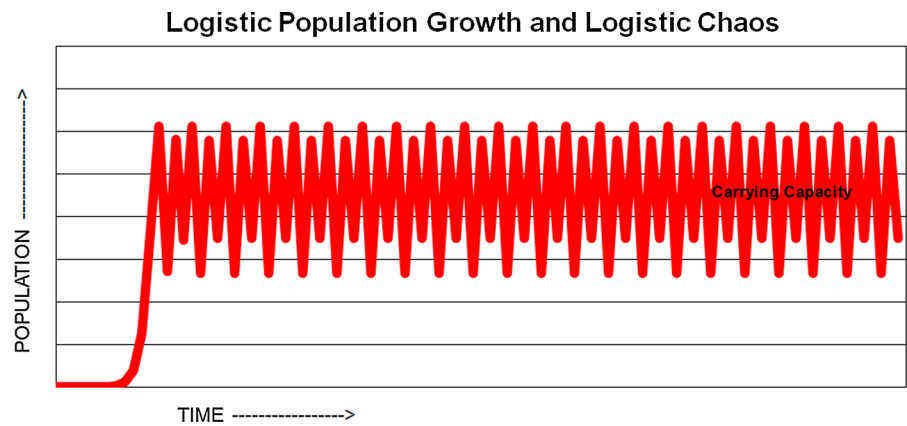
Fig. 4 Logistic growth for chaos parameter = 2.5
