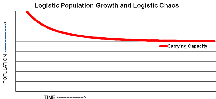
Fig. 1 Logistic solution for population approaching steady state from above
