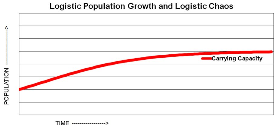
Fig. 2 Logistic solution for population approaching steady state from below
