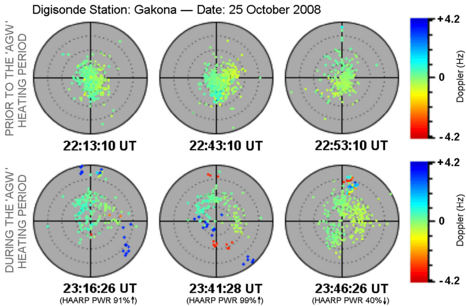
Fig. 5 A set of digisonde skymap data recorded on 25 October 2008, showing a few individual snapshots of the F-region ionosphere prior to the HAARP-AGW experiment ( top row ) as well as those during the HAARP-AGW heating period ( bottom row )
