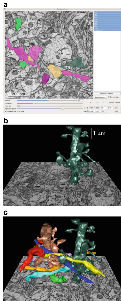
Fig. 4 Reconstruction from 2D contours. a Input to VolRoverN is a set of 2D polygonal traces, or contours, derived from EM images. b Software embedded in VolRoverN called ContourTiler fits a triangulated surface to each set of contours to produce a 3D surface model. c Multiple components are combined using ForestTiler such that they are free of intersections
