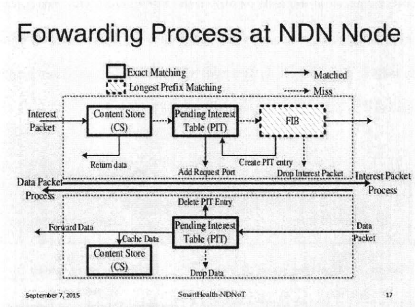
Figure 2-2 NDN Forwarding Pipeline [39]
