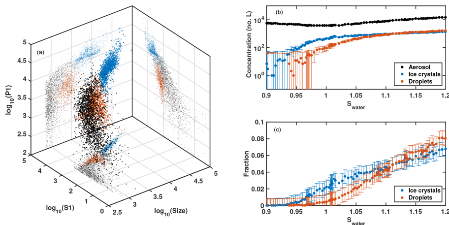
Figure 7. Application of three-class supervised ML on an example activation experiment where the chamber RH is increased. (a) Aerosol particles (black), ice crystals (blue), and water droplets (red) shown in \log_{10}(P_1) vs. \log_{10}(S_1) vs. \log_{10}(\text{Size}) parameter space with classification accuracy of 99 %. 2-D projections of the data are shown at axes limits with smaller markers. (b) Concentration of aerosol particles, ice crystals, and water droplets as a function of chamber RH. Error bars represent classification uncertainty. (c) Fraction of particles activated as ice crystals and water droplets as a function of chamber RH. Error bars represent classification uncertainty. Data points with lower error bars below zero indicate that the values are statistically indistinguishable from zero.
