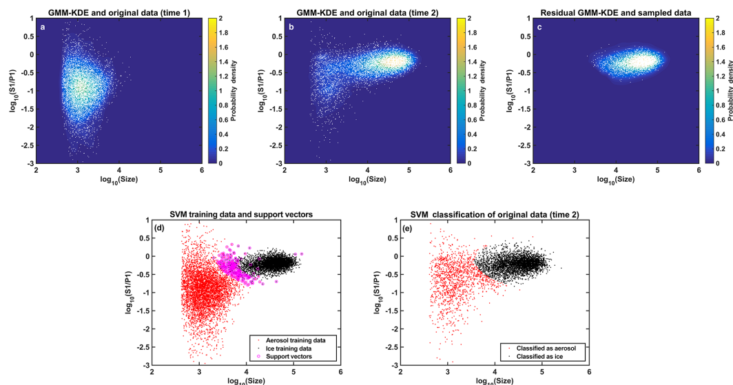
Figure 6. Illustration of the supervised ML procedure used to classify OPC data in \log_{10}(S_1/P_1) vs. \log_{10}(\text{size}) parameter space. The units of Size, S_1 , and P_1 are all intensity counts. (a) Data and GMM-KDE for an aerosol only time interval (time 1). (b) Data and GMM-KDE for an aerosol + ice time interval (time 2). (c) Residual GMM-KDE (time 2 minus time 1) and data from weighted sampling informed by the deconvolved PDF. (d) Aerosol data, ice data, and support vectors for SVM training. Cross-validated classification accuracy is 99 % in this example. (e) Data from time 2 classified by SVM as aerosol and ice. See Sect. 3.2 for details.
