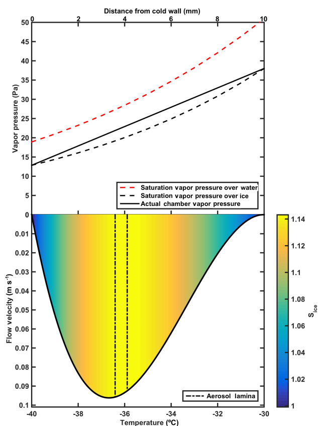
Figure 1. Representation of idealized chamber thermodynamic and flow conditions with a chamber width of 1 cm. The chamber cold wall (left) temperature is -40^{\circ}\text{C} and chamber warm wall (right) is -30^{\circ}\text{C} . The top half of the figure shows the saturation vapor pressures over ice (black dashed line), over water (red dashed line), and chamber vapor pressure (solid black line) for 10\text{ L min}^{-1} sheath + 1\text{ L min}^{-1} sample flow. Note the chamber is supersaturated everywhere with respect to ice but subsaturated with respect to water. The bottom half of the figure shows the flow velocity profile with the aerosol lamina given by the black dashed dotted lines. The colors show the horizontal variation in the ice saturation ratio across the width of the chamber. The asymmetry in the flow profile is a result of the buoyant displacement of the flow towards the cold wall.
