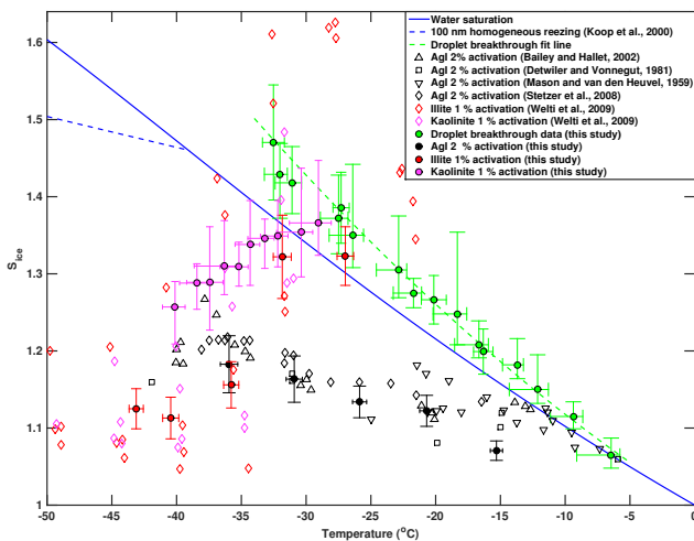
Figure 10. Experimental heterogeneous ice nucleation results and comparison to literature with polydisperse NX illite, AgI, and 500 nm kaolinite particles. AS droplet breakthrough data and corresponding (quadratic) fit line are shown in green. Error bars represent uncertainty in lamina temperature and supersaturation conditions. The homogeneous freezing line for solution droplets for J = 10^{11}\text{ cm}^{-3}\text{ s}^{-1} from Koop et al. (2000) is also shown for reference.
