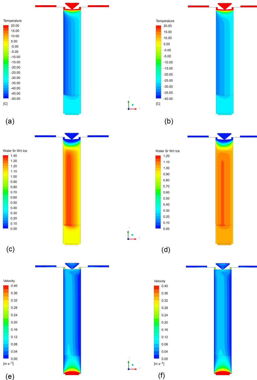
Figure 12. Fluent simulation results for two sets of chamber conditions in a cross-sectional view. The left column shows results for nominal lamina temperature of -40^{\circ}\text{C} and lamina S_{\text{ice}} at 1.3. (a) Temperature ( ^{\circ}\text{C} ), (c) S_{\text{ice}} , and (e) flow velocity ( \text{m s}^{-1} ). The right column shows results for nominal lamina temperature of -30^{\circ}\text{C} and lamina S_{\text{ice}} at 1.1. (b) Temperature ( ^{\circ}\text{C} ), (d) S_{\text{ice}} , and (f) flow velocity ( \text{m s}^{-1} ).
