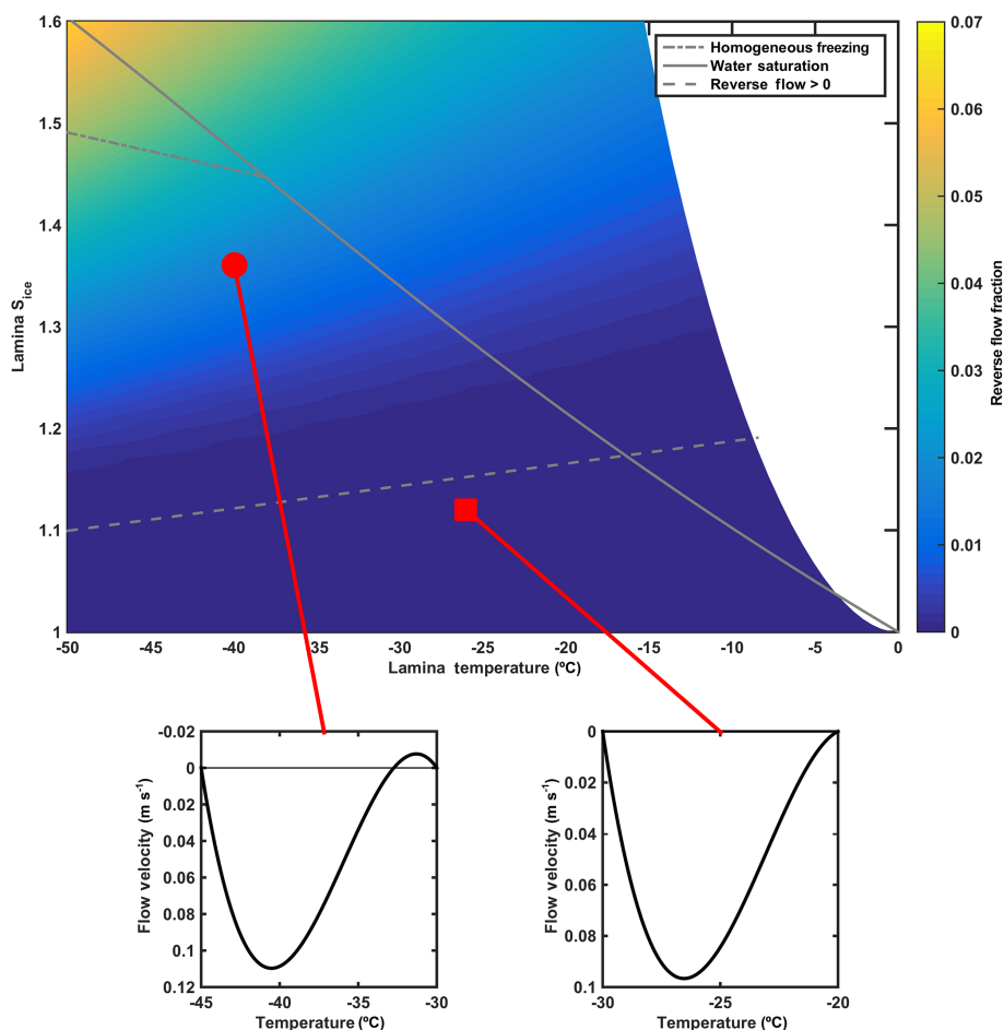
Figure 5. Phase diagram of ice saturation ratio vs. temperature showing the thermodynamic conditions accessible by CFDC chambers. The color scale shows the ratio of (upward) reverse flow to (downward) normal flow in the chamber (with 10 standard \text{L min}^{-1} sheath flow, 1 standard \text{L min}^{-1} sample flow, and 1000 hPa chamber pressure) assuming a negligibly thick ice layer predicted by Rogers (1988) with the dashed grey line marking the boundary between zero and nonzero flow reversal (see Sect. 3.1 for details). The solid grey line is water saturation, and the grey dashed dotted line shows the onset of homogeneous freezing of solution droplets for J = 10^{11} \text{ cm}^{-3} \text{ s}^{-1} from Koop et al. (2000). Two flow profiles are shown as insets: the coldest temperature in each corresponds to the cold wall temperature and the warmest to the warm wall temperature. Flow reversal occurs along the warm wall in one case (left, red circle) and not in the other (right, red square).
