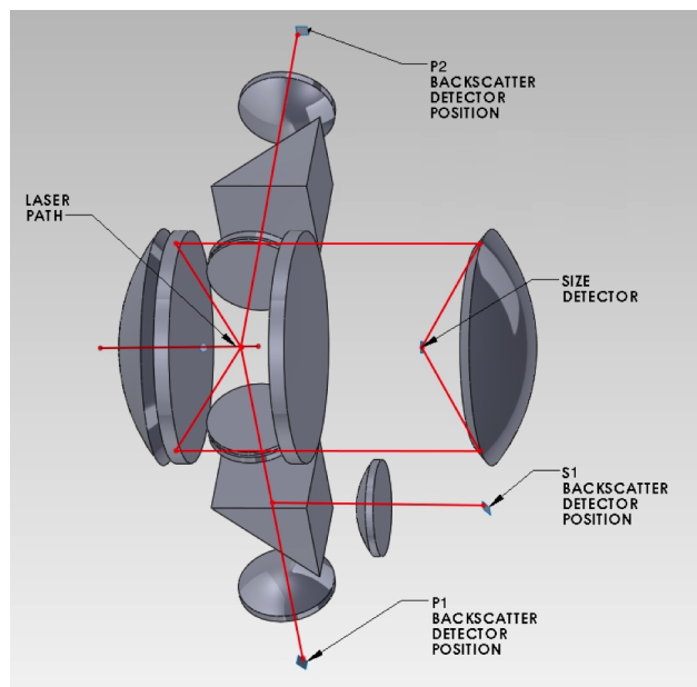
Figure 4. Schematic optical setup of the SPIN OPC. The laser light is shown entering the sampling region, with side scatter rays traveling to the sizing detector, and the backscatter rays traveling to the depolarization detectors (see Sect. 2.2 for details).
