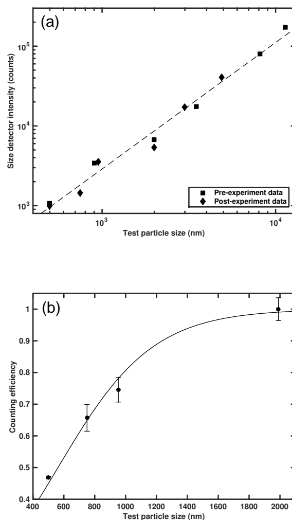
Figure 8. Particle sizing and transmission efficiency of the SPIN detector. (a) Detector intensity counts vs. test particle size before and after the freezing experiments in this study. The dashed line shows the power law fit to the data. (b) Size-dependent counting efficiency of AS particles with sigmoid fit. Error bars show measurement uncertainty.
