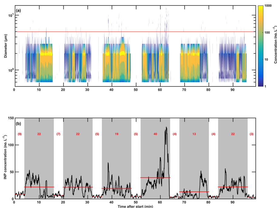
Figure 11. Example field measurement at \sim -30^\circ\text{C} and S_{\text{liq}} = 1.05 (reported lamina temperature of -30.7^\circ\text{C} \pm 0.2^\circ\text{C} and lamina S_{\text{liq}} of 1.05 \pm 0.01 over the measurement period). (a) The OPC size histogram time series for this measurement. The red horizontal line shows the 5\ \mu\text{m} size threshold for ice. (b) INP concentration time series using the 5\ \mu\text{m} size threshold. Shaded areas show measurement periods and unshaded areas show filter periods. Solid red horizontal lines show average INP concentrations from measurement periods (with the value specified above in parentheses). Dashed red horizontal lines show average frost concentrations during filter periods (with the value specified above in parentheses).
