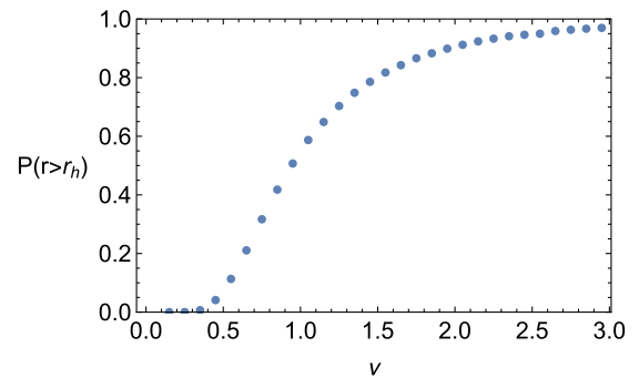
FIG. 4. Fraction of the probability density, in the ground state, which has support for r > r_h \equiv \sqrt{-\theta/\mu} .
