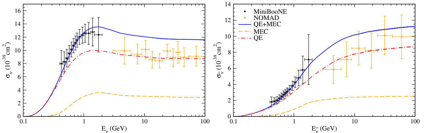
FIG. 14. MiniBooNE CCQE \nu_\mu - ^{12}\text{C} ( \bar{\nu}_\mu - ^{12}\text{C} ) total cross section per nucleon as a function of the neutrino energy. The left panel corresponds to neutrino cross sections and the right one to antineutrino reactions. Data are from [1,2].
