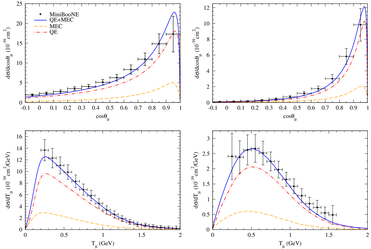
FIG. 13. MiniBooNE flux-averaged CCQE \nu_\mu - ^{12}\text{C} ( \bar{\nu}_\mu - ^{12}\text{C} ) differential cross section per nucleon as a function of the muon scattering angle (top panels) and of the muon kinetic energy (bottom panels). The left panels correspond to neutrino cross sections and the right ones to antineutrino reactions. Data are from [1,2].
