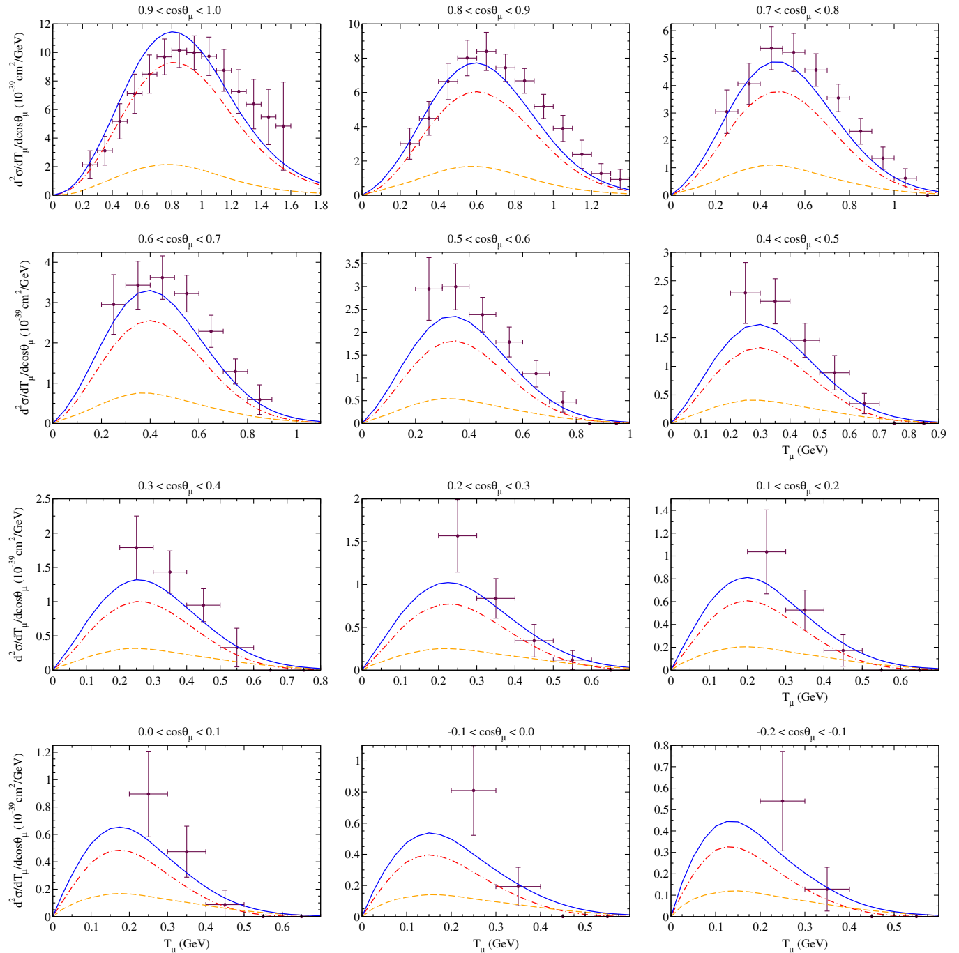
FIG. 8. As for Fig. 6, but now for the \bar{\nu}_\mu CCQE process on ^{12}\text{C} . Data are from [2].
