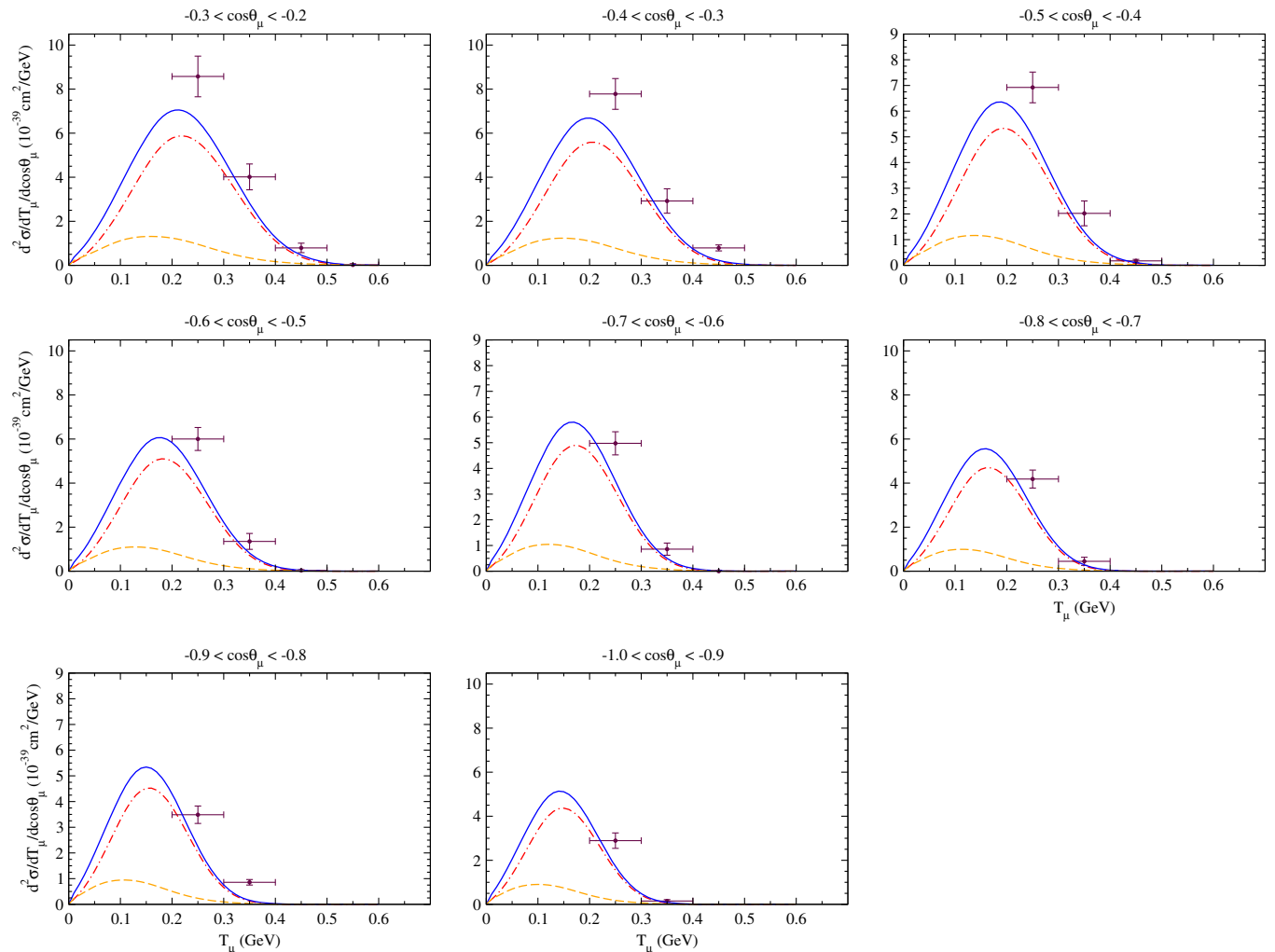
FIG. 7. As for Fig. 6 but considering more backward kinematics. Data are from [1].
