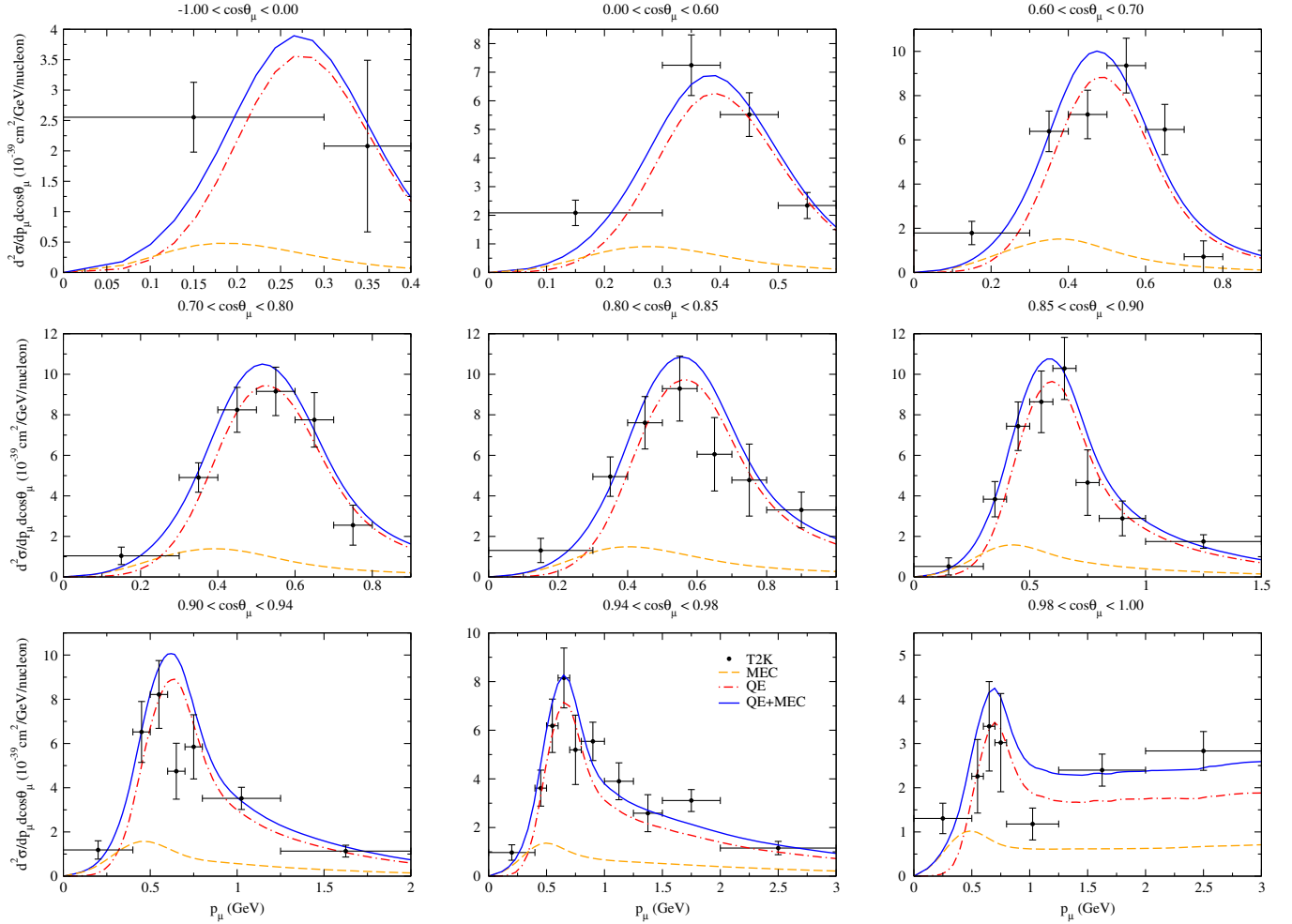
FIG. 17. T2K flux-folded double differential cross section per target nucleon for the \nu_\mu CCQE process on ^{12}\text{C} displayed versus the \mu^- momentum p_\mu for various bins of \cos\theta_\mu obtained within the SuSAv2+MEC approach. QE and 2p-2h MEC results are also shown separately. Data are from [6].
