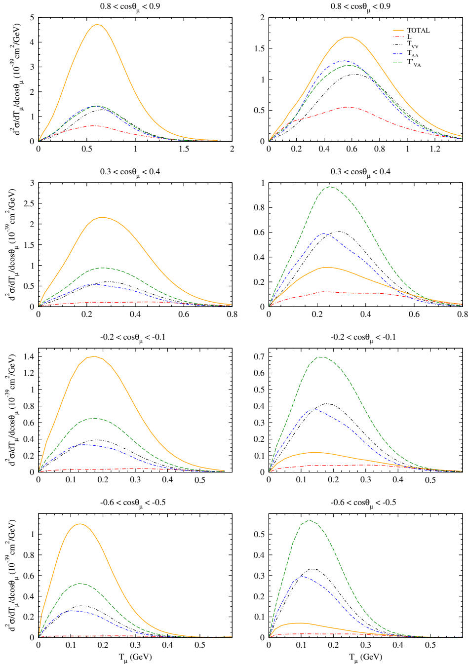
FIG. 10. Comparison of the different 2p-2h MEC channels for the \nu_\mu (left panels) and \bar{\nu}_\mu (right panels) MiniBooNE double differential cross section.
