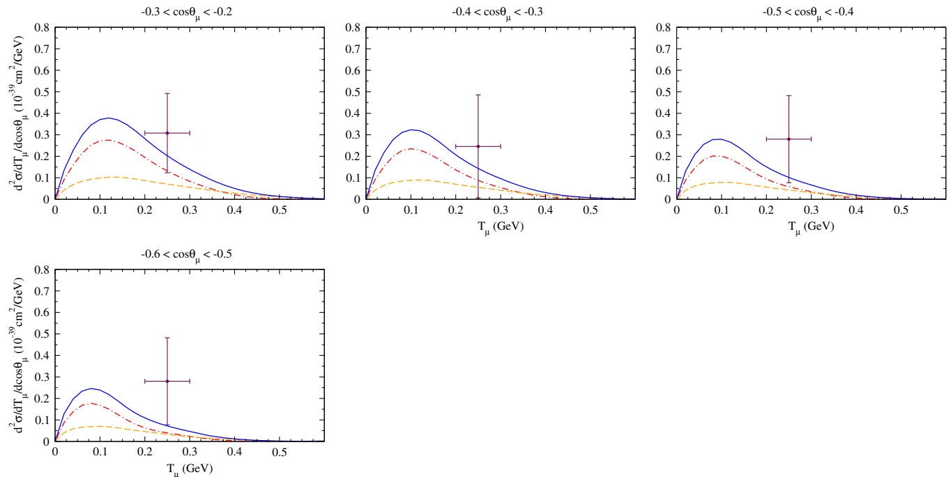
FIG. 9. As for Fig. 8, but considering more backward kinematics. Data are from [2].
