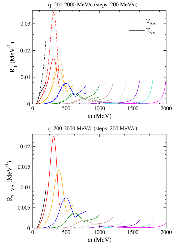
FIG. 3. Comparison between 2p-2h MEC axial-axial transverse ( T_{AA} ) response functions and the vector-vector ones ( T_{VV} ) versus \omega (top panel). The transverse vector-axial interference term ( T'_{VA} ) is also shown (bottom panel). The curves are displayed from left to right in steps of q = 200 \text{ MeV}/c .
