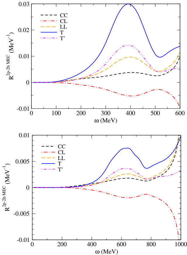
FIG. 1. Comparison between 2p-2h MEC transverse ( T = T_{VV} + T_{AA} and T' = T'_{VA} ) response functions and the longitudinal ones ( CC , CL , and LL ) at q = 600 \text{ MeV}/c (top panel) and q = 1000 \text{ MeV}/c (bottom panel).
