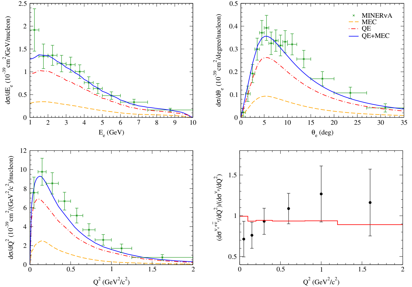
FIG. 16. MINERvA flux-integrated differential \nu_e CCQE-like cross section vs electron energy (top left) and electron angle (top right). The cross section vs Q^2_{QE} is shown in the bottom panel. Data are from [46].
