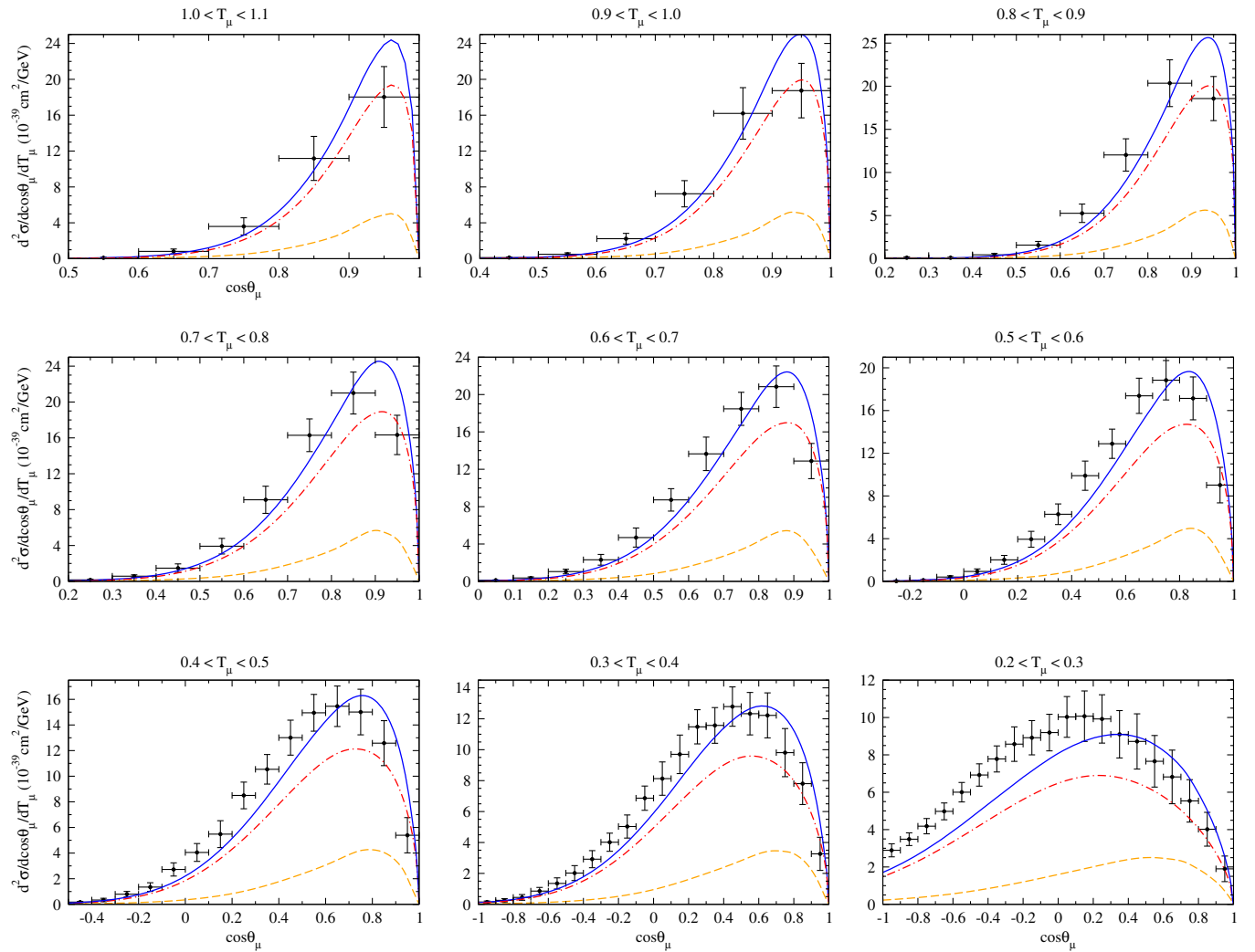
FIG. 11. MiniBoone flux-folded double differential cross section per target nucleon for the \nu_\mu CCQE process on ^{12}\text{C} displayed versus \cos\theta_\mu for various bins of T_\mu obtained within the SuSAv2 + MEC approach. QE and 2p-2h MEC results are also shown separately. Data are from [1].
