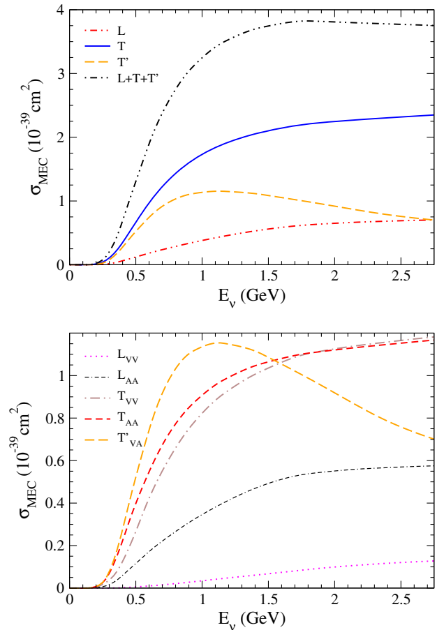
FIG. 2. Separation into components of the total 2p-2h MEC \nu_\mu cross section displayed versus neutrino energy E_\nu . The total longitudinal ( L ), transverse ( T ), and transverse interference ( T' ) contributions are shown (top panel) as well as the total 2p-2h MEC cross section ( L + T + T' ). Longitudinal and transverse channels are decomposed into vector and axial contributions (bottom panel).
