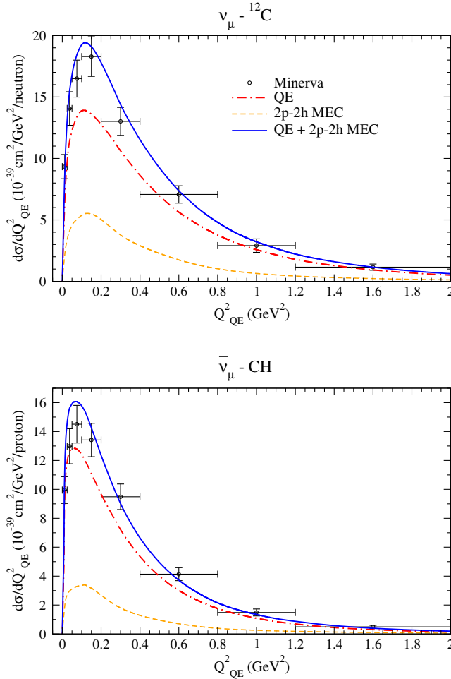
FIG. 15. Flux-folded \nu_\mu - {}^{12}\text{C} CCQE (upper panel) and \bar{\nu}_\mu - \text{CH} (lower panel) scattering cross section per target nucleon as a function of Q_{QE}^2 and evaluated in the SuSAv2 and SuSAv2 + MEC models. MINER \nu A data are from [44].
