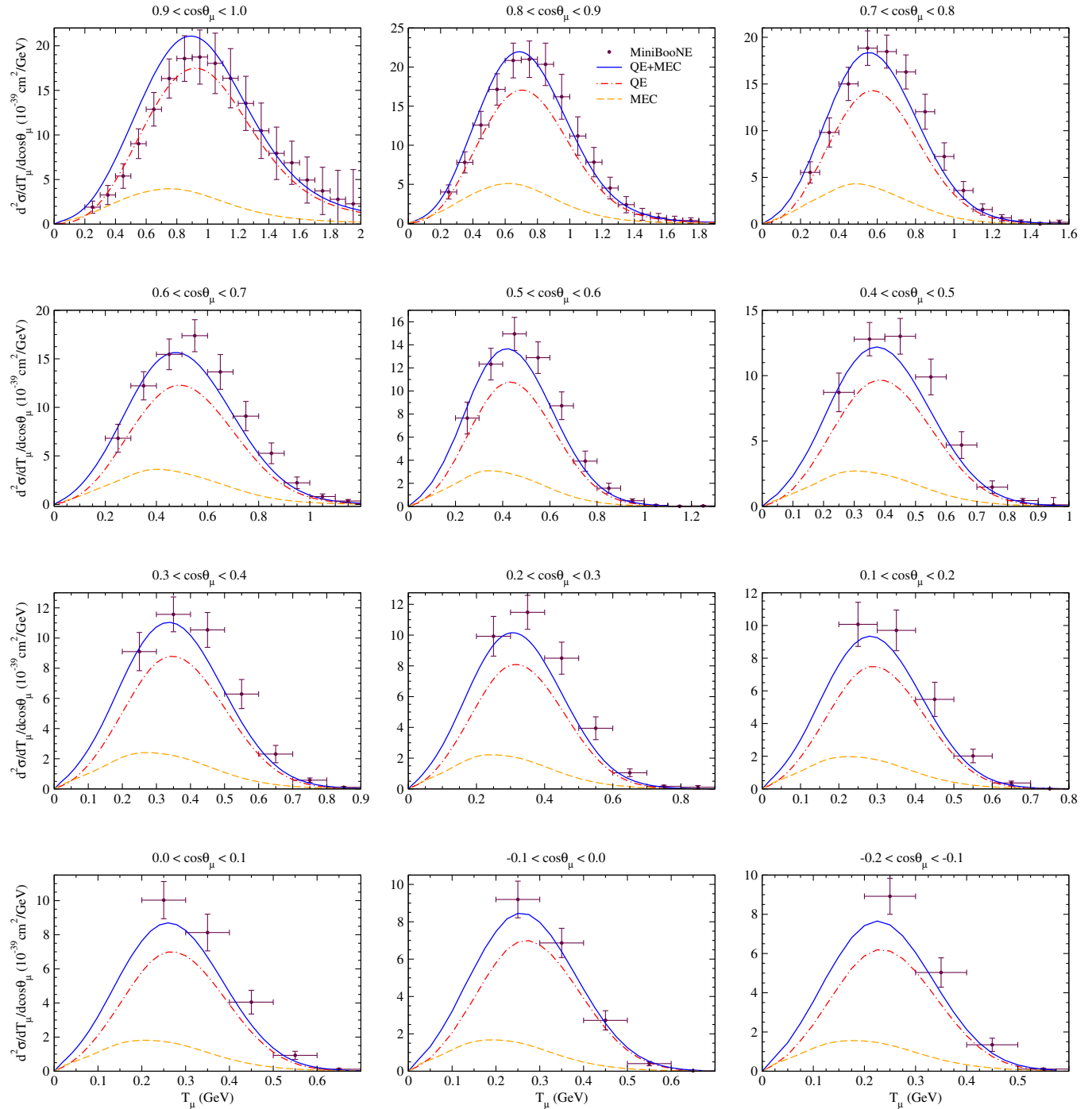
FIG. 6. MiniBooNE flux-folded double differential cross section per target nucleon for the \nu_\mu CCQE process on ^{12}\text{C} displayed versus the \mu^- kinetic energy T_\mu for various bins of \cos\theta_\mu obtained within the SuSAv2 + MEC approach. QE and 2p-2h MEC results are also shown separately. Data are from [1].
