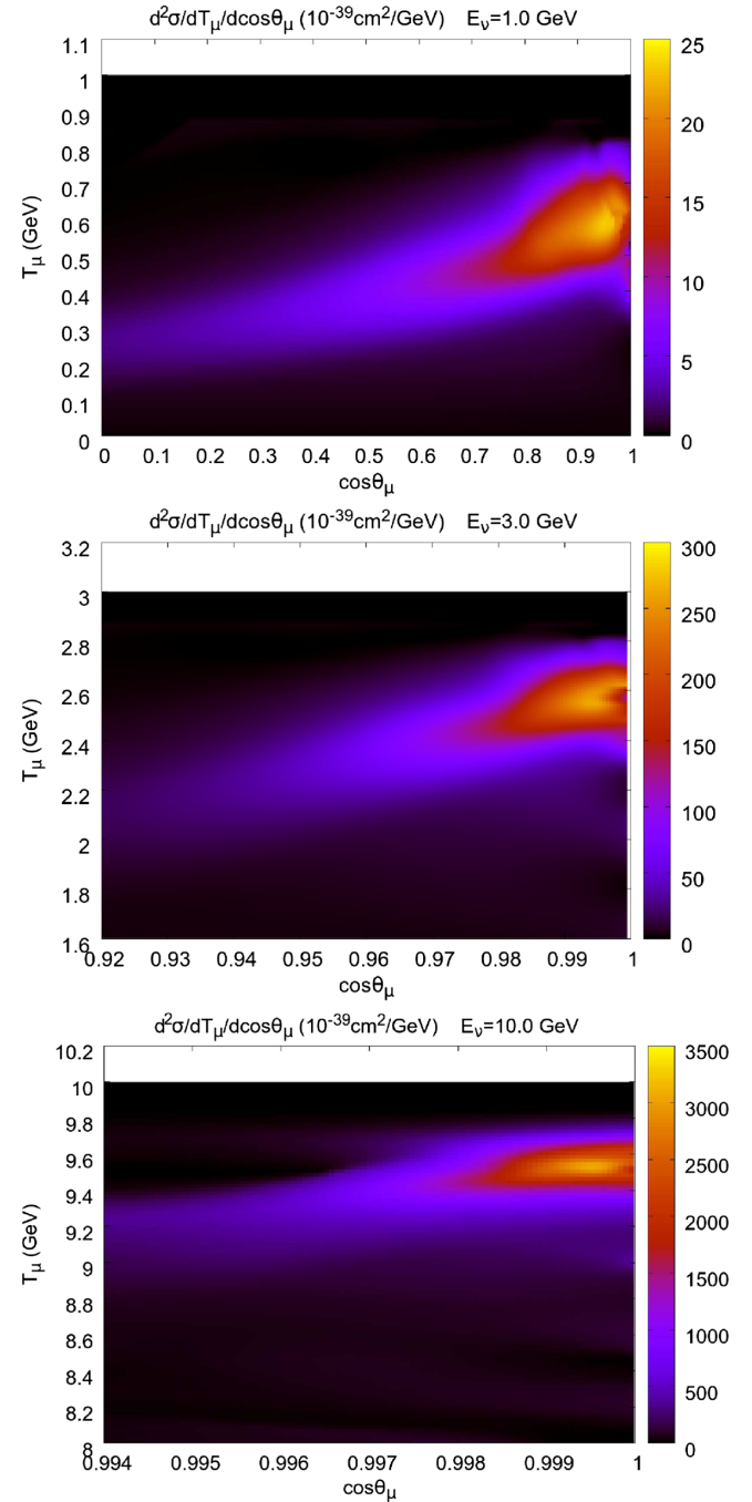
FIG. 5. The 2p-2h MEC density plots of the double-differential cross section per neutron of ^{12}\text{C} at three different neutrino energies E_\nu versus T_\mu and \cos\theta_\mu .
