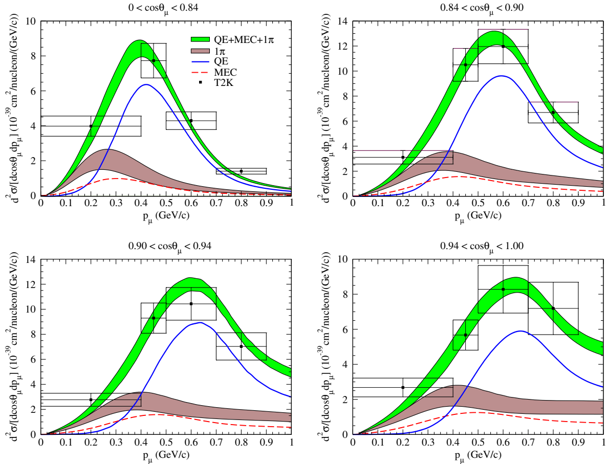
FIG. 18. The CC-inclusive T2K flux-folded \nu_\mu - {}^{12}\text{C} double-differential cross section per nucleon evaluated in the SuSAv2 + MEC model is displayed as a function of the muon momentum for different bins in the muon angle. The separate contributions of the QE, 1\pi , and 2p\text{-}2h MEC are displayed. The data are from [4].
