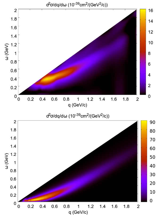
FIG. 4. The 2p-2h MEC (top panel) and QE (bottom panel) density plots of the double-differential cross section per neutron of ^{12}\text{C} versus \omega and q at E_\nu = 3 \text{ GeV} .
