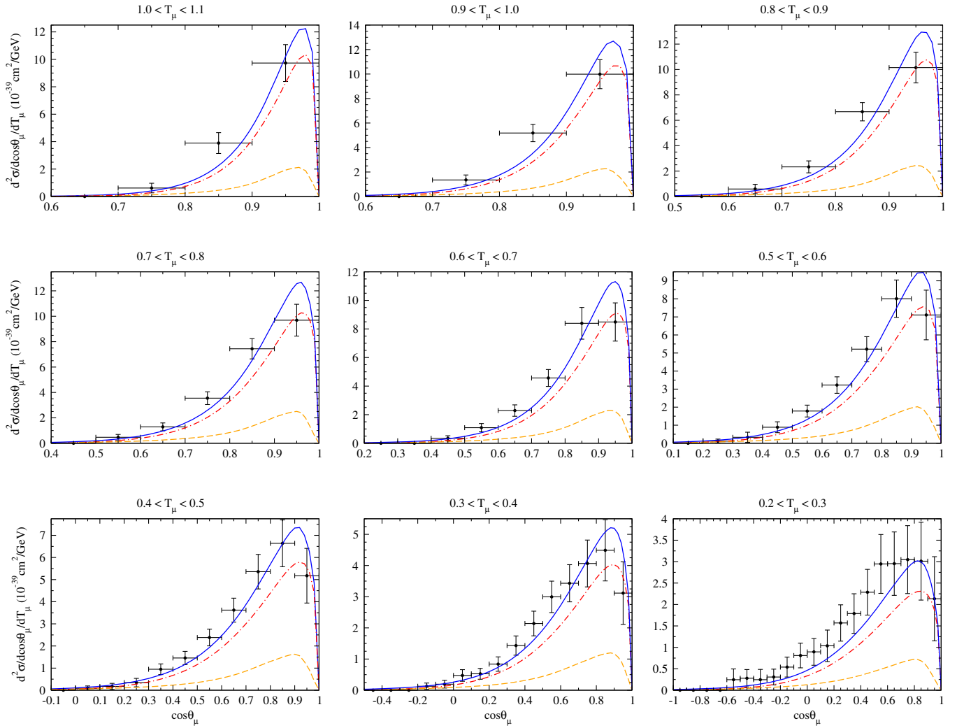
FIG. 12. As for Fig. 11, but now for the \bar{\nu}_\mu CCQE process on ^{12}\text{C} . Data are from [2].
