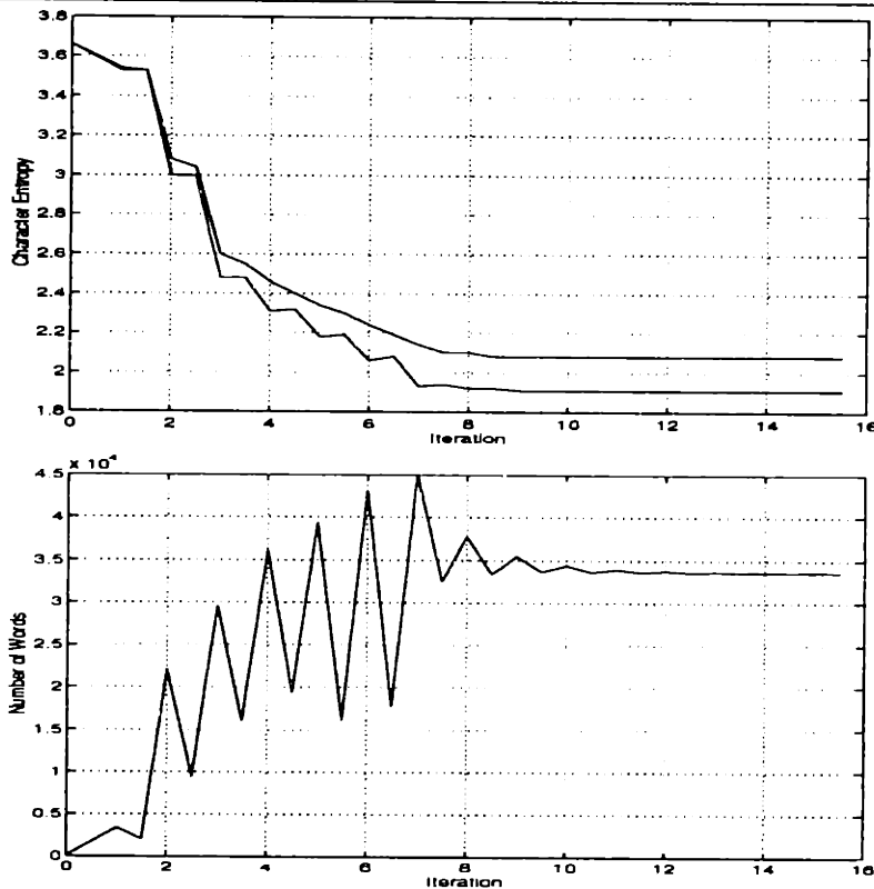
Figure 6.2: Learning curves for the algorithm on the Brown corpus. The top graph plots model performance. The upper line is the compression rate—the complete description length divided by length of the input. The lower line discounts the cost of parameters: it is the cross-entropy rate of the model with the input. The bottom graph plots the number of words in the lexicon.
