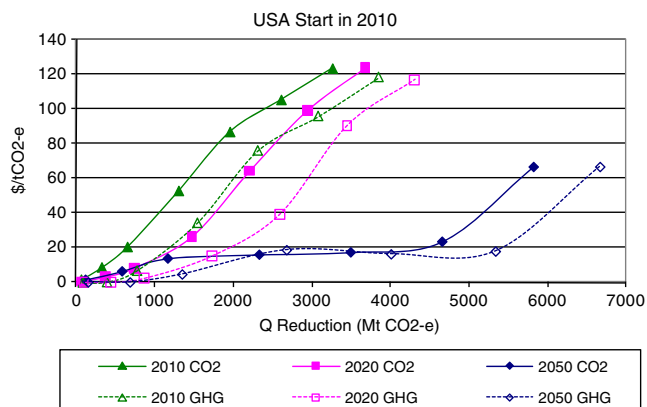
Fig. 5 MACs in 2010, 2020, and 2050 when the policy started in 2010 applies to just CO 2 and when it applies to all GHGs
