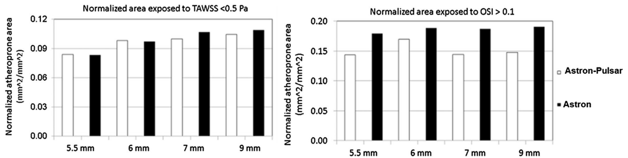
FIGURE 7. Normalized surface area exposed to time-averaged wall shear stress (TAWSS) of less than 0.5 Pa (left) and oscillatory shear index (OSI) of more than 0.1 (right). Oversizing leads to larger areas being exposed to low TAWSS and more prominent atheroprone conditions at the arterial wall, which is more noticeable for the cases with the stiffer Astron stent. On the other hand, while the deployment of Astron noticeably rises the oscillatory characteristics of local blood flow, those features are not directly affected by stent oversizing.
