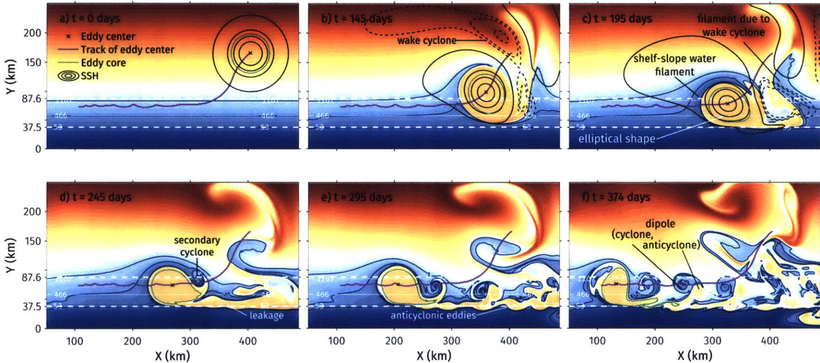
Figure 5.1: Snapshots of surface cross-shelf dye field. Bathymetric contours are in gray; dashed lines mark the shelf- and slope-break. The green contour identifies the core of the eddy (Section 3.2). Blue contours identify shelf-slope water parcels that started out at the marked isobaths. SSH is contoured in black; negative values are dashed. (a) Initially, each water parcel is tagged with its latitude. (b,c) As the eddy moves southwestward, it homogenizes the dye within itself. The eddy advects shelf-slope water across isobaths. (c,d) The eddy sheds fluid forming a warm along-shelf current. The advected shelf-slope water forms a filament (blue contours). (d,e) Cyclonic vortices containing shelf-slope water combine with anticyclonic fluid from the core of the eddy to form dipoles (Section 5.3.2). The process repeats, creating many dipoles that propagate away from the eddy. (f) The eddy water on the shelf at x \approx 430 km is an artifact caused by imperfect open boundary conditions.
