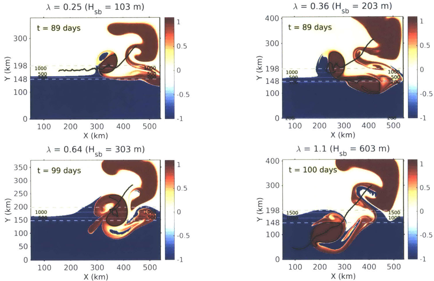
Figure B.1: Can the eddy cross the shelfbreak? Tracers tagging eddy water (red) and shelf-slope water (blue) illustrate different behaviour when varying \lambda = (shelfbreak depth)/(eddy depth scale). The black contour is the core of the eddy and the black line shows the track of the eddy's center.
