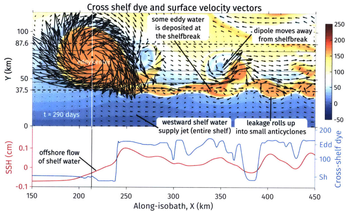
Figure 5.11: Above: horizontal velocity vectors and cross-shelf dye at the surface for a flat shelf. Below: along-shelf profiles of SSH and cross-shelf dye at the shelfbreak. There is offshore transport to the east of the eddy's center driven by eddy water leaking on to the shelf. All of the shelf to the east of the eddy is forced into motion to supply the offshore flow.
