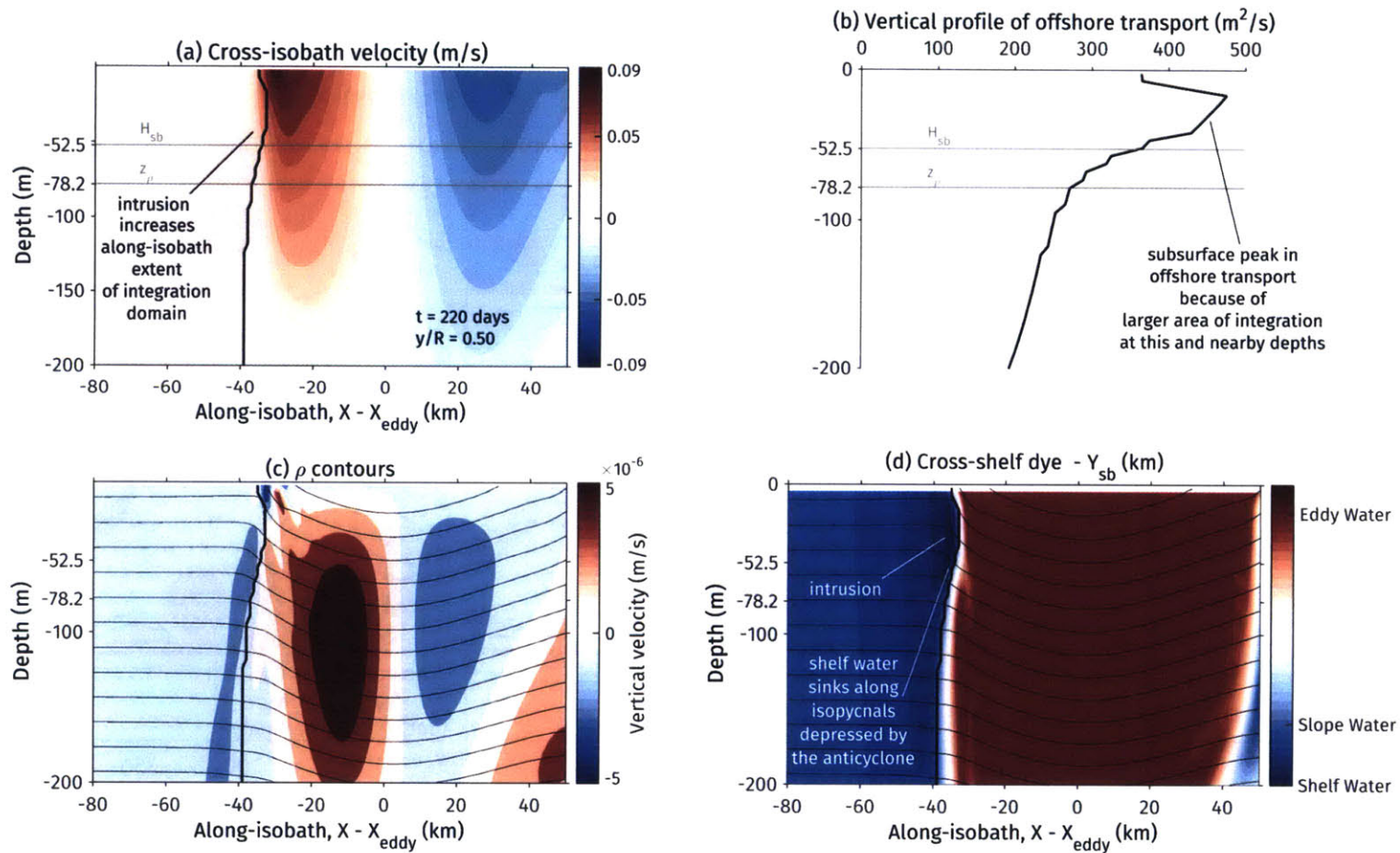
Figure 5.5: Instantaneous x - z sections. (a) Surface intensified cross-isobath velocity field and an intrusion into the eddy. The black contour is the boundary between eddy and shelf-slope water. Integrating the cross-shelf velocity field (a) within the black contour in x , results in (b), the vertical profile of offshore transport with a sub-surface peak. (c) Downward velocities experienced by slope water parcels as they sink along isopycnals to a depth z_p (Section 5.4). (d) The cross-shelf dye field, with overlaid \rho contours.
