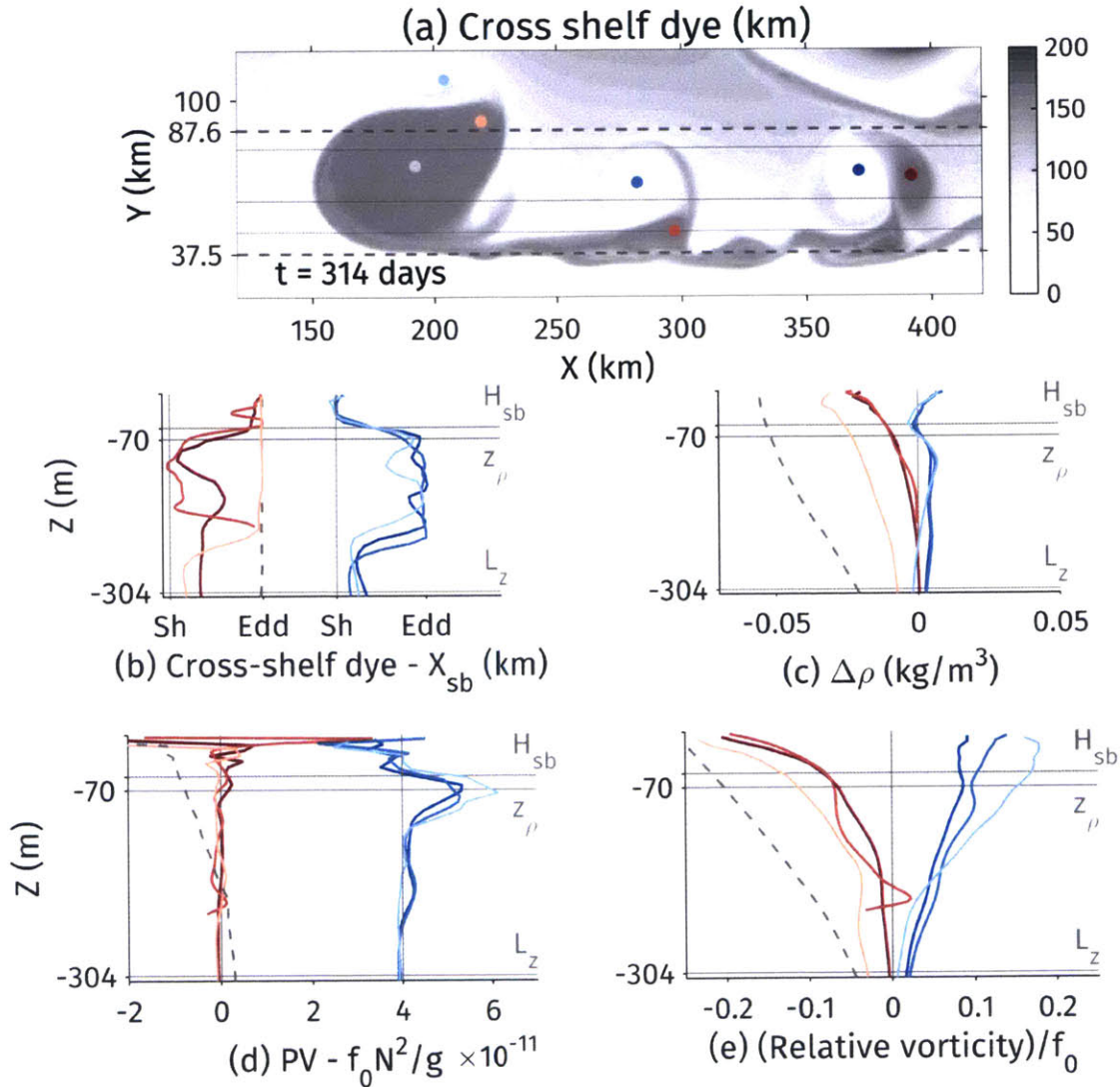
Figure 5.8: Vertical profiles at the dots illustrating the transition from an unstable wave to a dipole. The red profiles, on the left in each panel, are in locations with anticyclonic vorticity and vice versa . The gray dashed profile is at the eddy center providing a reference value for the fields. In (b) and (d), the lines on the right are displaced to make them easier to see. z_\rho is the predicted depth to which shelf water sinks, determined using the initial density field (see text). (b) Water masses as identified by cross-shelf dye: “Sh” is shelf-slope water and “Edd” is eddy water. (c) Profiles of the density anomaly. The anticyclones are always lighter than ambient water. The cyclones have the stacked structure explained in Section 5.4. (d) Profiles of PV anomaly: the cyclones have a subsurface peak corresponding to the interface between shelf and eddy water (see a). (e) Normalized relative vorticity whose sign doesn’t change with depth.
