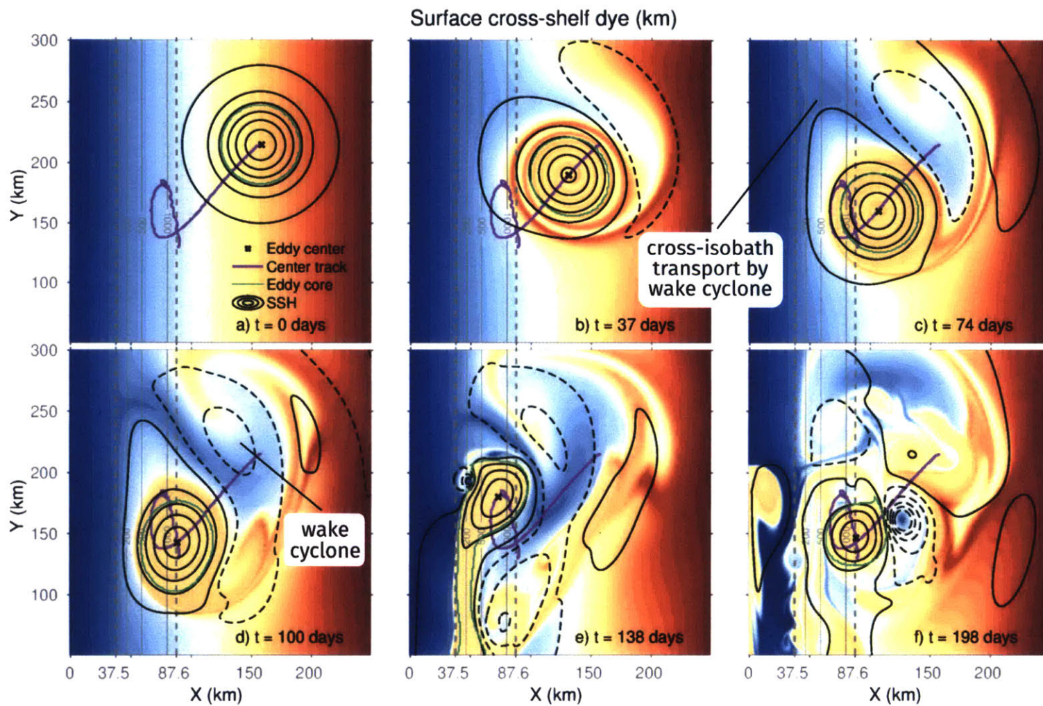
Figure 5.14: Surface contours for a simulation with a western coast. All contours are as in Figure 5.1.
