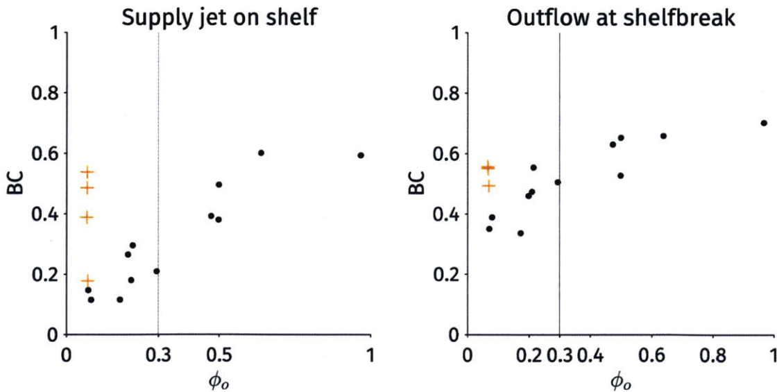
Figure 6.8: The shelf water supply jet is more baroclinic, as measured by BC , for larger values of non-dimensional parameter \phi_0 (Section 6.4.2). Orange points are simulations with bottom friction. They appear to be more baroclinic than the corresponding inviscid simulation, but a more detailed examination shows this to be false (Section 6.5).
