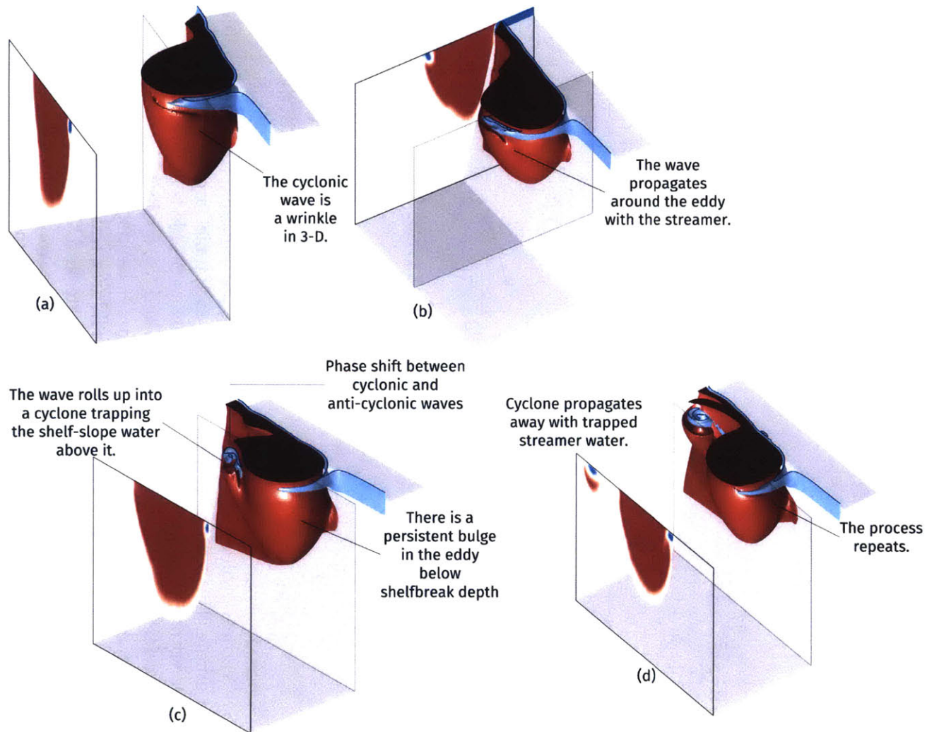
Figure 5.7: Smoothed dye fields at t = 215, 225, 235 and 255 days for the same run as in Figure 5.6.
