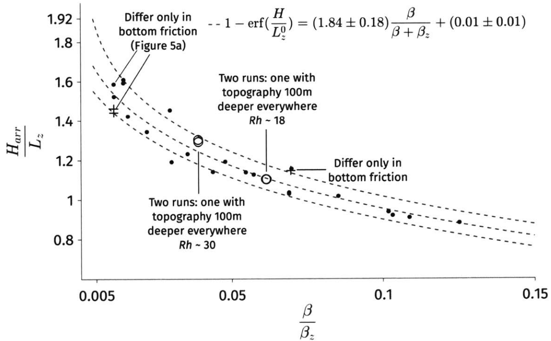
Figure 4.5: Flierl et al. (1983) based scaling for isobath H_{arr} at which the eddy's cross-isobath motion is appreciably reduced. The location is marked by a \times in Figures 4.2 and 4.7. All these simulations have (slope width) > (eddy width) and Rh \leq 40 . The black dots are model simulations with anticyclones, constant N^2 , no bottom friction and east-west isobaths. The '+' are simulations with bottom friction. Overlapping Os are two simulations that only differ in that one has topography 100 m deeper everywhere. There are two sets of such simulations.
