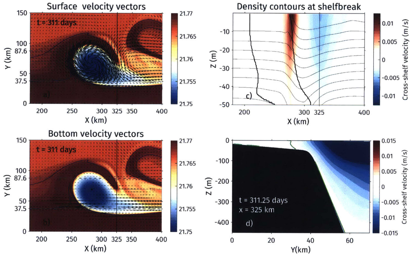
Figure 6.14: Snapshots for the same simulation as in Figure 6.13 with \varphi_o = 0.35 . (a,b) Surface density in colour with surface and bottom velocity vectors in (a) and (b) respectively. (c) Density contours and cross-shelf velocity at the shelfbreak. The black contour bounds water that has started inshore of the shelfbreak. (d) The vertical structure of cross-shelf velocity where eddy water moves onto the shelf. The thick green contour is v = 10^{-4} \text{ m s}^{-1} .
