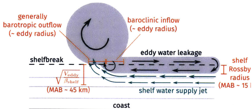
Figure 6.17: Shelf and slope flows forced by an eddy at the shelfbreak.
