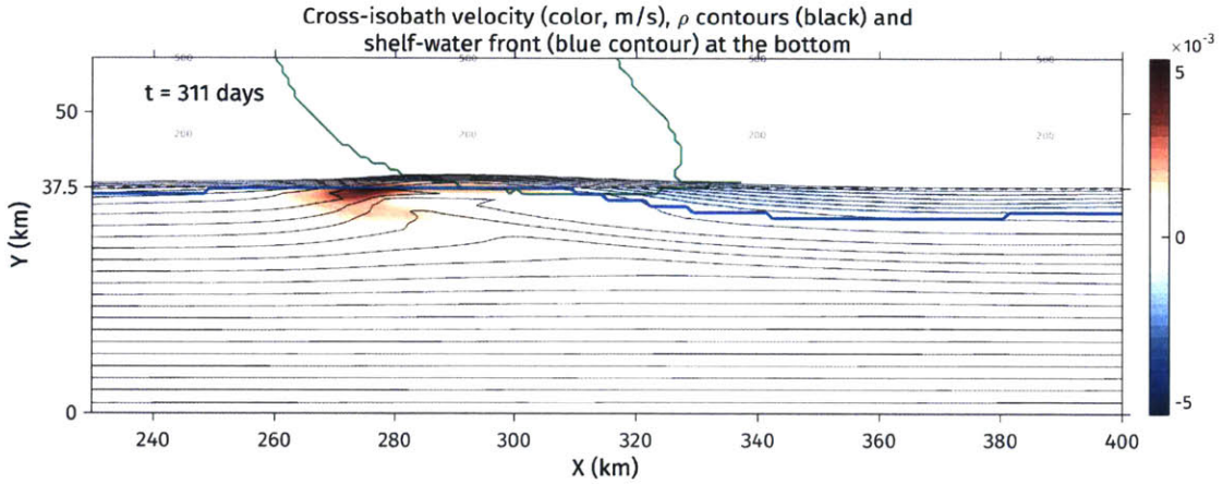
Figure 6.13: Instantaneous cross-isobath velocity in color and density contours at the bottom for an simulation with \varphi_o = 0.35 , i.e. the outflow is baroclinic. For clarity, only density contours over the shelf are shown. The cross-isobath flow creates a bottom density anomaly where the shelf water supply jet starts crossing isobaths. The along-isobath density gradient intensifies as the cross-isobath velocity increases at x = 270 km. It then modifies the vertical shear of the outflow.
