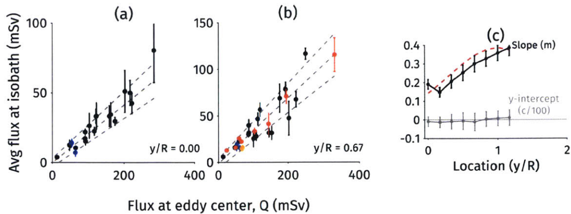
Figure 7.2: Parameterization for average flux at an isobath (flat shelf). Panels (a) and (b) are for particular isobaths: y/R = 0, 0.67 . Regression lines, diagnosed flux = mQ + c , are obtained using weighted least squares with weights being the inverse of the standard error. The black points are inviscid runs, blue points are viscid and red points are runs with a sloping shelf. Panel (c) shows the isobath dependence of the regression slope m and y -intercept c (Table 7.1). The red dashed curve is a Gaussian centered at the eddy center y/R = 1 .
