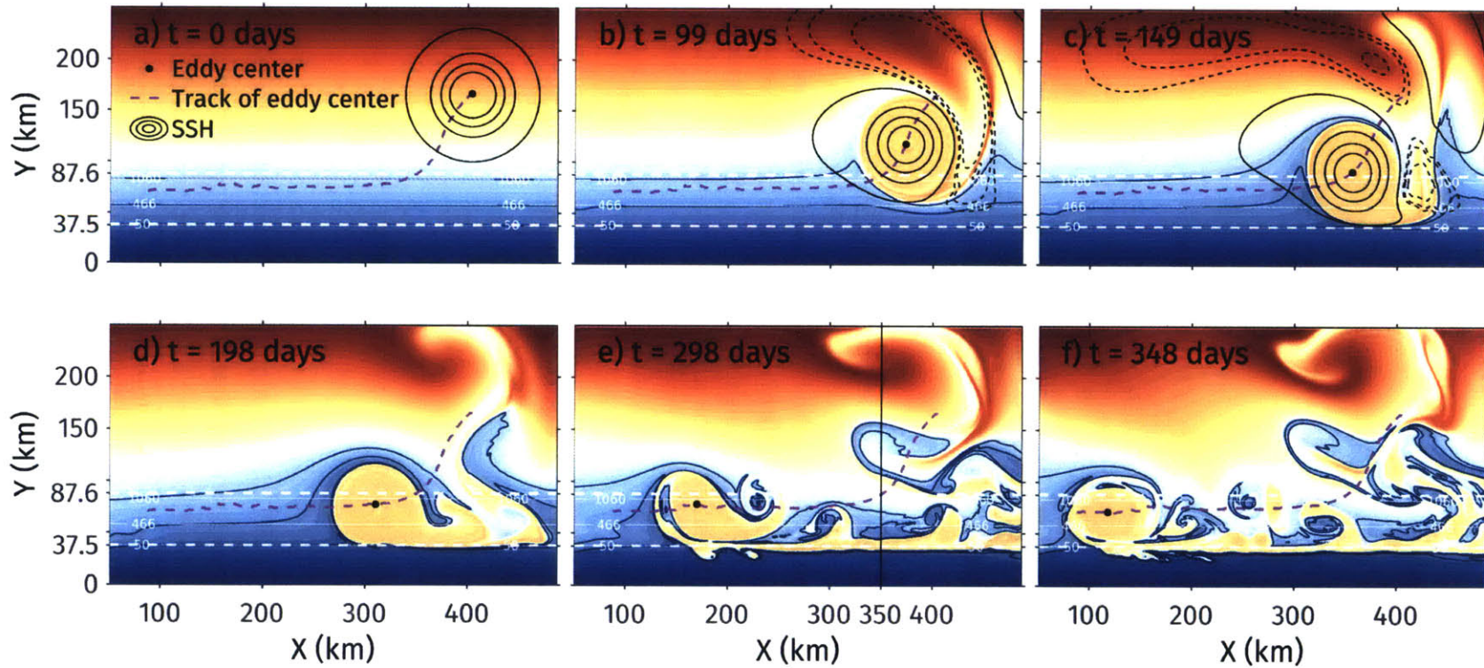
Figure 6.1: Snapshots of the cross-shelf dye field at the surface. Black contours are SSH, dashed contours indicate negative values. Thick white dashed lines mark the shelf- and slope-break. The evolution is just like that in Figure 5.1.
