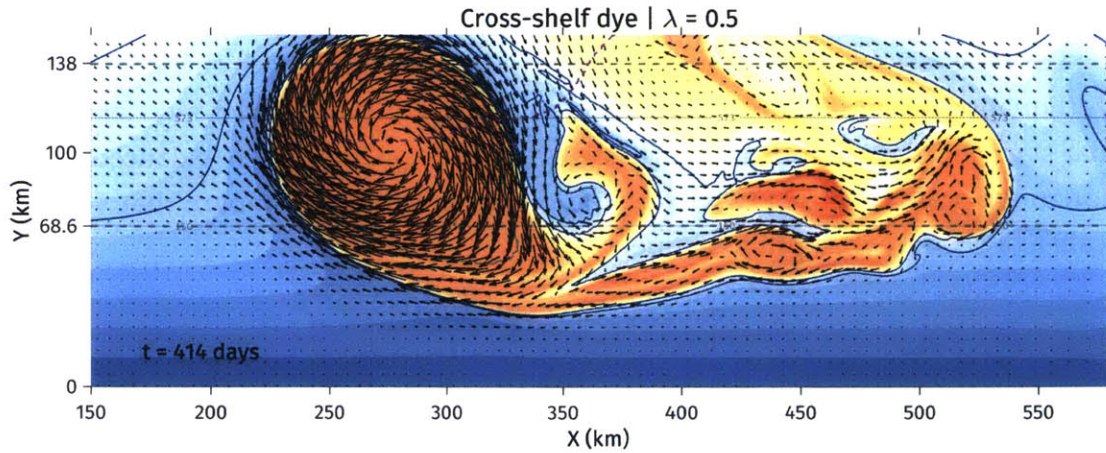
Figure 6.10: For \lambda = H_{sb}/L^2 = 0.5 , a substantial portion of the eddy's core crosses onto the shelf. The velocity vectors indicate that the eddy can now extract shelf water from a distance larger than L_\beta . Such simulations are excluded from Figure 6.11a. They are not excluded from Figure 6.11b where the width of the eddy leakage on shelf, as measured far downstream at x = 450 km for this simulation, correlates well with the shelf Rossby radius.
