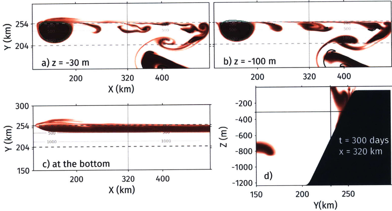
Figure 5.2: The along-shelf leakage, visualized using eddy dye, from a cyclone interacting with topography to the north is a lot weaker and less well-organized compared to that for an anticyclone (Figure 5.1). Panels (a,b,c) show x - y sections at depths z = -30 m, -100 m and along the bottom. There is a thin sheet of eddy fluid along the slope. Higher up in the water column, the flow is weak and less coherent than the leakage in Figure 5.1d,e.
