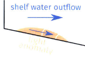
Figure 6.12: The kinematic bottom boundary condition imposed by the bottom slope on a cross-isobath flow forces the creation of density anomalies. These anomalies modify the vertical shear of the velocity field through the thermal wind equation.
