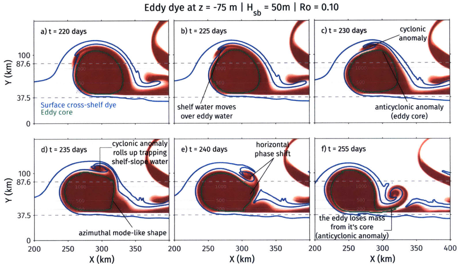
Figure 5.6: Growth of unstable waves shown by snapshots of eddy dye field interpolated to z = -75 \text{ m} . The eddy's vertical scale is 400 \text{ m} . Bathymetric contours are in gray, with dashed lines indicating the shelf- and slope-break. All other contours are of surface fields. The cross-shelf dye is in blue, showing offshore transport of slope water. The green contour defines an eddy core. (a,b) Slope water, advected by the near-surface velocity field, intrudes into the eddy (blue contour moves over red dye). (c,d,e) The cyclonic annulus fluid at depth starts to roll up into a cyclonic vortex trapping the shelf-slope water above it. (f) The eddy flings the cyclone away, which extracts some eddy water from the core (elongated green contour).
