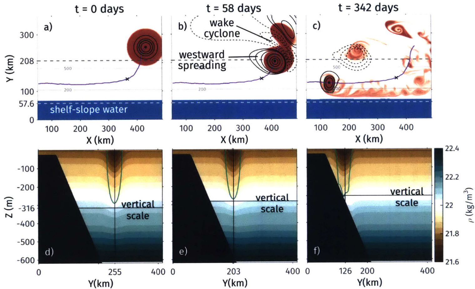
Figure 4.2: An eddy is prevented from reaching the shelfbreak. Panels (a-c) are snapshots of eddy dye (red) and shelf-slope water (blue). The blue water mass comprises water parcels that started inshore of a line 10 km offshore of the shelfbreak. SSH is contoured in black; negative contour values are dashed. The track of the eddy's center is in purple. Bathymetric contours are in gray, with dashed lines marking the shelf- and slope-break. Sponge regions are excluded. Panels (d-f) are y - z sections of density through the eddy's center. The green contour in all panels marks the core of the eddy (Section 3.2).
