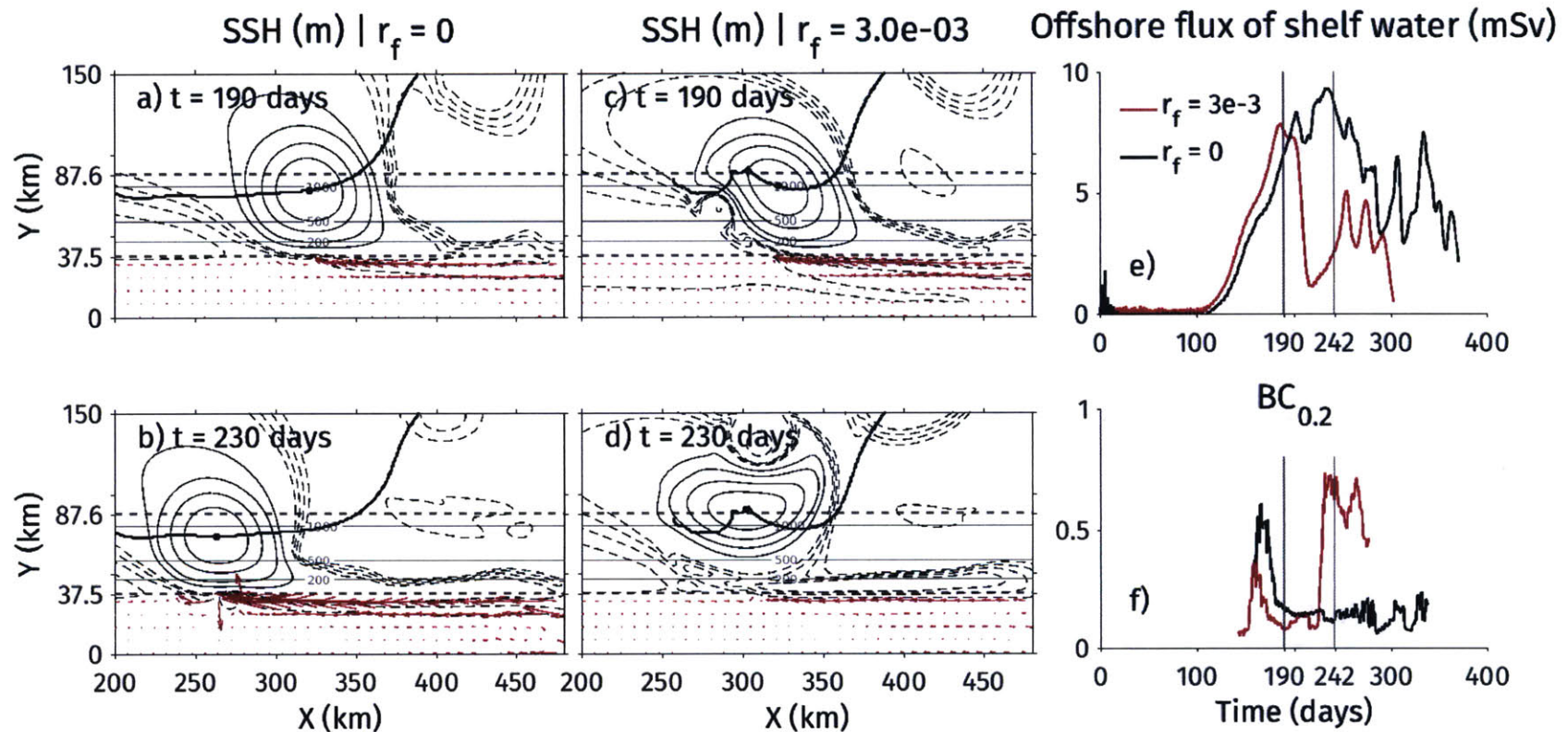
Figure 6.15: The influence of bottom friction. (a,b) and (c,d) are snapshots of SSH and surface velocity vectors for two simulations, one with no bottom friction, r_f = 0 and one with r_f = 3 \times 10^{-3} \text{ m s}^{-1} . Negative SSH contours are dashed. (e, f) Time series of offshore flux of shelf water at the shelfbreak and a parameter measuring the baroclinicity of flow on the shelf, BC defined in (6.2), for the two simulations. Non-zero bottom friction coefficient results in the spinup of a strong secondary cyclone that pulls the eddy away from the shelfbreak at t = 230 days, causing a sharp drop in the offshore flux at the shelfbreak. For the viscous simulation, BC initially drops to a value comparable to that for the inviscid simulation. However, there is a sharp increase in BC when the eddy moves away.
