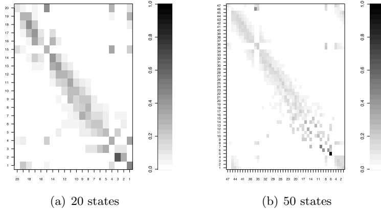
Figure 4: Markov transition matrices for wind uncertainty. (a)-(b) are obtained from a maximum likelihood fit to hourly time series
