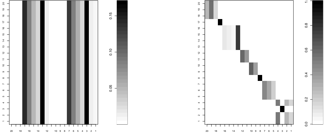
(a) Equilibrium density of ML Markov Chain, for any \epsilon > 0 .
