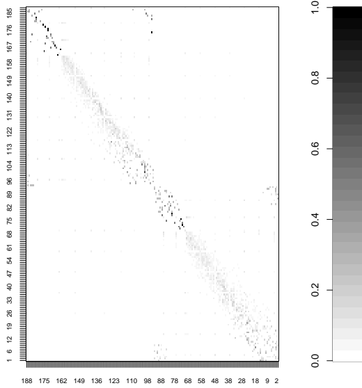
(a) A Markov chain with 200 states
