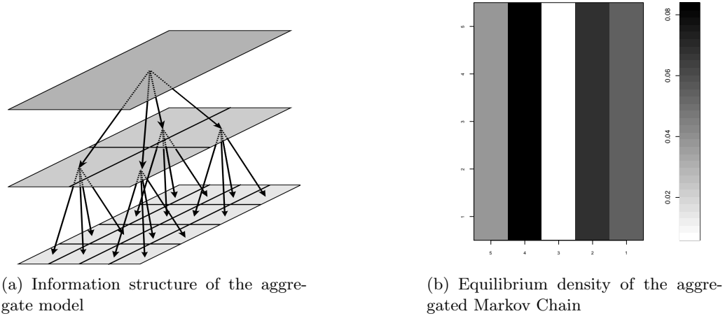
Figure 3: The aggregated model depicted in (b) gives the correct long term behavior (compare (b) with Figure 2(a)).
