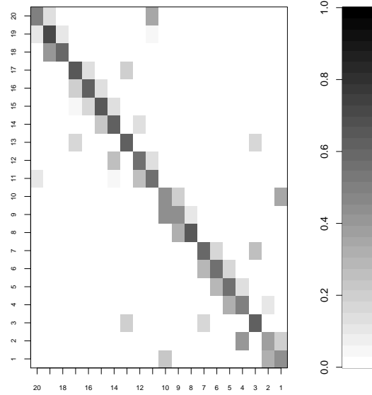
(b) A Markov chain with 20 states
