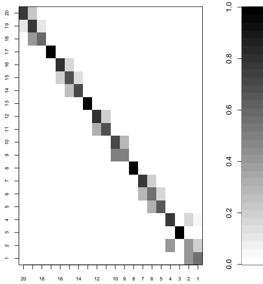
(c) Assumptions in existing models
