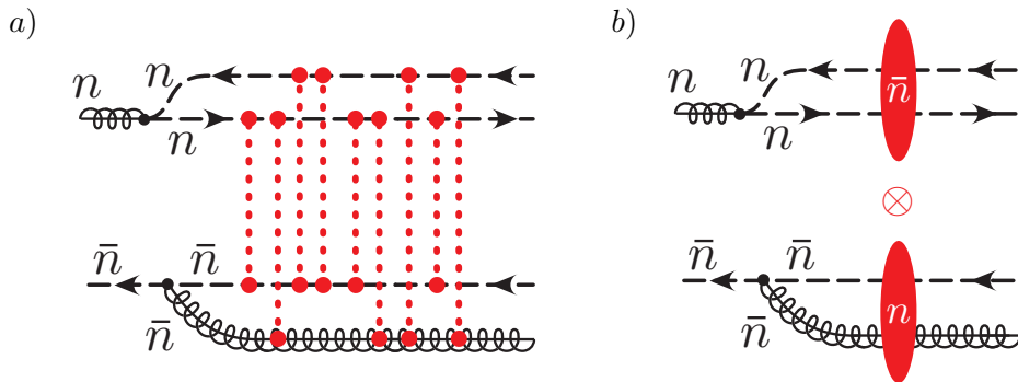
Figure 27. Correspondence between multiple Glauber exchange, with an example diagram shown in panel a), and the picture of Wilson lines used to represent partons crossing a shockwave, shown in panel b). The n -collinear particles see the other side via Glauber exchange only at an instant in time and longitudinal distance indicated by the location of the shockwave that is drawn as a large shaded red ellipse. In a mirror manner, the \bar{n} -collinear particles also see a shockwave representing the Glauber exchanges.
