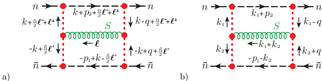
Figure 14. Two different momentum routings for the two loop diagram stemming from the time ordered product of two \mathcal{O}_{n\bar{n}}^{qq} insertions with one soft gluon. The soft momentum \ell^\mu = k_1^\mu + k_2^\mu can only be routed in a way which is consistent with the power counting. In a) the loops are soft and n - \bar{n} Glauber with \ell^\mu \sim (\lambda, \lambda, \lambda) and k^\mu \sim (\lambda^2, \lambda^2, \lambda) respectively, while in b) the loops are s - n Glauber and s - \bar{n} Glauber with k_1^\mu \sim (\lambda^2, \lambda, \lambda) and k_2^\mu \sim (\lambda, \lambda^2, \lambda) respectively.
