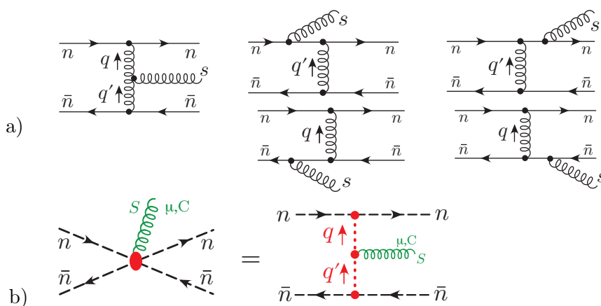
Figure 17. One Soft Gluon Matching for the Mid-Rapidity Operator in SCET appearing in quark-antiquark scattering. a) Full theory graphs. b) EFT Mid-Rapidity Operator graph with one soft gluon, shown by two equivalent diagrams which exploit a localized or factorized notation.
