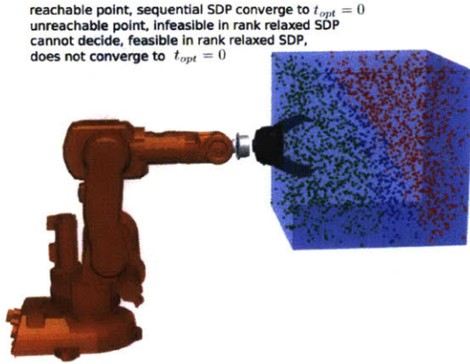
Figure 5-12: Robot arm reachability.
