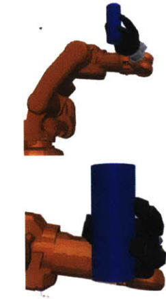
Figure 5-22: optimized force closure grasp from two views.
