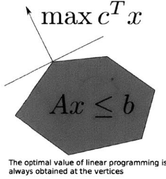
Figure 4-4: Linear programming
