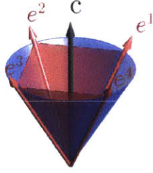
Figure 3-2: A nonlinear friction cone (blue) and the linearized friction cone (red). The unit length cone axis c is the direction of the normal contact force. e_1, \dots, e_4 are the four edges of the linearized friction cone.
