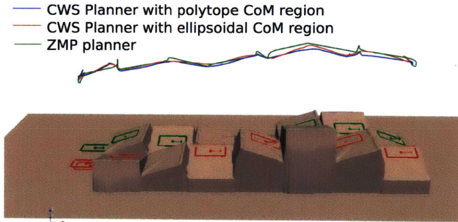
Figure 4-15: CoM trajectories on the terrain course
