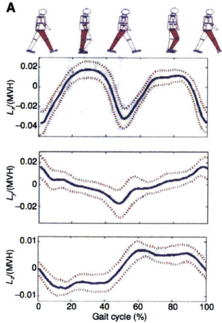
Figure 4-3: Normalized centroidal angular momentum for human walking experiments. The normalization factor is the product of the human mass ( M ), the walking velocity ( V ) and CoM height ( H ) [63]. The solid line is the mean value, the dashed lines are one standard deviation from the mean.
