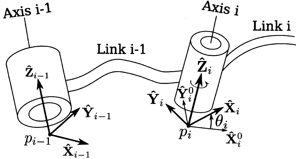
Figure 5-2: [24] A link frame \hat{\mathbf{X}}_{i-1}, \hat{\mathbf{Y}}_{i-1}, \hat{\mathbf{Z}}_{i-1} is attached to link i - 1 , link frame \hat{\mathbf{X}}_i, \hat{\mathbf{Y}}_i, \hat{\mathbf{Z}}_i is attached to link i . \hat{\mathbf{Z}}_{i-1}, \hat{\mathbf{Z}}_i are the revolute axes of the joints. The axis frame \hat{\mathbf{X}}_i^0, \hat{\mathbf{Y}}_i^0, \hat{\mathbf{Z}}_i^0 is attached to the joint i , and is fixed in the link frame i - 1 . The axis frame i and the link frame i share the frame origin and \hat{\mathbf{Z}}_i axis, the latter frame is obtained by rotating the former by angle \theta_i around the \hat{\mathbf{Z}}_i axis.
