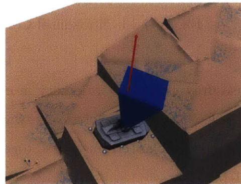
(b) CWS planner with ellipsoid CoM region
