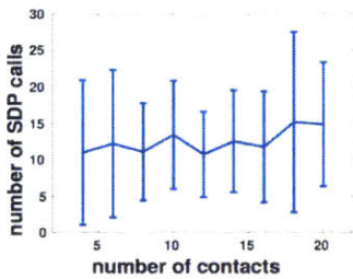
Figure 5-9: Scalability w.r.t number of contacts on a 30 facets polyhedron.
