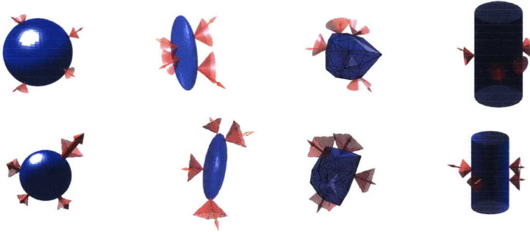
Figure 5-8: Force closure contacts on different geometries. The upper row uses non-linear friction cone, the lower row uses linearized friction cone. For the polyhedron (column 3), the contact facets are not specified by the user beforehand.
