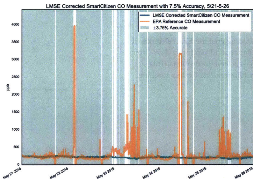
Figure 33: SmartCitizen CO with 7.5% Accuracy Threshold
