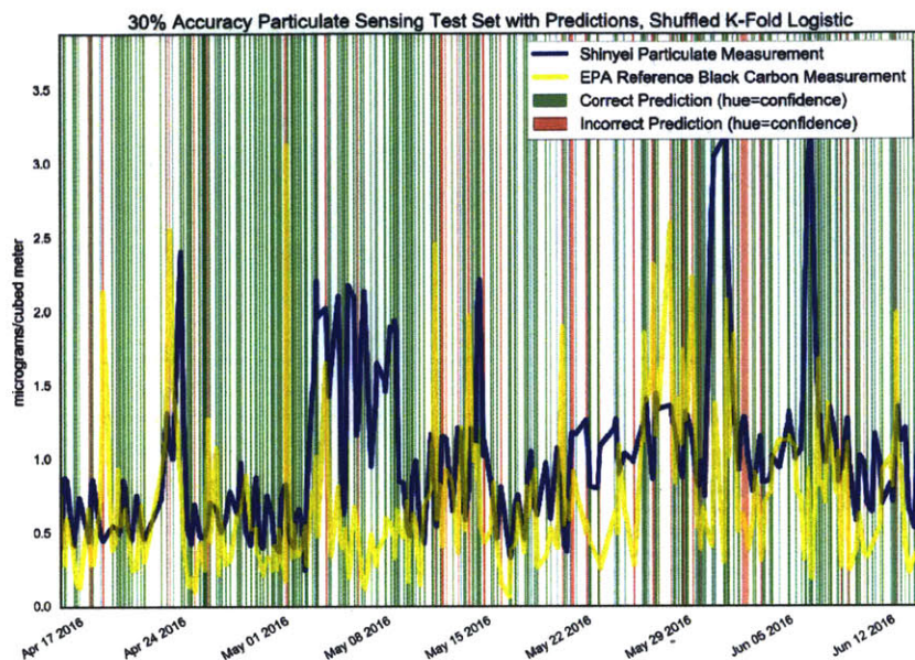
Figure 74: Sharp Particulate Prediction Accuracy
