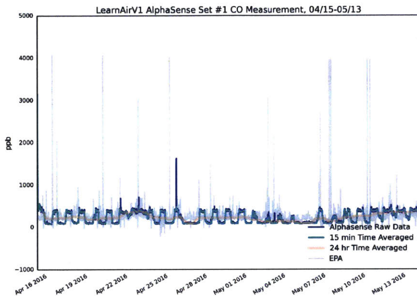
Figure 80: AlphaSense CO Sensor 1 Raw Data
