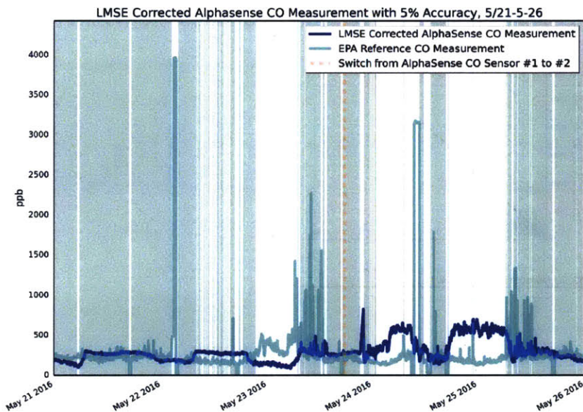
Figure 45: AlphaSense CO Sensor 1 and 2 with 5% Accuracy Threshold
