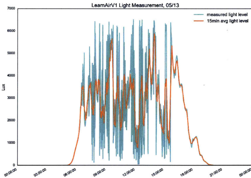
Figure 64: Lux during Test Period
