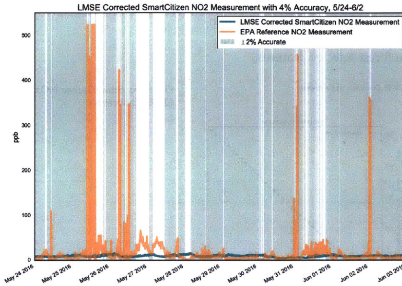
Figure 71: SmartCitizen NO 2 with 4% Accuracy Threshold
