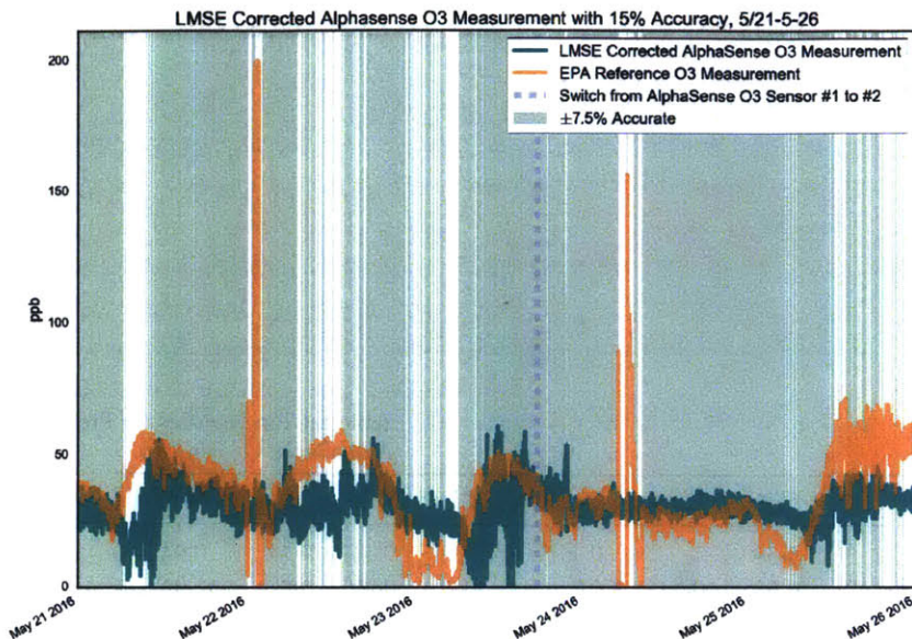
Figure 52: AlphaSense O 3 Sensor 1 and 2 with 15% Accuracy Threshold
