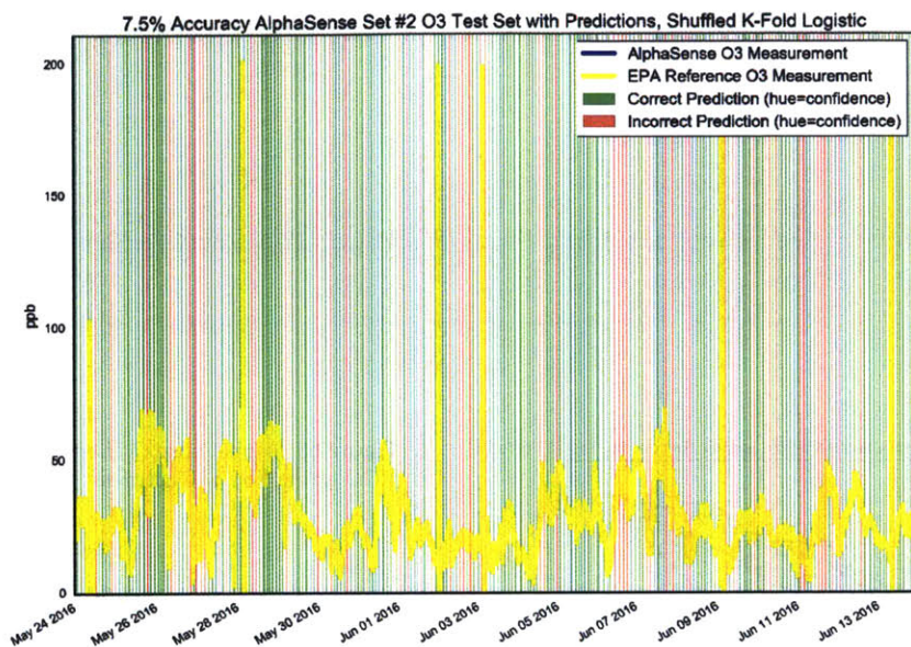
Figure 94: AlphaSense O 3 Sensor 2 Prediction Accuracy
