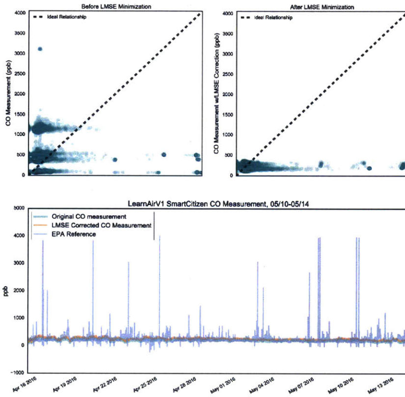
CO SmartCitizen Measurement LMSE Correction on Calibration
