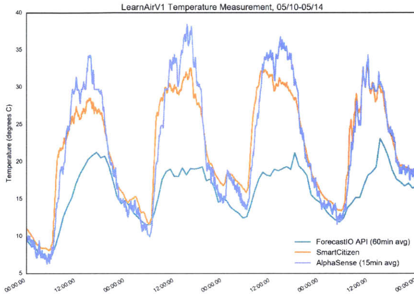
Figure 17: Temperature close-up
