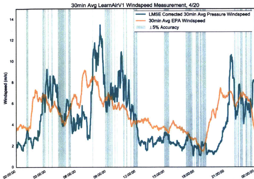
Figure 21: Wind Speed Measurement with 10% Accuracy, Zoomed
