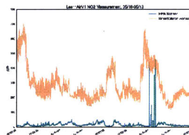
Figure 35: SmartCitizen NO 2 Raw Data
