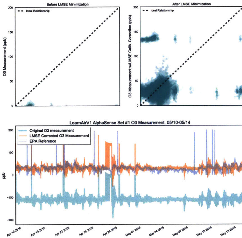
O3 AlphaSense Set #1 Measurement LMSE Correction on Calibration
