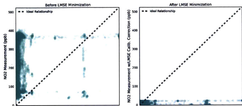
NO2 AlphaSense Measurement LMSE Correction on Calibration
