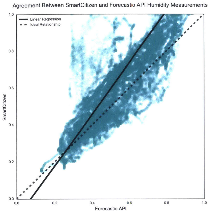
Figure 15: Humidity Comparison, SmartCitizen and ForecastIO
