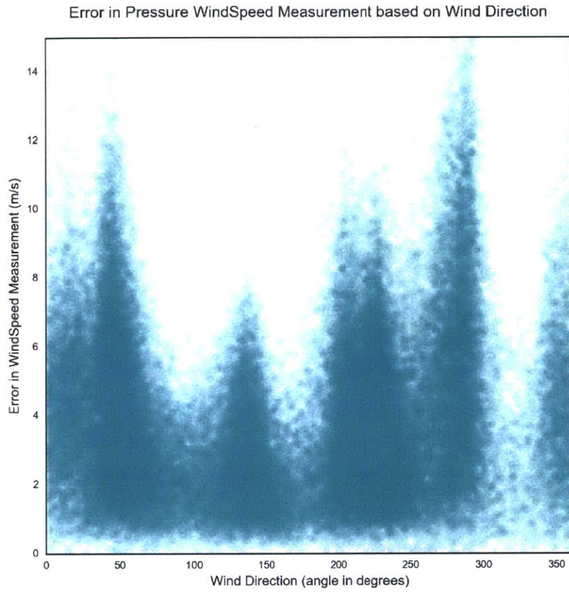
Figure 22: Discrepancy in Windspeed Measurement vs Wind Direction
