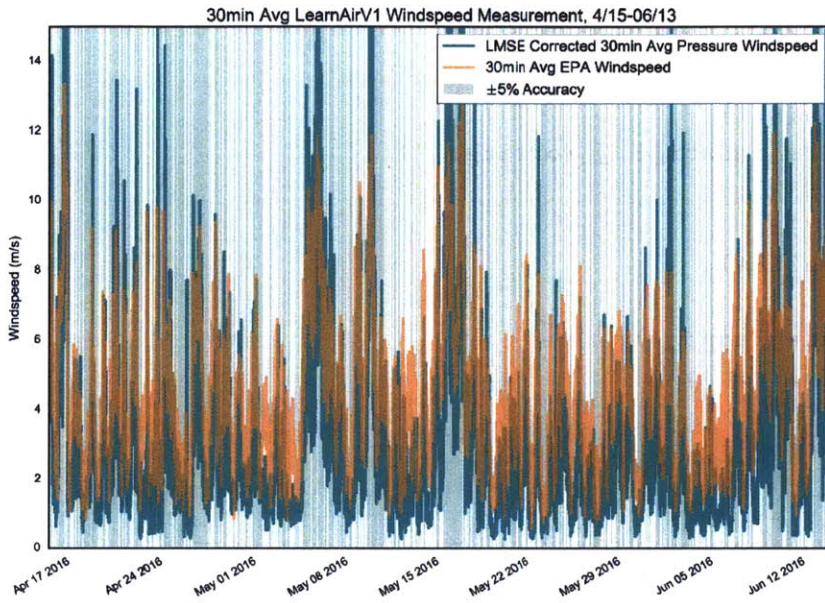
Figure 57: Wind Speed Measurement with 10% Accuracy
