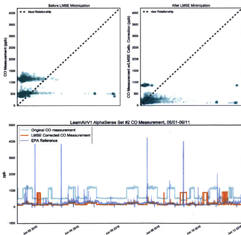
CO AlphaSense Set #2 Measurement LMSE Correction on Calibration
