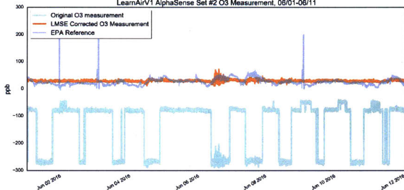
LearnAirV1 AlphaSense Set #2 O3 Measurement, 06/01-06/11
