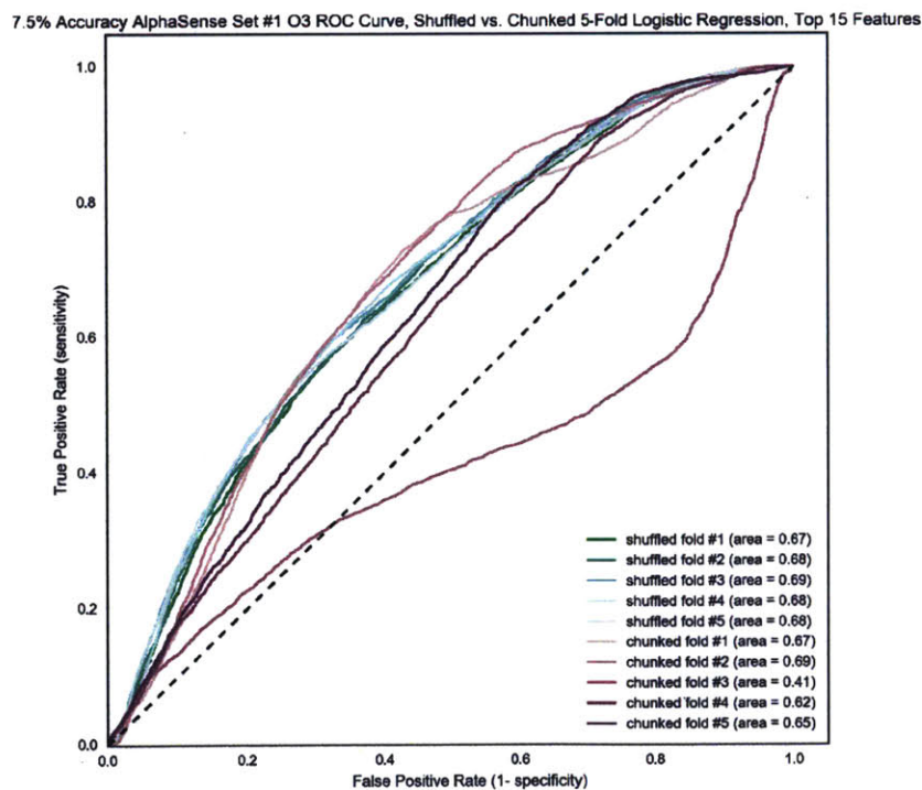
Figure 95: AlphaSense O 3 Sensor 1 ROC Using Top 15 Features
