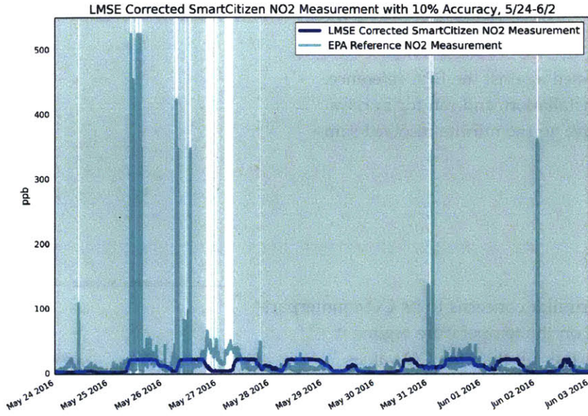
Figure 49: AlphaSense NO2 with 10% Accuracy Threshold
