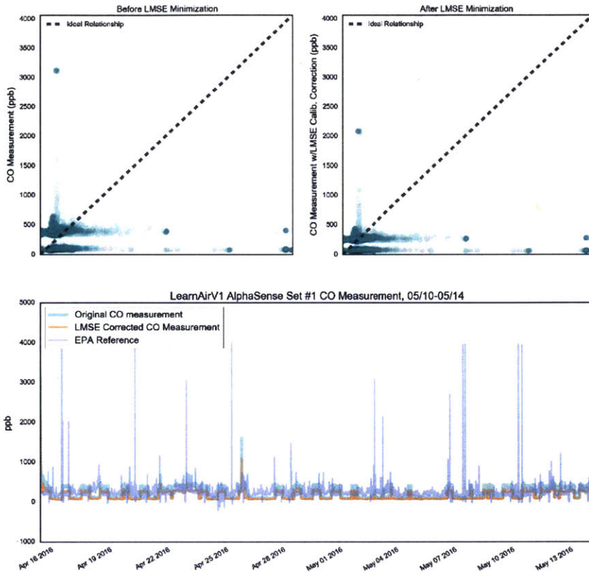
CO AlphaSense Set #1 Measurement LMSE Correction on Calibration
