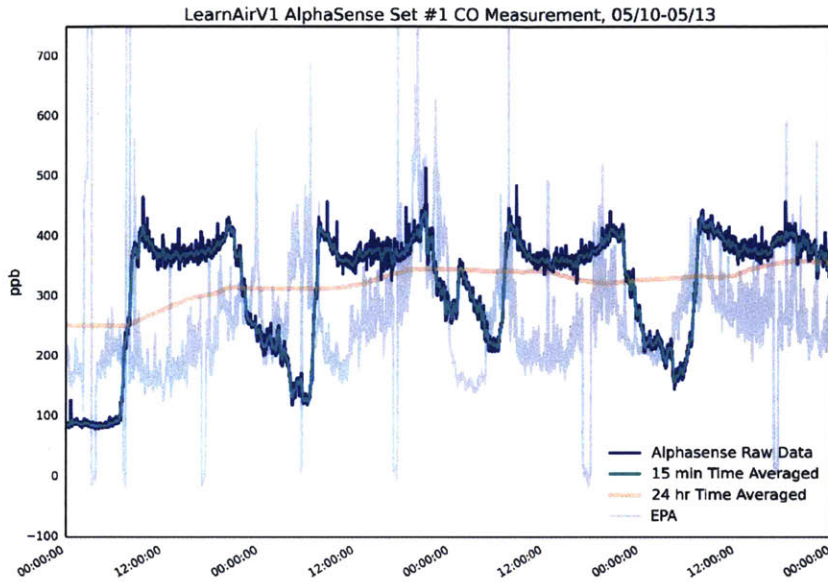
Figure 43: AlphaSense CO Sensor 1 Raw Data Zoomed
