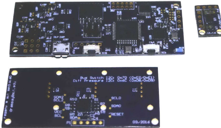
Figure 9: Main and daughter boards of learnAir V2.0
