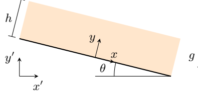
FIGURE 8. A schematic of the setup for the inclined plane problems. The global axes are x' and y' , while the axes x and y are parallel and perpendicular to the inclined plane respectively. The bottom of the inclined plane is a fully rough boundary.
