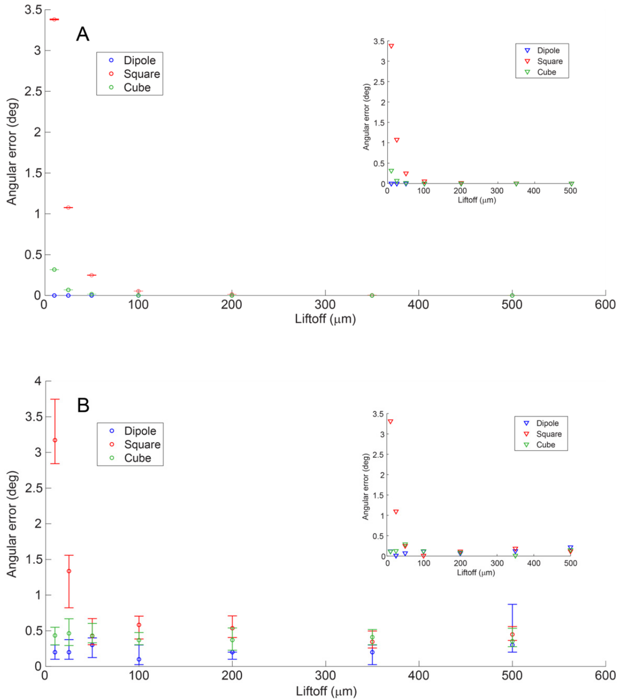
Figure 4: Error in the direction of the estimated net moments as a function of liftoff distance for all three test sources and different noise levels. Each colored circle represents the sample median of the angular error. The error bars denote the first and third sample quartiles. Colored triangles in the insets show the angular error of the mean net moment, which is typically smaller than the sample median. (A) Noiseless case (SNR = \infty ). (B) 10:1 proportion of signal and noise (SNR = 20 dB).
