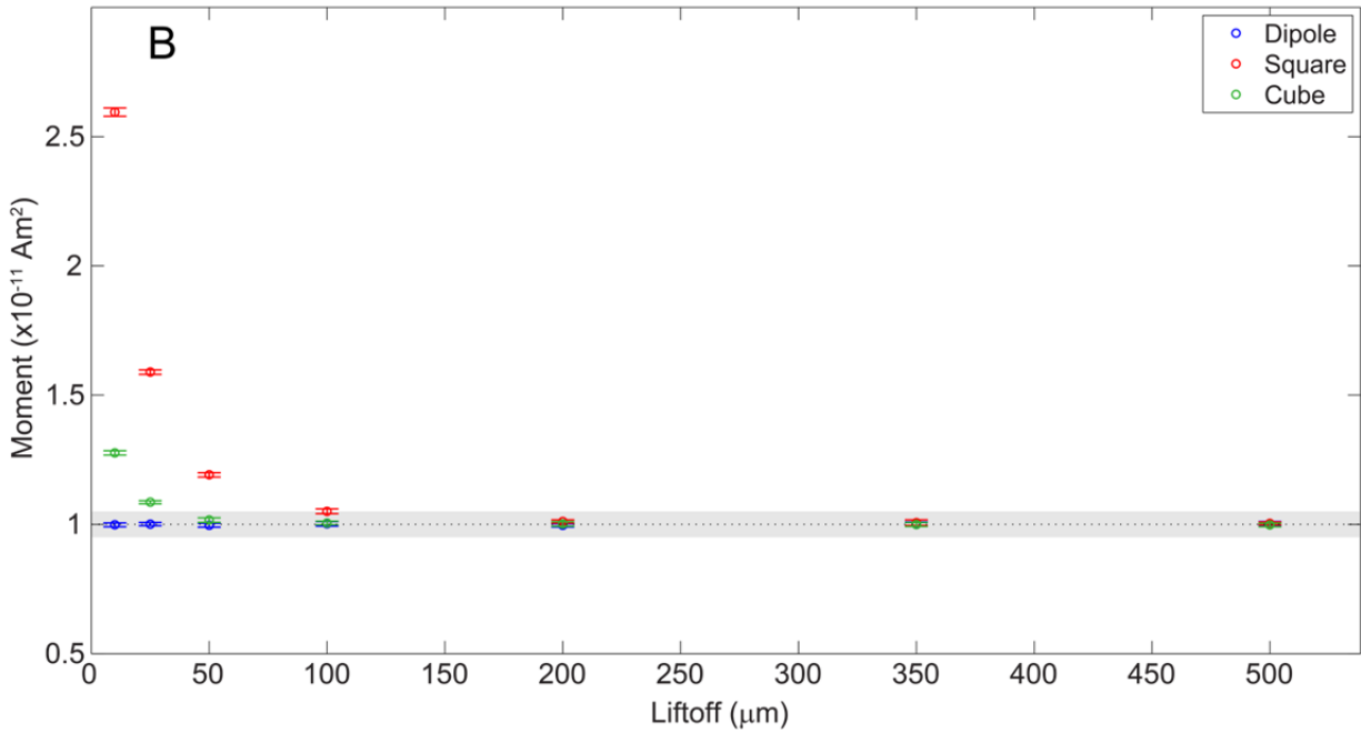
Figure 3: Magnitude of estimated net moments as a function of liftoff distance for all three test sources and different noise levels. Each colored circle represents the magnitude of the mean net moment (the mean of the magnitudes of estimated moments was omitted for clarity purposes, as it virtually coincides with the magnitude of the mean net moment). The error bars represent plus or minus one sample standard deviation. (A) Noiseless case ( \text{SNR} = \infty ). (B) 10:1 proportion of signal and noise ( \text{SNR} = 20 \text{ dB} ).
