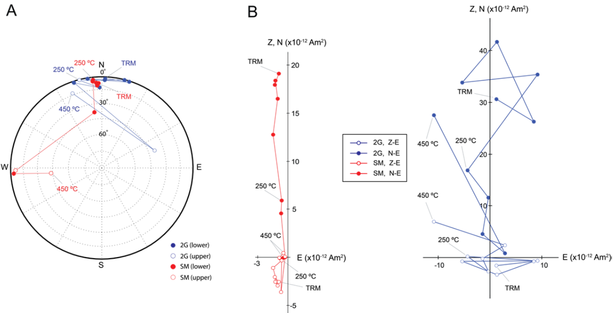
Figure 7: Thermal demagnetization of a small clump of cutting dust from the Millbillillie eucrite. We imparted a 50 \mu\text{T} TRM at 580 \text{ }^\circ\text{C} to the sample prior to carrying out a sequence of thermal demagnetization steps. At each step, the sample was measured on the 2G rock magnetometer and on our SQUID microscope magnetometer. (A) Net moment directional data shown on an equal area stereoplot (SQUID microscope data shown in red, 2G data shown in blue). (B) Up-east and north-east projections of the endpoints of the net moment vector shown (SQUID microscope data shown in red, 2G data shown in blue). (Magnetic field was mapped \sim 200 \mu\text{m} above the sample.)
