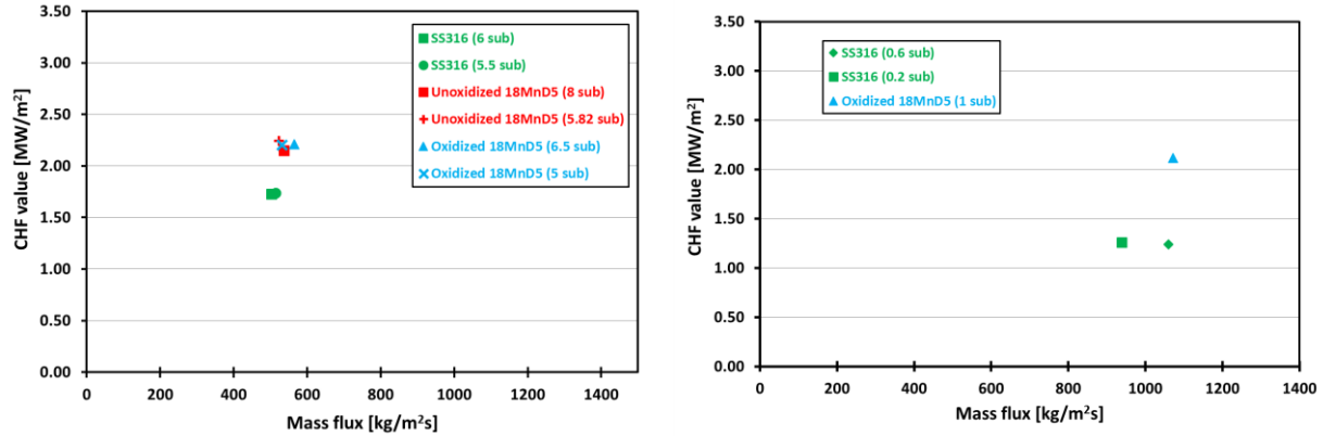
Figure 12. CHF data for test condition I (90°, 500 kg/m²s, 7°C sub) (left), and test condition II (45°, 1000 kg/m²s, sat) (right).
