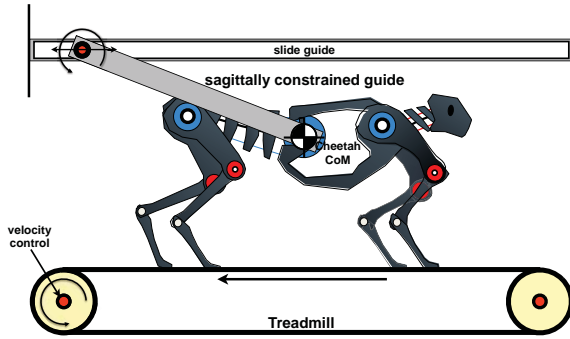
Fig. 13: Experimental setup of MIT Cheetah on treadmill. Motion is constrained to the sagittal plane.
