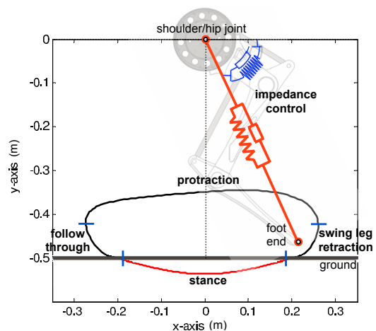
Fig. 11: Desired swing phase (black solid line) and stance phase (red solid line) trajectory for the front leg, as well as the desired ground position (straight black solid line at -0.5 m). The point (0, 0) is the location of shoulder/hip of the robot.
