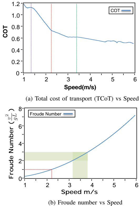
Fig. 16: The plot shows TCoT and Froude number with respect to running speed from 1 m/s to 6 m/s. (a) The red line indicates the start of running (2.3 m/s). The green line shows when the swing leg retraction speed reaches 3.4 m/s. (b) The red line represents a Froude number of 1.0, where animals switch from walk to run. For the MIT Cheetah robot, the Froude number of 1 corresponds to 2.3 m/s, the speed at which the robot switches from walk to run. The green area is the region of Froude numbers between 2.0 and 3.0 where quadrupeds change the gait from trot to gallop
