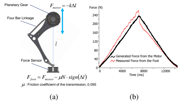
Fig. 8: (a) The experimental setup used for determining loss in the mechanical transmission. The force at the foot is calculated using the torques applied by the motors and compared against a force sensor under the foot. (b) Experimental data showing the difference between the expected force on the foot as generated from the motors, and the actual force measured.
