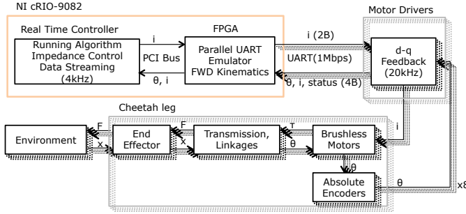
Fig. 12: Control System Diagram for the MIT Cheetah Robot. The main controller (NI cRIO-9082) has the Real-Time multicore controller and the FPGA and controls 8 BLDC motor drivers in parallel.
