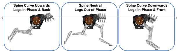
Fig. 10: Differential Spine Actuation. During high speed running, the spine can be actuated by choosing to actuate the rear legs either in-phase or out-of-phase. When the legs are in-phase and backward, the differential coupling would cause the spine to arch upwards, increasing the stride length of the MIT Cheetah. When the legs are in-phase and forward, the differential would make the spine curve downwards, tucking the rear legs further forward. Otherwise, when the legs are out-of-phase, the spine remains neutral.
