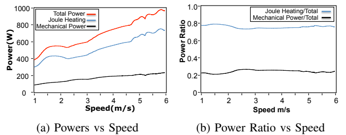
Fig. 18: The plot shows Joule heating and mechanical power, and the ratios between them with respect to running speed from 1m/s to 6m/s. (a) The red line represents the total power consumption from the battery, which is the sum of Joule heating and mechanical power. The blue line is the power used in Joule heating. The black line is the mechanical power. (b) The blue line is the ratio of Joule heating to the total power, and the black line is the ratio of mechanical power to the total power. The ratios are not changed significantly with respect to speeds.
