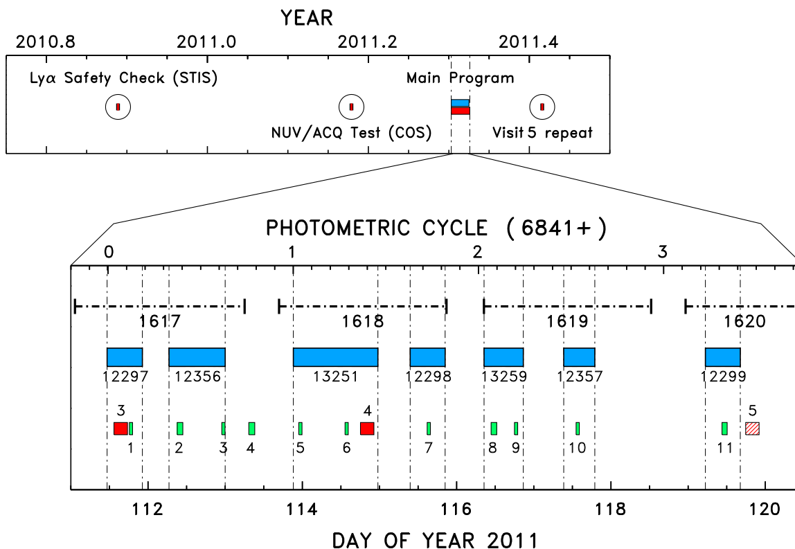
Figure 2. Overview of the FK Com COCOA-PUFS project. The upper panel sketches major elements of the campaign. The lower panel focuses on the intensive main program in 2011 April: the Chandra pointings (blue—ObsIDs annotated), the three “long program” 3-orbit HST Visits of GO-12376 (red rectangles—Visit numbers annotated), and the interspersed eleven 1-orbit “short program” HST Visits of GO-12279 (green—Visit numbers annotated). The red hatched GO-12376 Visit 5 failed (owing to a Guide Star acquisition issue), and was repeated two months later in 2011 June. Dotted-dashed bars in the upper part of the panel depict orbital visibility periods for Chandra ; gaps represent perigee passes when Chandra could not observe.
