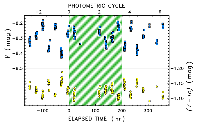
Figure 29. Optical photometry of FK Com before, during, and after the (green shaded) main campaign period. Upper part of the figure depicts the V magnitudes (blue squares; note reversed y-axis scale: brighter visual luminosities toward top of diagram), while the lower part illustrates the (V - Ic) color (yellow circles; higher values indicate redder colors). The apparent (nightly) changes are real and highlight the large and rapid photometric variability of the fast-rotating, heavily spotted G giant.
