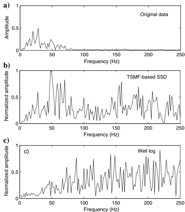
Figure 12. The amplitude spectra of the 270th trace of the field data in Figure 9 (a) before and (b) after the application of the TSMF-based SSD, and (c) the normalized amplitude spectrum of the reflectivity derived from well logs near the location of the 270th trace.
